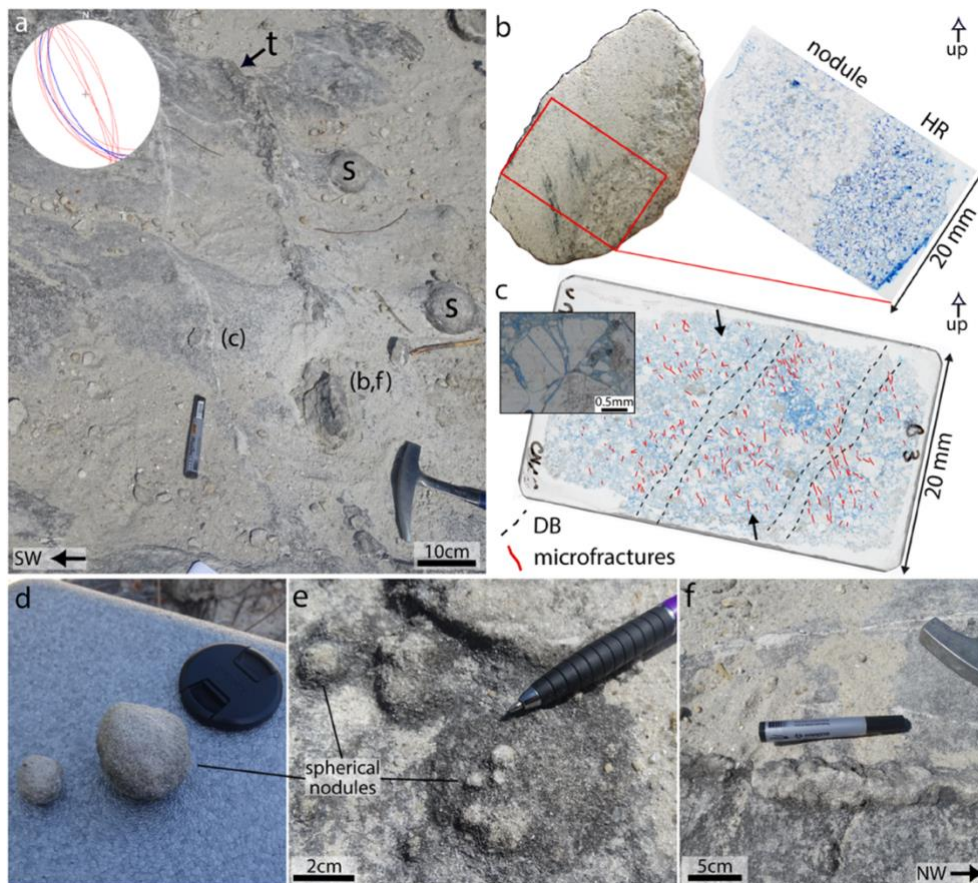
305 Figure 8. Typical relationships between nodules and DBs. (a) Continuous tabular nodule (t) and isolated spherical nodules (S) aligned parallel to the NW-SE normal-sense bands dipping SW ( \sim 55^\circ ; red lines in the inset stereoplot). The tabular bodies dip to the SW parallel to the bands (blue lines in the stereoplot in the inset). The position of (a) is indicated in Fig. 6b. (b) Hand specimen and polished thin sections impregnated with blue-dyed resin of a tabular nodule in (a). (c) Polished thin sections impregnated with blue-dyed showing two sub-parallel NW-SE normal-sense bands dipping SW. Mapping of microfractures developed at grain contacts consistent with Hertzian 310 contacts (e.g. Eichhubl et al., 2010; Soliva et al., 2013) endorses the normal kinematic of these bands (see Supplement S1 for details). “Up” refers to the topography. Close-up on spherical (d-e) and tabular (f) nodules from the field. Pen-marker length in (a, f) is about 13.5 cm. Lens-cover in (d) has a 5.5 cm diameter.
