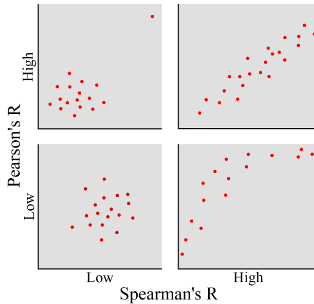
180 Figure 3 Comparison of the Spearman's rank correlation coefficient with respect to the parametric Pearson's correlation coefficient. Non-parametric Spearman's correlation is more robust in case of outliers, and is also able to detect non-linear correlation, in addition to standard linear correlation (Swan and Sandilands, 1995).
