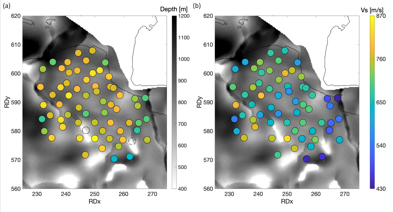
Figure 6. Average shear-wave velocities for the North Sea Group from each station in the Groningen network. Coordinates are plotted in Rijksdriehoek (RD) projection. (a) Map of the depth of base North Sea Group (Van Dalfsen et al., 2006) with, in circles, the average shear wave velocities for the entire North Sea Group ( V_s^{NSG} ). The solid circle represents the discarded station G45 and the dashed circle the discarded station G52. (b) Average shear-wave velocities calculated according to Eq. 5 for the lower part of the NSG ( V_s^{NSL} ): from 200 m depth till the base of the sedimentary cover.
