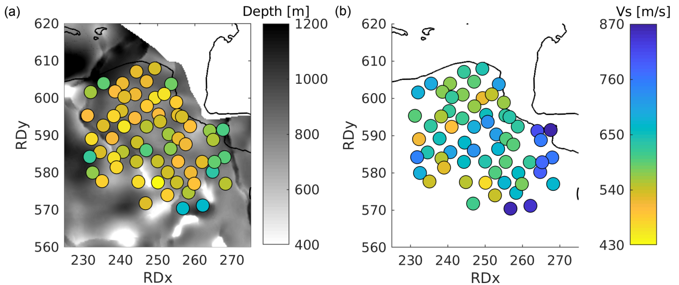
Figure 6. Average shear-wave velocities for the North Sea Group from each station in the Groningen network. Coordinates are plotted in Rijkdriehoek (RD) projection. (a) Map of the depth of base North Sea Group (Van Dalfsen et al., 2006) with, in circles, the average shear wave velocities for the entire North Sea Group ( V_s^{NSG} ). (b) Average shear-wave velocities calculated according to Eq. 5 for the lower part of the NSG ( V_s^{NSL} ): from 200m depth till the base of the sedimentary cover.
