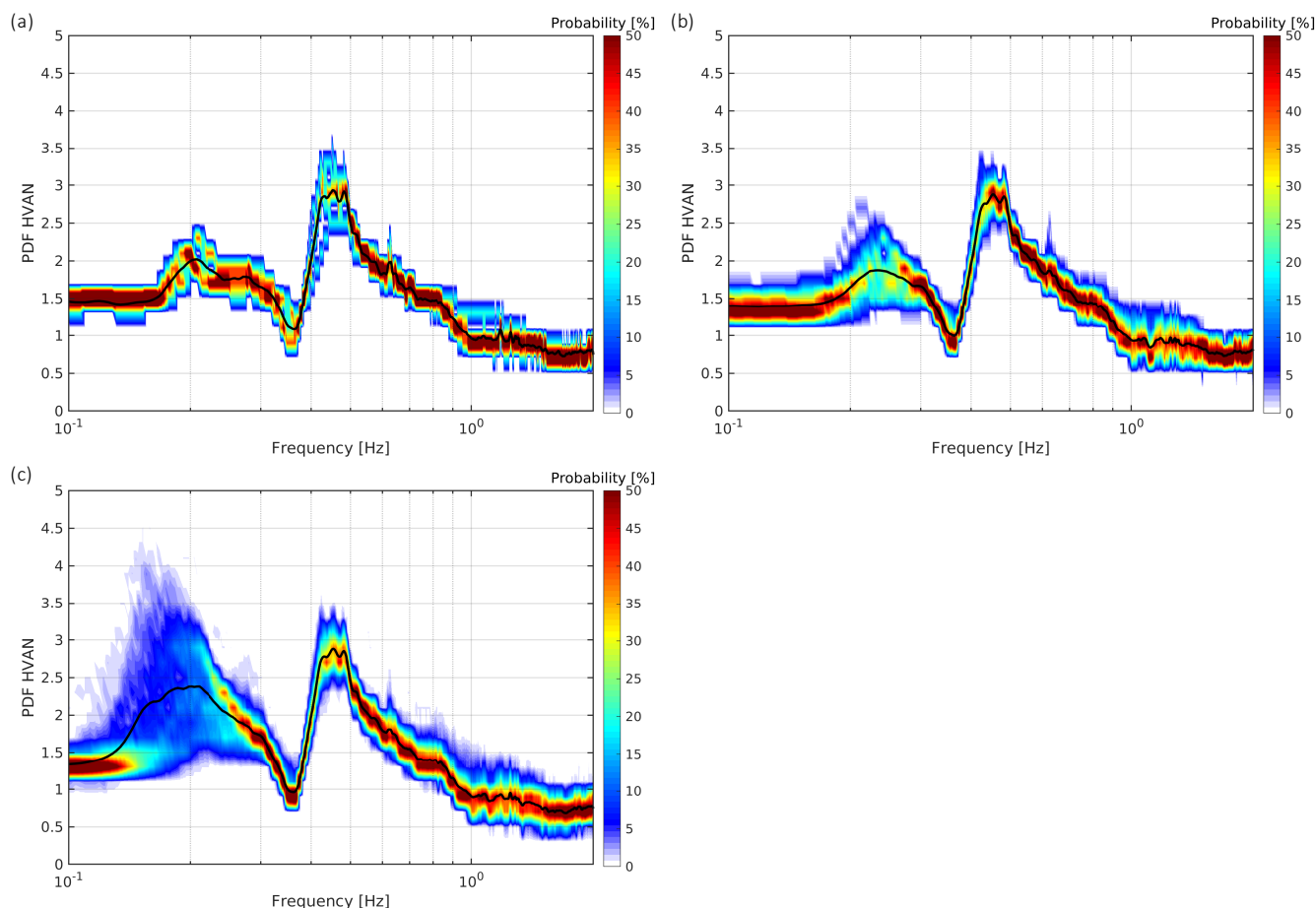
Figure 10. Probability density functions (PDF) from ambient noise horizontal- to-vertical spectral ratios (HVAN) for station G39, 50m level. The black line represents the mean. (a) PDF HVAN for one week (21/03/2017-28/03/2017). (b) PDF HVAN for one month (01/05/2017-01/06/2017). (c) PDF HVAN for one year (01/02/2017-01/02/2018).
