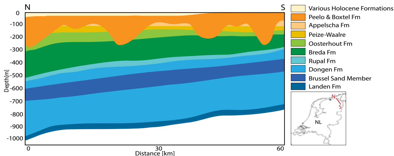
Figure 1. Schematic cross section of the North Sea Group (NSG) based on formation depths from www.dinoloket.nl and stratigraphic charts (Wong et al., 2007). The formations of the Lower NSG have blue colours, formations of the Middle NSG are in Green and Quaternary formations of the Upper NSG are in orange/yellow. From the different Members in the lower NSG, only the Brussel Sand is included due to its importance for this study.
