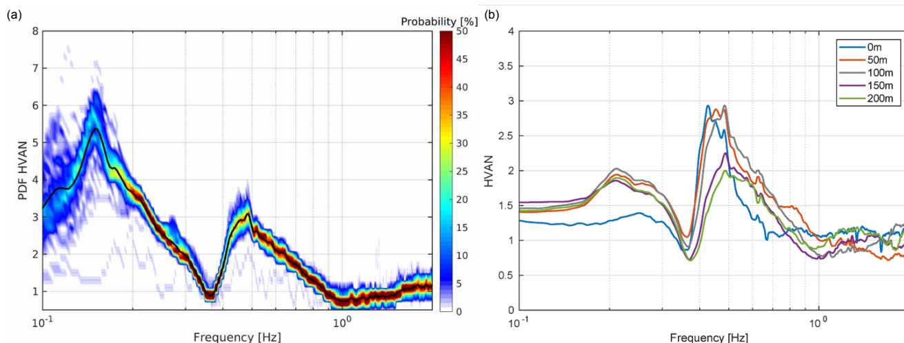
Figure 11. (a) PDF HVAN for one month (01/09/2018-01/10/2018) at broadband station G82B, located within 100 m of G39, and has a depth of 100m. The broadband PDF HVAN displays a peak for the fundamental mode (around 0.15Hz) and the secondary peak (around 0.45Hz) reflects the higher mode for Rayleigh waves. The black line indicates the mean from the PDF HVAN. (b) HVAN curves for one month for station G39 for all depth levels.
