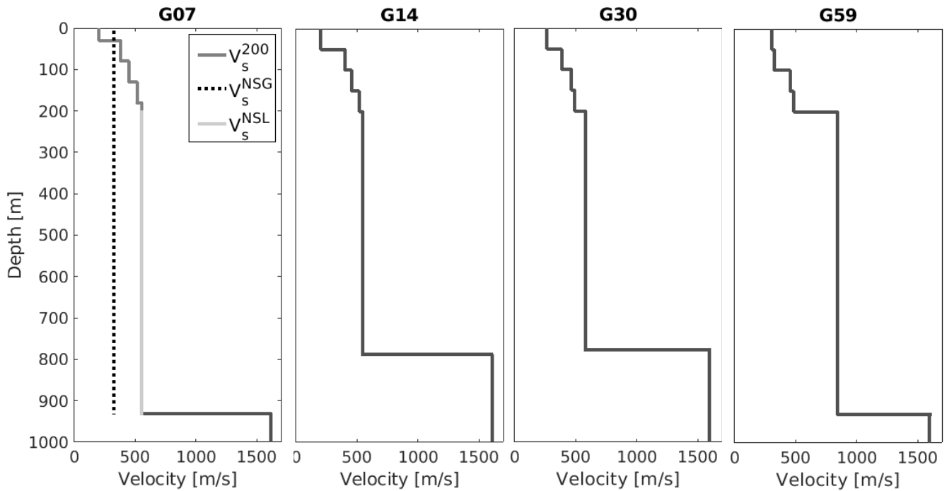
Figure 7. Subsurface velocity profiles from resp. station G07, G14, G30 and G59. The panel on the left shows the construction of a merged S wave profile: velocity profiles of the upper 200m ( V_s^{200} , dark grey line) are taken from Hofman et al. (2017), the entire NSG average velocity ( V_s^{NSG} , dotted line) from teleseismic phases. The V_s^{NSL} (light grey line) is calculated from the V_s^{200} and V_s^{NSG} (Eq. 5). The velocity contrast at around 800m depth is between the base NSG and top Chalk Group.
