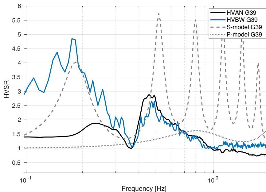
Figure 12. Modeled shear wave resonance (dashed line), pressure wave resonance (dotted line), HVAN (black solid line) and the HVBW (blue solid line) for the 50 meter depth seismometer of station G39. The HVBW is taken as the mean over 5 teleseismic phases (Table 1)
