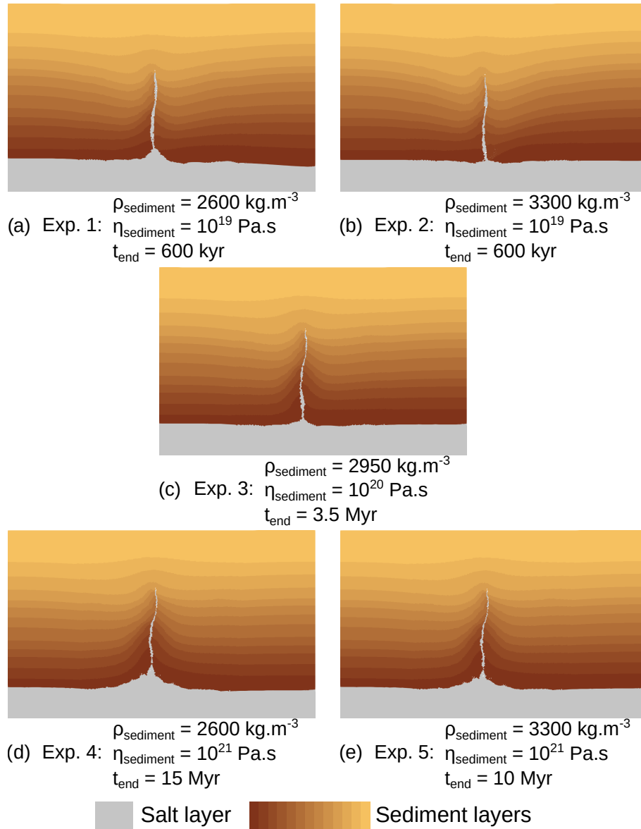
Figure 10. Results of the 5 restoration experiments done on the salt model setup of Fig. 8, after different time spans t_{\text{end}} .
