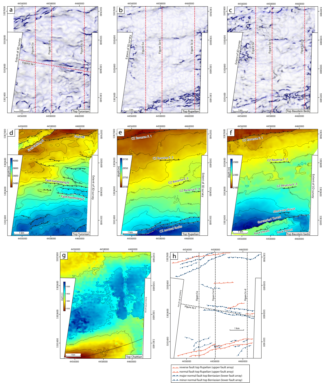
Figure 6. Co-rendered variance and most negative curvature multiattribute maps and depth-structure maps showing: (a), (d) lower fault array at top Turonian, (b), (e) upper fault array at Top Rupelian, and (c), (f) at top Baustein beds. (g) Depth-structure map of top Chattian showing termination of the Geretsried fold to ENE. Dashed line represents the fold hinge. (h) Map of fault traces interpreted within the 3D seismic volume.
