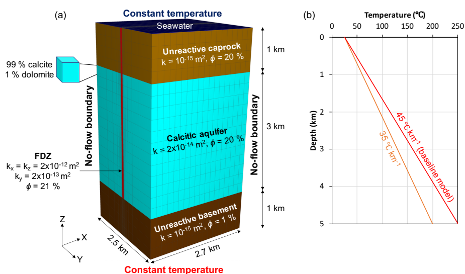
Fig. 1. Model dimensions, material properties, and simulation grid.
