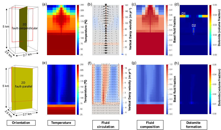
Fig. 2. 2D simulation results.
