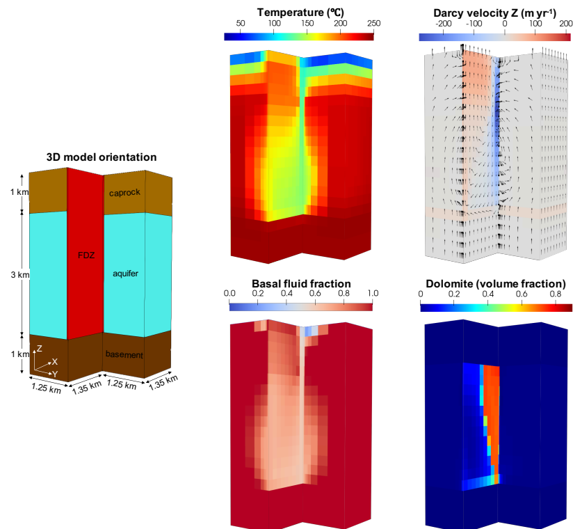
Fig. 3. 3D baseline simulation.
