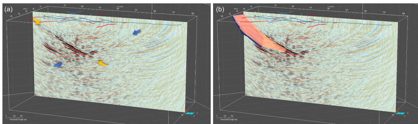
280 Figure 7: Depth slice through the FVM result using the 1D migration velocity model including information from MVA (Table 1): (a) without and (b) with the known mineralization in red and blue. The arrows in (a) mark the image of the main mineralization reflector and a crosscutting reflector dipping in the opposite direction (compare Figure 5 and 6). The shown slice is at the same location as the slice shown in Figure 5 and 6.
