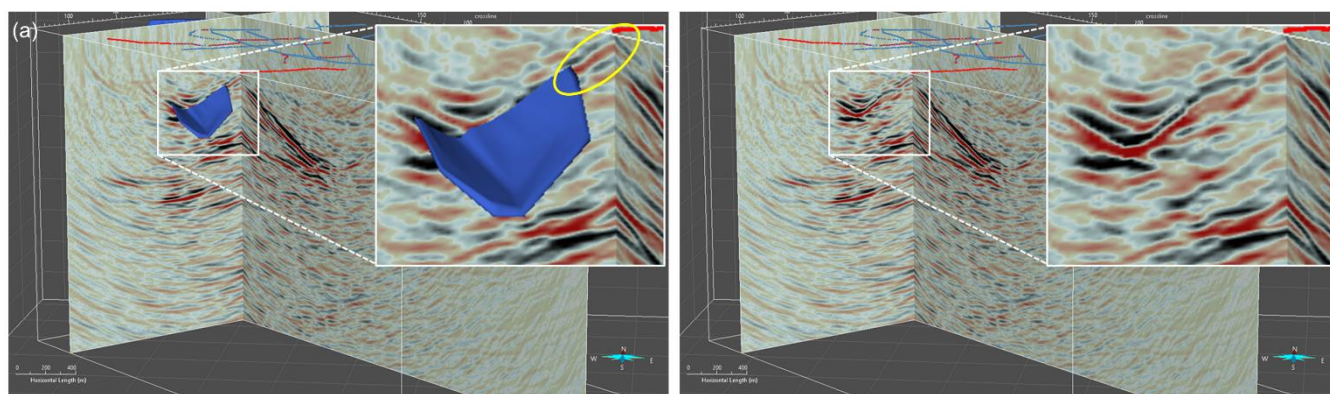
Figure 9: Perspective view with (a) and without (b) the model of the known mineralization (blue body). The zoomed inset shows a good agreement of the position, depth and shape of the known mineralization and the corresponding reflectors in the seismic image.
