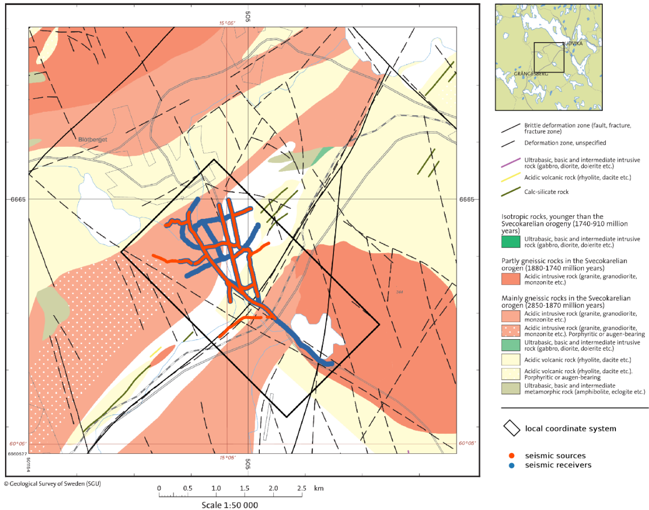
115 Figure 1: Survey layout with source (red) and receiver (blue) positions of the 3D survey and the local coordinate system used for first arrival traveltimes tomography and imaging (black box) on top of the bedrock map. Courtesy of the Geological Survey of Sweden.
