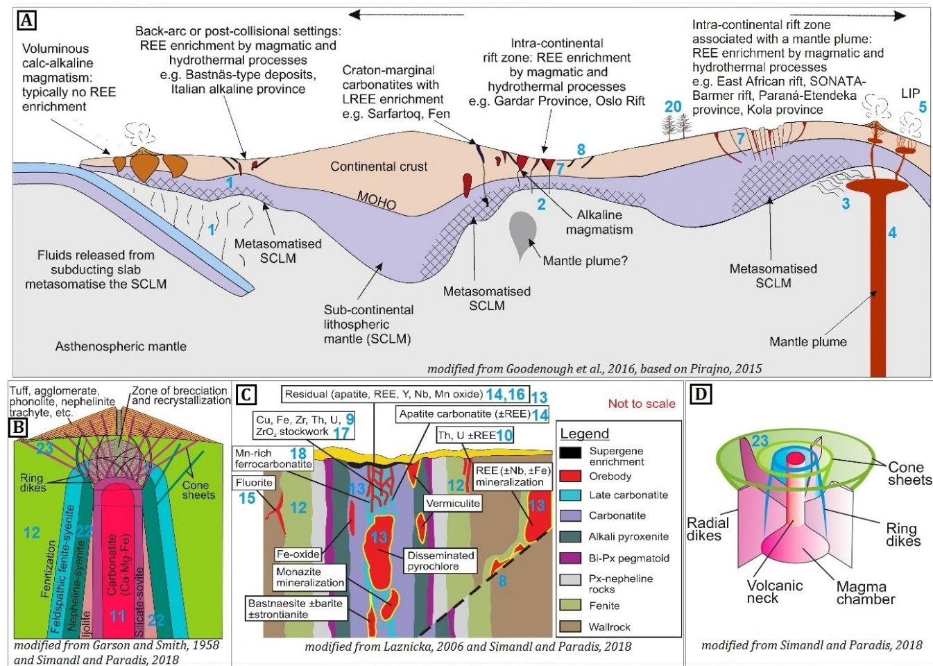
Figure 3. Idealised genetic model of a carbonatite-alkaline-complex-related REE mineral system (adapted from Aranha et al., under review) cross-referenced to processes listed in Table 2 through the numbers in blue. (A) Depicts the fertility and geodynamic setting along with the transport architecture on a regional scale. B, C and D focus on the emplacement architecture at the camp-to-prospect-scale. (B) Shows the idealised geometry of the intrusion and the relation of carbonatites and associated alkaline rocks and fenitisation (C) Presents the near-surface structural architecture and the spatial distribution of associated. (D) Displays the idealised geometry of a carbonatite-alkaline intrusion and the relationship between the magma chamber, ring dykes, cone sheets, and radial dykes.
