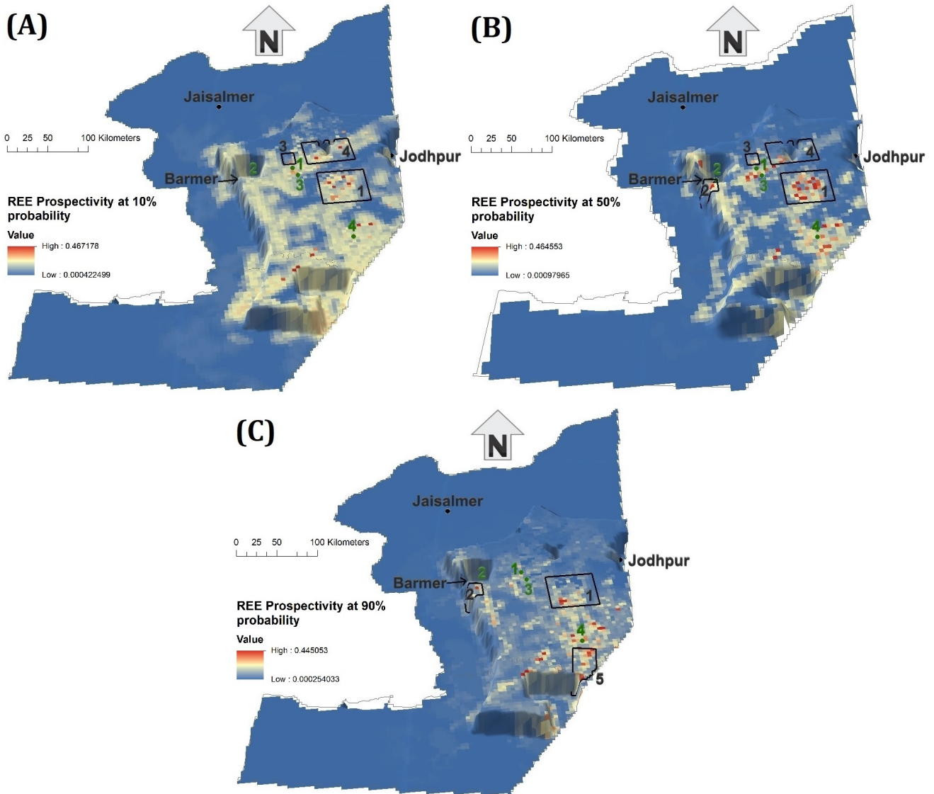
Figure 5. Continuous scale prospectivity maps at 10%, 50% and 90% probability levels draped over the confidence layer, shown in (A), (B) and (C), respectively. The colours mark increasing prospectivity from low (blue) to high (red). The elevations mark high confidence in the data used for prospectivity modelling. Black balls indicate major cities, and green balls indicate known carbonatite occurrences; green numbers correspond to the known carbonatite occurrences: 1 – Sarnu Dandeli, 2 – Danta-Langera-Mahabar, 3 – Kamthai, 4- Mundwara. Areas marked with black numbered rectangles are discussed in Section 7.
