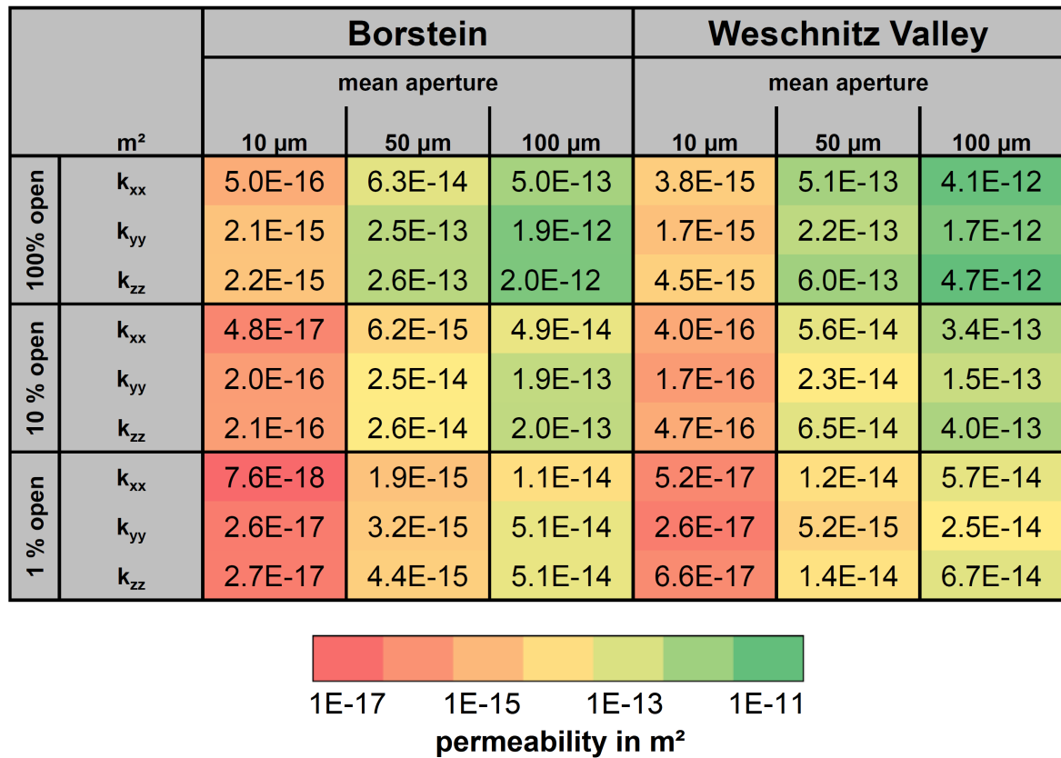
Figure 8. Summary of the DFN modelling. The Oda permeabilities in x-, y- and -direction were calculated as a function of fracture density, orientation, aperture and proportion of open fractures.
