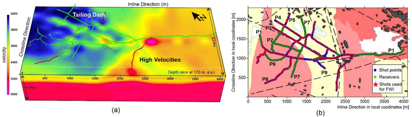
210 Figure 2: (a) Starting velocity model for FWI built using FAT. The depth slice is shown at 170 m above sea level. The velocity model is highly heterogeneous at the shallow level; however, it is relatively homogenous at the bedrock level (few tens of meters below the surface). (b) Shots, receivers, and spatial extent used during velocity model building in FAT/FWI in the local coordinate system (blue rectangular box in Fig. 1). Green dots mark the receivers, overlapping blue dots show all the shots (>1000) and red stars show a subset of 216 shots used for FWI.
