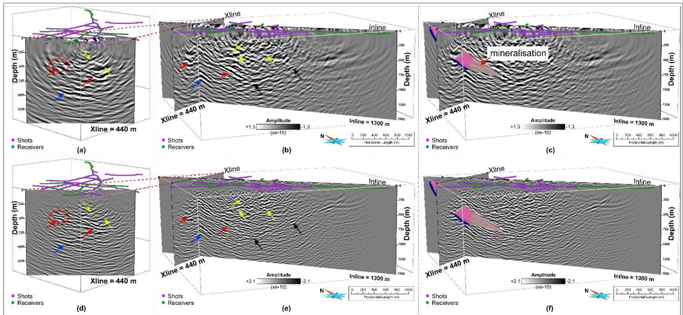
Figure 13: (a) and (b) shows a crossline and cross-sectional view of depth image produced from RTM using the FAT velocity model. (c) is same as (b) with the projection of know mineralisation. (d), (e) and (f) is same as (a), (b) and (c) but for FWI velocity model. Different arrows show different events observed in the depth images. Blue and pink surfaces are the known mineralisation surfaces produced mainly based on drilling in the area. The depth image derived from the FWI velocity model is less noisy, more focussed and with higher accuracy as compared to the FAT velocity model.
