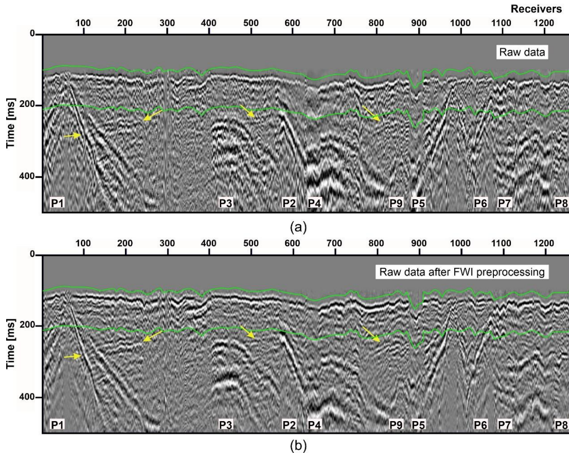
Figure 3: A comparison of an exemplary (a) raw show gather, and (b) data after preprocessing (observed data) is shown after applying linear moveout (LMO) with a constant velocity of 5500 m/s and bulk shift of 100 ms. Yellow arrows mark the reflection from the mineralisation, and green lines show the data range used during FWI inversion. The location of different receiver lines marked with P's can be followed in Figure 2b. Note that after the preprocessing, first arrivals are more prominent with higher SNR and better coherency.
