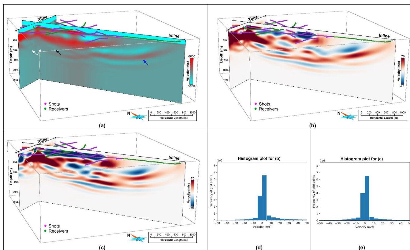
325 Figure 6: (a) Velocity model produced from random selection of shots (subset-2), compare with Figure 5b, (b) velocity perturbation model produced using velocity model derived from subset-1 and from manual selection of shots, i.e. velocity model shown in Figure 5b, (c) same as (b) but for subset-2, (d) and (e) histogram plot for (b) and (c). The plot shows the efficacy of the inversion strategy which effectively produces a similar velocity model independent of shot selection within acceptable limits of velocity perturbation.
