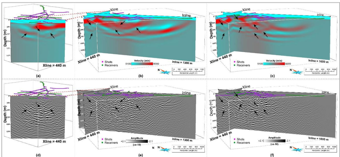
Figure 14: (a) shows crossline, (b) and (c) and cross-sectional view of FWI velocity model for two different inline position. (d), (e) and (f) is same as (a), (b) and (c) but for RTM depth image. Black arrows shows noticeable events present for both the results.
