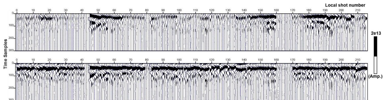
380 Figure 8: Source wavelet estimation for each shot location used in FWI for (a) starting model from FAT, and (b) FWI velocity model. Note that a better amplitude response and coherency is obtained from the FWI velocity model.
