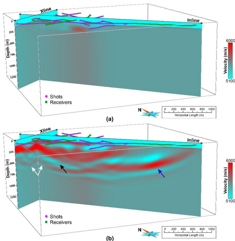
300 Figure 5: Comparison of velocity model resulted from (a) FAT, and (b) FWI using a dataset comprising a manual selection of 216 shots. Note that the velocity details with depth for the FAT velocity model is restricted in the near-surface region while FWI derived velocity model has much greater details at depth. White arrows indicate a dipping high-velocity layer in the SE direction which appears to follow a curved geometry in the SW direction, black arrow shows the possible presence of a cross-cutting fault and blue arrow shows artefact introduced in the velocity model due to only one-way energy propagation as there are only receivers in the SE part of the survey. Several other features in terms of high and low velocities can also be inferred in the near-surface region.
