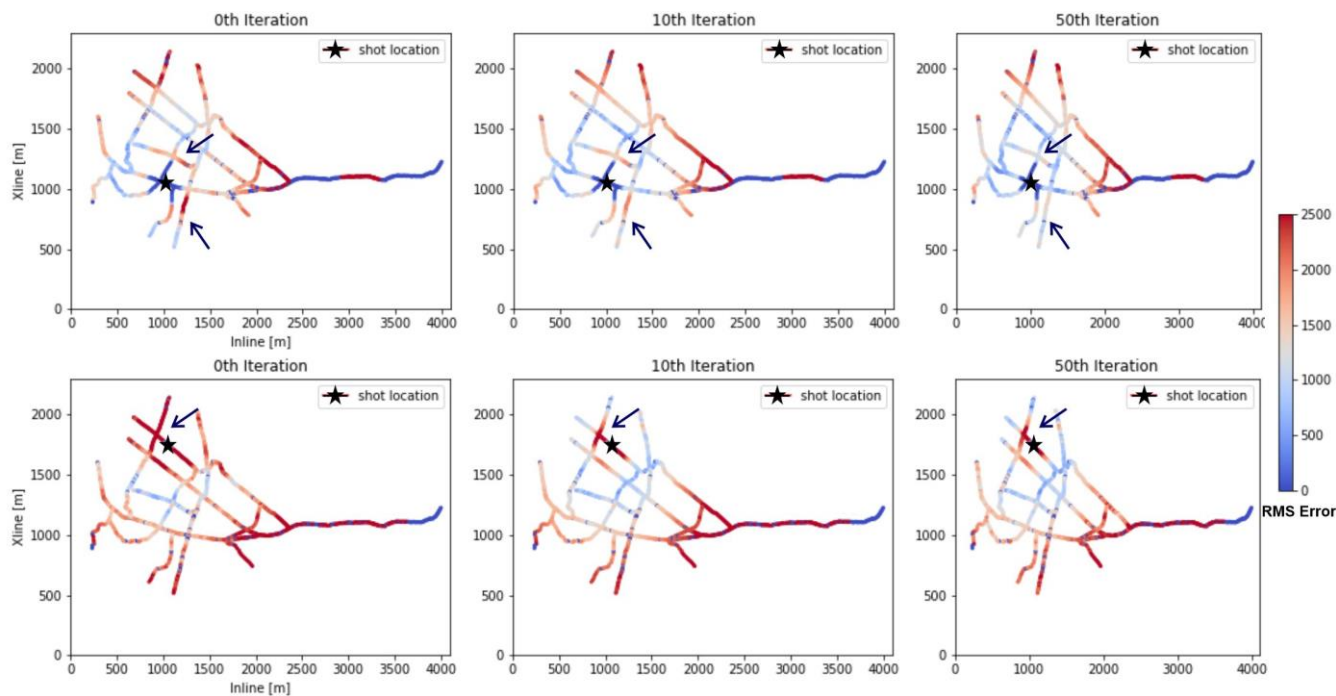
385 Figure 9: RMSE maps for two different shot locations showing the drop-in cost-function at different iterations. The drop in cost-function is mainly driven by near-to-intermediate offsets traces, while far offset traces has comparatively less reduction. Zero value corresponds with the traces which were omitted during the FWI.
