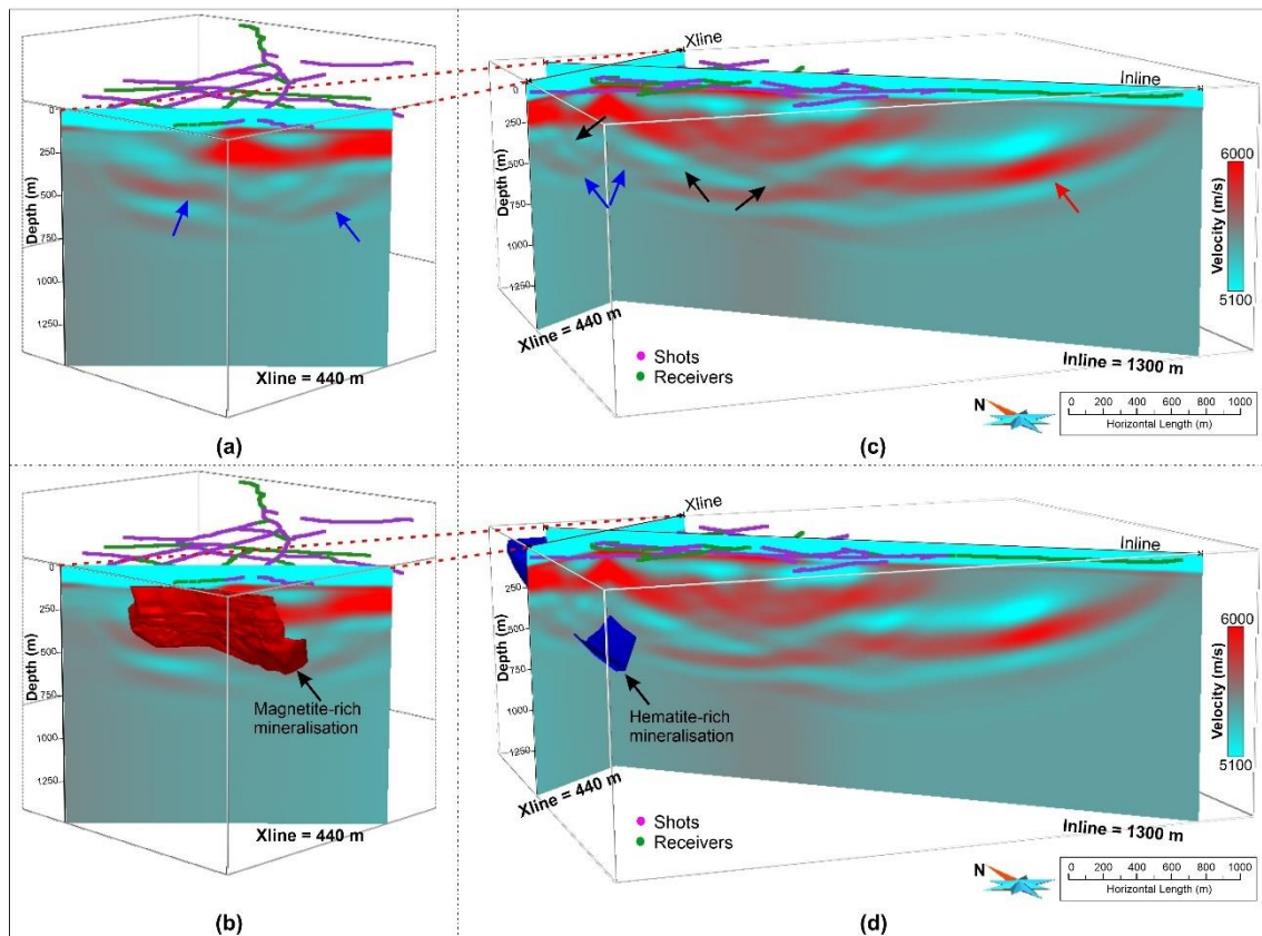
470 Figure 12: (a, b) Crossline view of the FWI derived velocity model, (c, d) Cross-sectional view of the FWI derived velocity model. Projection of the modelled mineralisation is shown in (b) and (d). Blue arrows mark high-velocity layers interpreted to be associated with mineralisation, black arrows show different geologically plausible fault structures and the red arrow shows artefact from FWI due to the one-sided illumination.
