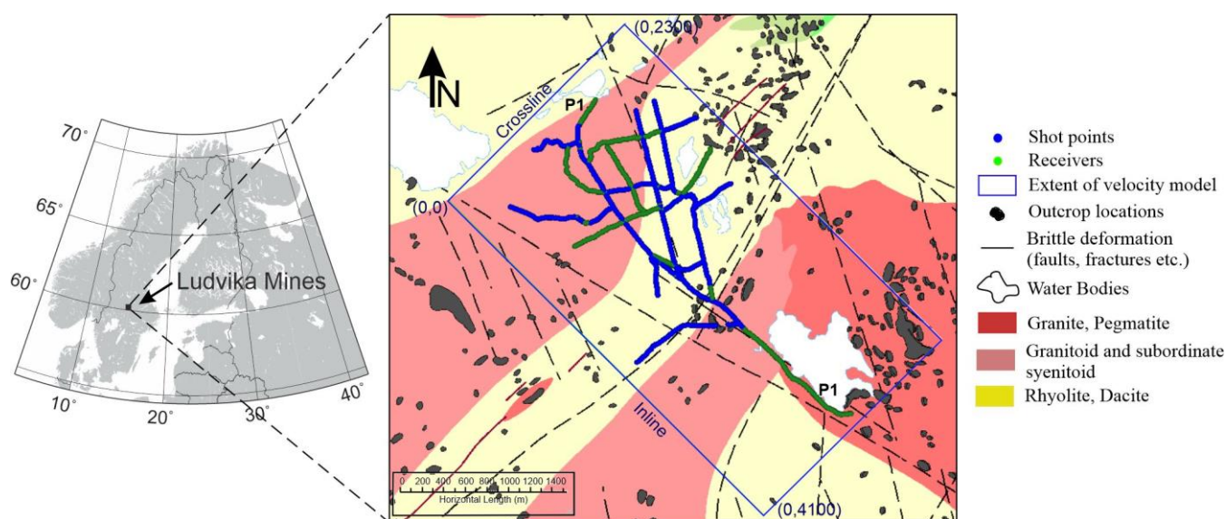
Figure 1: 3D data acquisition geometry at Blötberget and bedrock geology (modified after Geological Survey of Sweden). Receivers of the sparse 3D survey are shown by green dots and shots by blue dots overlapping the receivers. The rectangular blue box shows the extent of velocity model space used for FWI and subsequent depth imaging using RTM in local coordinates.
