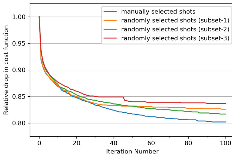
295 Figure 4: A plot showing the relative drop in cost-function for the inversion using different shot subsets. All the plots show that the inversion strategy is stable and effective, and does not depend significantly on the selection of shots as long as the uniform areal distribution of shots is followed across the survey area.
