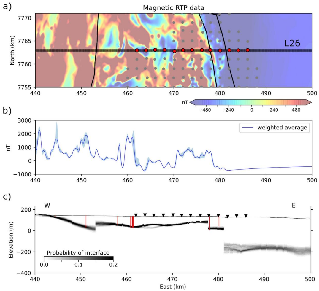
Figure 101010. Data preparation. (a) map view of the data in the region of interest. The grayed-out area corresponds to the zone considered for the averaging of the magnetic data. Red points are MT soundings considered in this study. Grey circles are others MT soundings not used in this study. (b) shows data for magnetic inversion (solid line) and the envelope of the data from the 800 meters band around L26 (light blue shade). The shades of blue represent the weight assigned to the data points in the calculation of the average: the lighter the shade, the lower the weight. (c) Depth of the eCover-basement interface probability p_{int} (Seillé et al., 2021). Red lines are the drill holes, and their bottom represent the intersection with the basement. The drill holes plotted are projected a distance up to 800 meters away from the profile.
