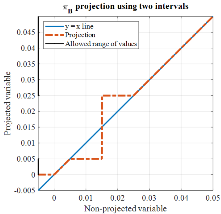
Figure A 111. Projection using \pi_B as per eq. 19 using two intervals as follows: [0, 0.005] , [0.025, +\infty[ . This example uses the intervals selected in the synthetic case study illustrating the proof-of-concept introduced in Sect. 3.
