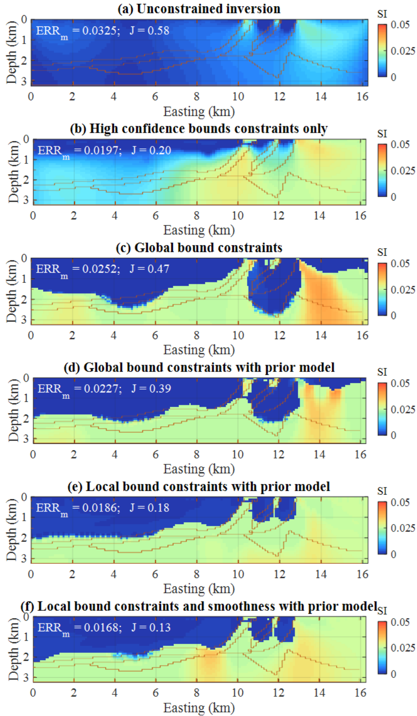
Figure 6. Inversion results for the different scenarios tested. Cases (a) through (ef) correspond to inversions using prior information and constraints summarised in Table 2 .
