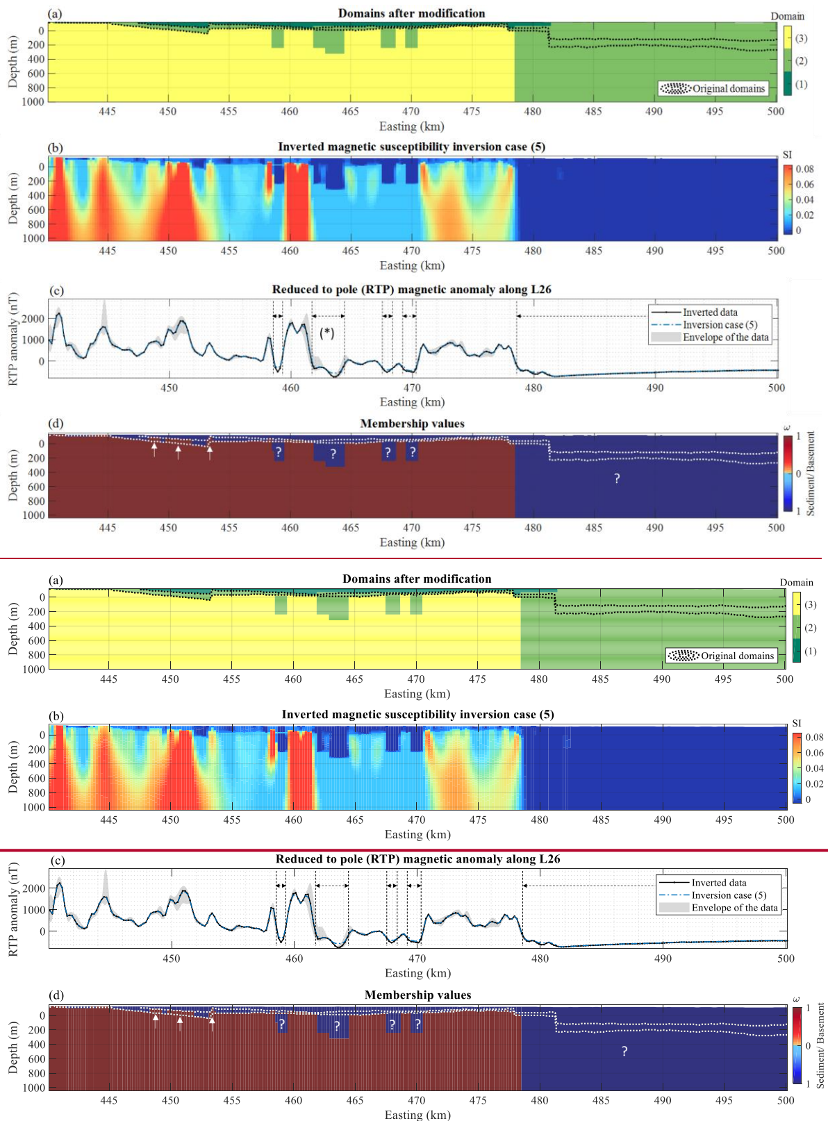
815 Figure 13. (a) MT-derived domains adjusted following the adjustments suggested by magnetic data inversion, for domains with (1) sedimentary units only, (2) sedimentary and non-sedimentary units and (3) non-sedimentary units only. (b) is the inverted model for inversion case (5) and (c) is the inverted and field magnetic RTP data, with the horizontal extent of the locations where MT bounds were are adjusted; (d) shows the membership values to the sedimentary and basement units obtained using eq. (10), overlaid with the original contours of MT-derived domains. In (c), the grey shading shows the envelope of the data shown in Figure 10 Figure 10 Figure 10 820
