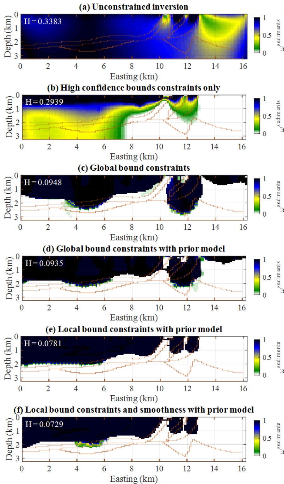
Figure 7. Membership values for the non-magnetic lithologies. Cases (a) through (f) correspond to inversions using prior information and constraints summarised in
