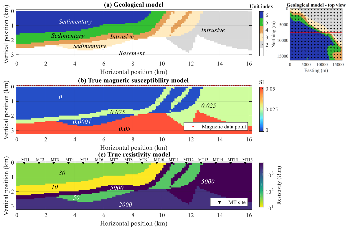
345 Figure 2. (a) True geological model (b) true magnetic susceptibility model and (c) true resistivity model with the simulated MT acquisition setup geometry in the top-left corner where triangles represent MT sites. The red dots in (b) represents the 2D magnetic data line; MT sites are marked in (c). The inset in the top-right corner shows a top view of the model with the magnetic data line in red and MT sites as triangles.
