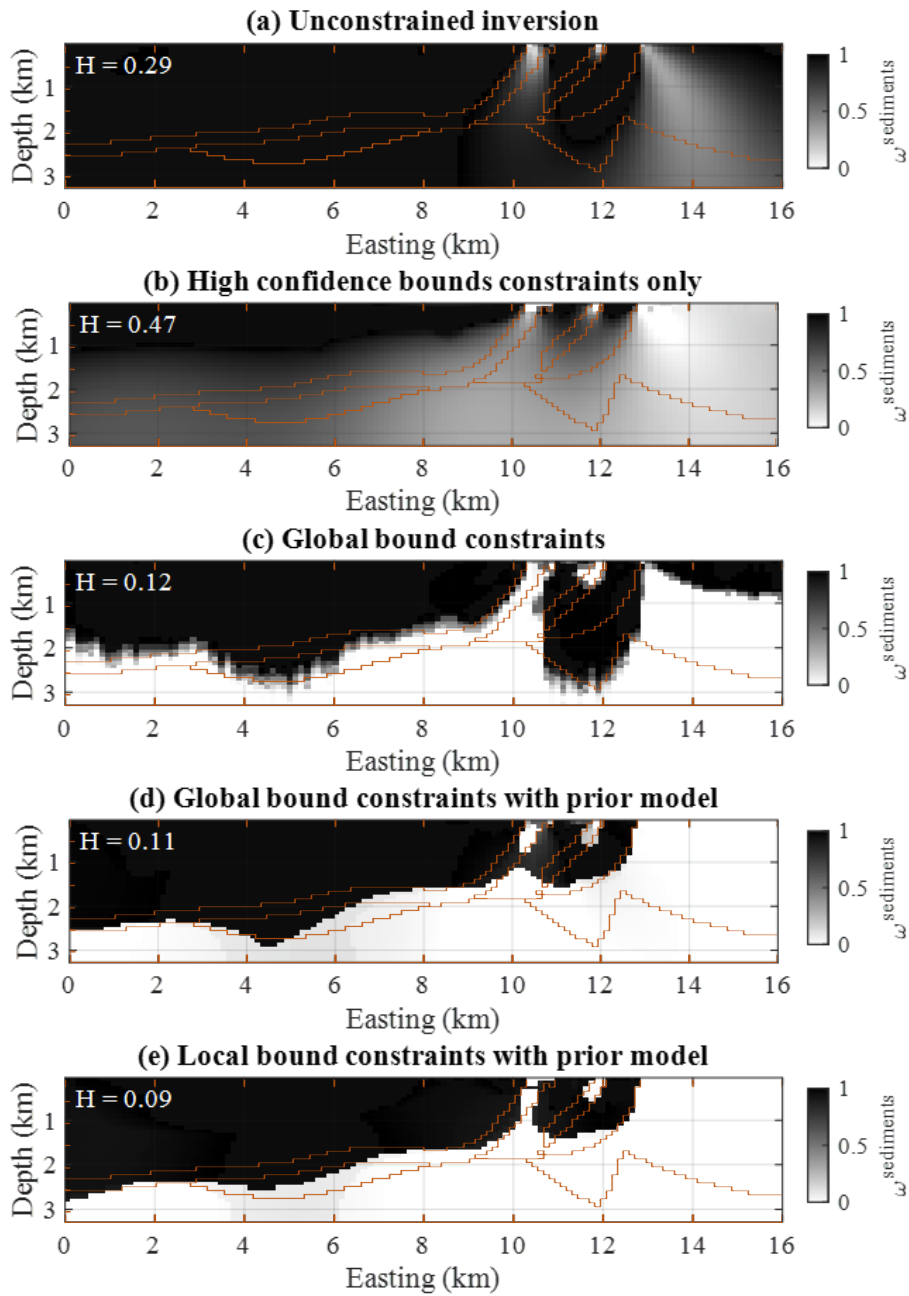
525 Figure 7. Membership values for the non-magnetic lithologies. Cases (a) through (e) correspond to inversions using prior information and constraints summarised in Table 2. The brown lines materialise the interfaces between geological units in the true model. H refers to the information entropy of the model (eq. 11).
