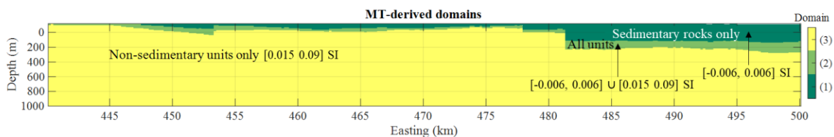
640 Figure 10. MT-derived domains for cases with (1) sedimentary units only, (2) sedimentary and non-sedimentary units and (3) non-sedimentary units only. The magnetic susceptibilities for the different domains are indicated on the Figure.
