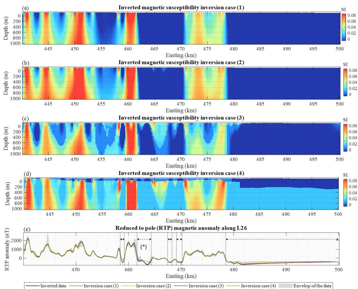
675 Figure 11. Inversion results. (a) through (d) correspond to inversion types (1) through (4), respectively; (e) shows the data fit for the 4 inversions shown. The grey shading shows the amplitude of the data shown in Figure 9 for calculating the weighted average of the inverted anomaly. The dashed lines mark the horizontal extension of areas where hypotheses made for magnetic inversion may be incompatible with the data.
