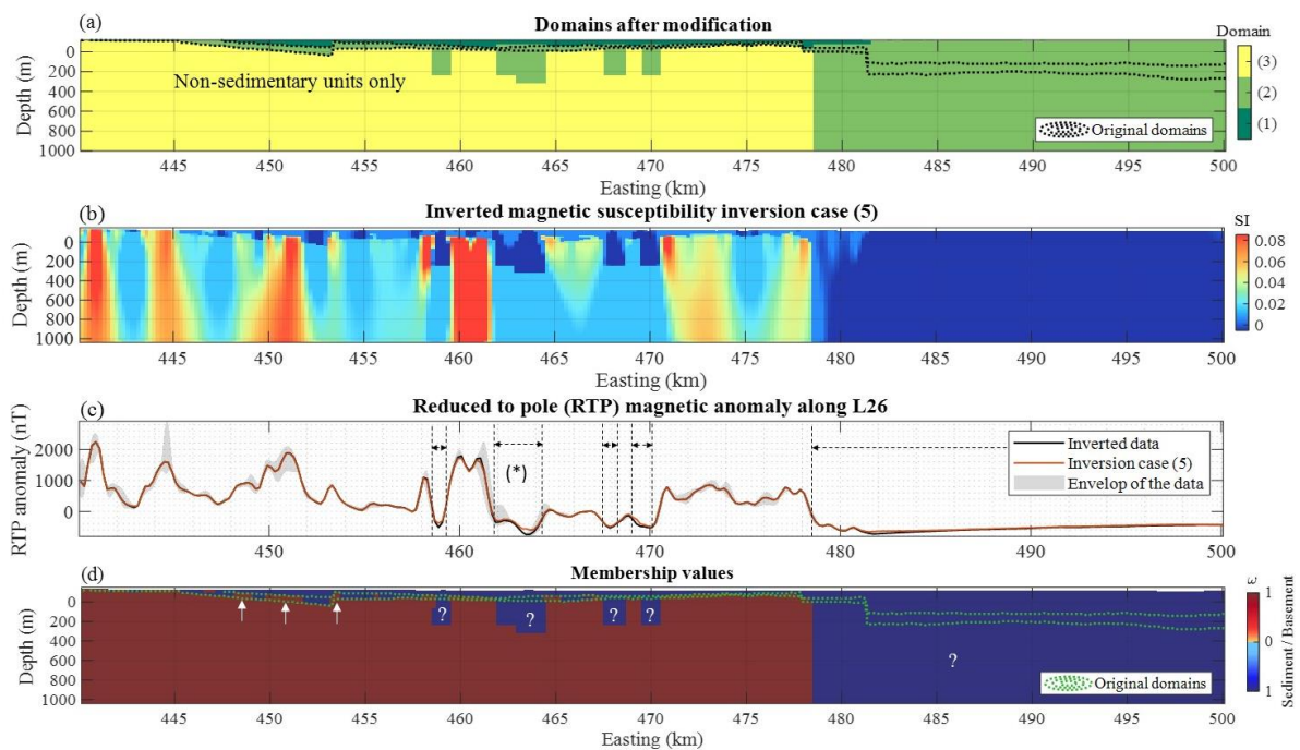
710 Figure 12. (a) MT-derived domains adjusted following the adjustments suggested by magnetic data inversion, for domains with (1) sedimentary units only, (2) sedimentary and non-sedimentary units and (3) non-sedimentary units only. (b) is the inverted model for inversion case (5) and (c) is the inverted and field magnetic RTP data, with the horizontal extent of the locations where MT bounds are adjusted; (d) shows the membership values to the sedimentary and basement units obtained using eq. (10), overlaid with the original contours of MT-derived domains. In (c), the grey shading shows the envelope of the data shown in Figure 9 for calculating the weighted average of the inverted anomaly.
