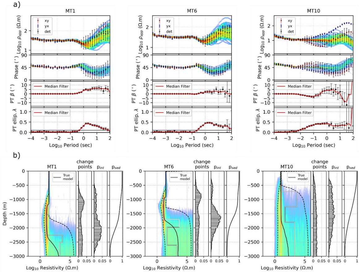
425 Figure 4. Example of posterior a) response and b) resistivity distributions for three MT sites MT1 in (left), MT6 in 430 (middle) and MT10 in (right), located along the profile as shown in Figure 2. In a) the phase tensor skewness \beta and ellipticity \lambda are shown. In b) the change points (interface probability distribution), the cover-basement interface probability distribution p_{int} and the sedimentary cover probability distribution p_{sed} are shown.. Sites MT1 and MT6 are located in in the basin, site MT10 is located in the area most affected by 2D/3D effects (see Figure 2c for location). High probabilities in the model posterior distribution is represented by warm colours, and low probabilities with cold colours. The dashed lines represent the 5 th and the 95 th percentiles of the model posterior distribution and the black line represents the median of the model posterior distribution. The white line is the true 1D model extracted beneath the MT station.
