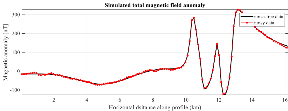
Figure 3. Simulated total magnetic field anomaly.
