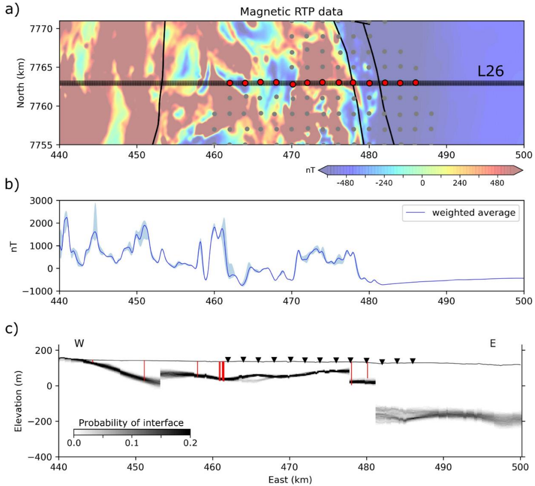
630 Figure 9. Data preparation. (a) map view of the data in the region of interest. The grayed-out area corresponds to the zone considered for the averaging of the magnetic data. Red points are MT soundings considered in this study. Grey circles are others MT soundings not used in this study. (b) shows data for magnetic inversion (solid line) and the envelope of the data from the 800 meters band around L26 (light blue shade). The shades of blue represent the weight assigned to the data points in the calculation of the average: the lighter the shade, the lower the weight. (c) Cover-basement interface probability p_{int} (Seillé et al., 2021). Red lines are the drill holes, and their bottom represent the intersection with the basement. The drill holes plotted are projected a distance up to 800 meters away from the profile.
