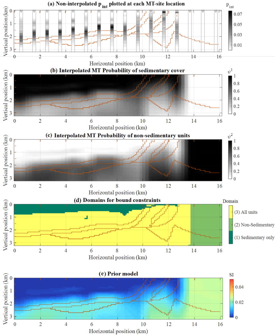
480 Figure 5. Probability of interfaces between sedimentary cover p_{int} and basements as recovered from MT inversion shown at the location of each MT site (a), interpolated probability of sedimentary cover written \psi^1 (b) and non-sedimentary units, written \psi^2 (c), corresponding domains (d), and (e) prior model from MT derived rock unit probabilities and magnetic susceptibility rock units observed in the area. The location of the simulated MT sites is reminded in (a). The brown lines materialise the interfaces between geological units in the true model.
