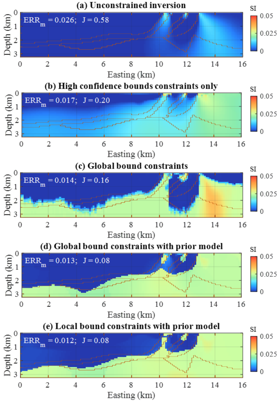
Figure 6. Inversion results for the different scenarios tested. Cases (a) through (e) correspond to inversions using prior information and constraints summarised in Table 2.
