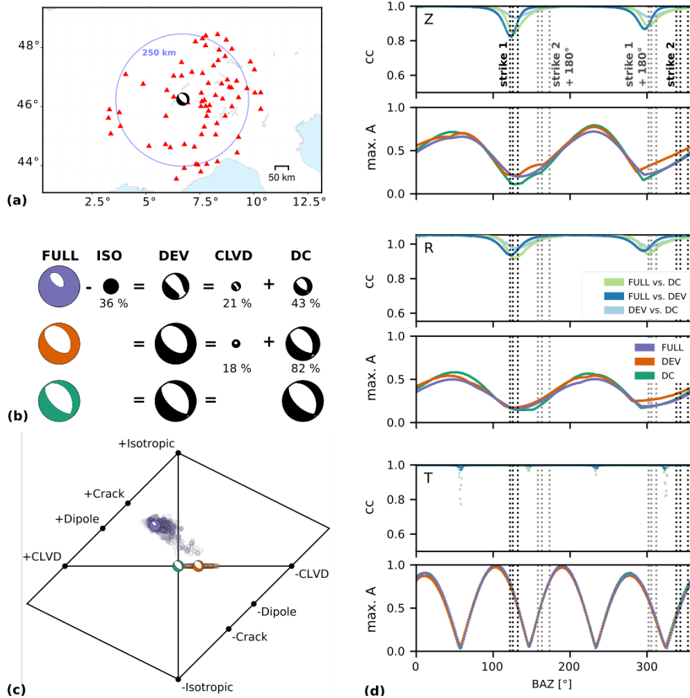
Figure 5. Earthquake close to Lake Geneva (France-Swiss border region), Mw 3.9, 2019-05-28 08:48:06. (a) Seismic network used for the MT inversions (73 broadband sensors, red triangles) and synthetic network (blue dots, in 1^\circ steps). (b) Decomposition of the full (purple), deviatoric (orange) and pure-DC (green) MT inversion solution with the smallest misfit. (c) Hudson plots showing the ensemble of solutions for the full and the deviatoric MT inversions, colors as in (b). Larger symbols depict best solutions of b. (d) For the three MT solution (full, deviatoric and DC) synthetic data were forward computed for the fictional network shown in (a). For each component (Z,R,T), the first row shows the maximum cross-correlation values of the three synthetic traces at each station (BP filter 0.02-0.1 Hz). The second row shows the maximum absolute amplitude at each backazimuth, normalized over the three solutions. The dashed lines indicate the strike 1 and 2 directions of the two nodal planes of full, deviatoric and DC solution and their 180^\circ equivalent.
