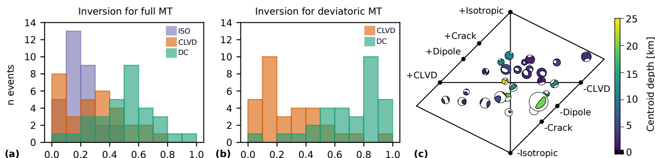
Figure 3. Histograms showing the decomposition of the full (a) and deviatoric (b) MT inversion results into isotropic (ISO), compensated linear vertical dipole (CLVD) and double couple (DC). Each bar of 10% width (x-axis) indicates for how many test earthquakes (y-axis) the proportion of decomposition is found. For example, an isotropic component of 10-20% is found for 13 test events in the full MT inversion. (c) Hudson plot showing non-DC components of individual events. Four events with Kagan angles > 60^\circ between full and deviatoric solutions were removed, since they were not well resolved. Color represents depth, beachball size magnitude.
