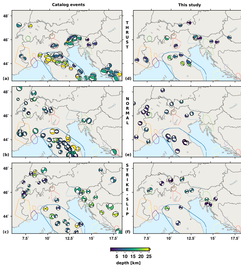
Figure 11. (a)-(c) Catalog depths of earthquakes shown in Fig. 9. (Depths might be fixed in some catalogs.) (d)-(e) Centroid depths of MT solutions in this study. Earthquakes are sorted according to their mechanisms: (top) thrust faulting events, (center) normal faulting events and (bottom) strike-slip events. The outlines of spatial clusters of increased seismic activity from Fig. 12a are indicated for comparison.
