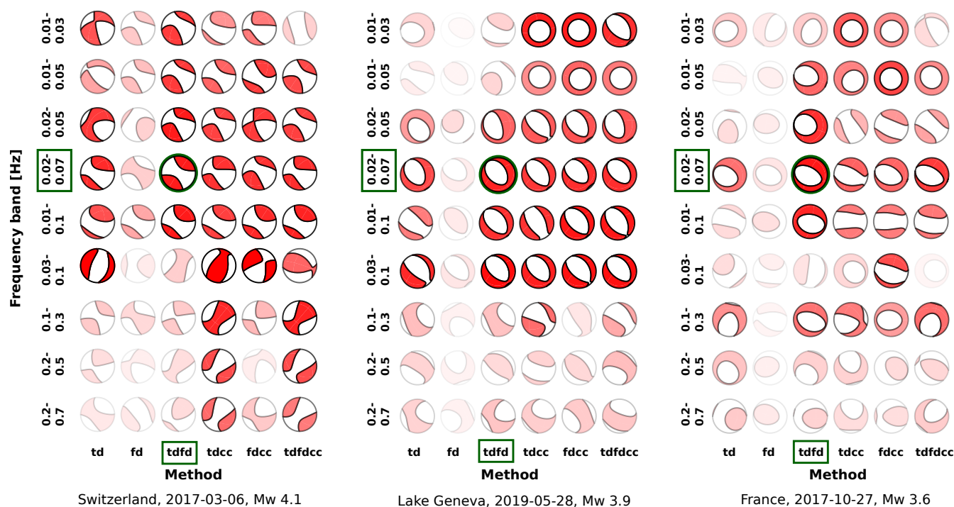
Figure 7. Testing of input data types and frequency ranges for three earthquakes with magnitudes between Mw 3.6 to 4.1. Abbreviations: td - time domain full waveforms; fd - frequency domain amplitude spectra; cc - cross-correlation fitting of full waveforms; tdfd, tdcc, fdcc and tdfdcc are combinations of these. Color intensity represents summed uncertainty of MT components. A combination of fd and td in a frequency band between 0.02-0.07 Hz yields the best results for Mw > 3.3 (marked in green).
