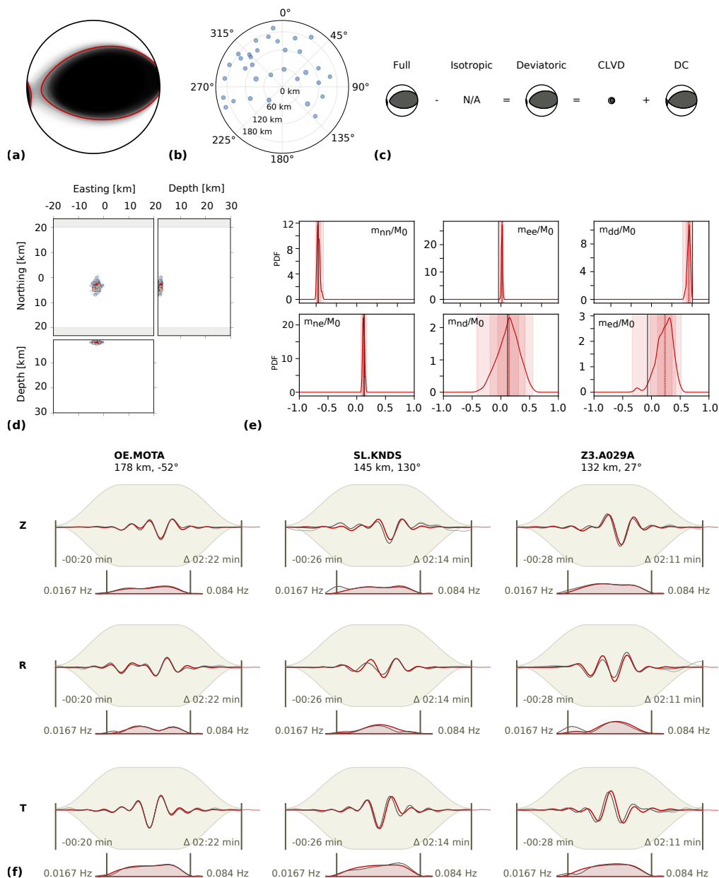
Figure 2. Example MT inversion result, 2019-06-14, Mw 3.9, NE Italy. (a) Fuzzy beachball illustrating the MT solution uncertainty. (b) Station distribution around the epicenter. (c) Decomposition of the best MT solution into DC and CLVD component. (d) Resolution of the centroid depth, easting and northing relative to the starting position. (e) Probability density functions (PDF) showing the resolution of the six independent MT components m_{xy} normalized by the seismic moment M_0 . (f) Examples of waveform and spectral fits at three stations and three components. Red and black lines indicate synthetic and recorded waveform data, respectively. Station name, azimuth and distance to the epicenter above each column. Numbers within the panels describe the time window and the frequency band.
