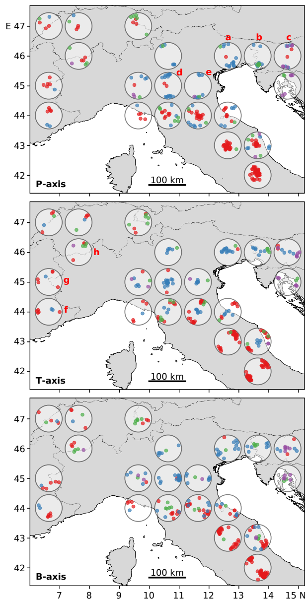
Figure 10. Regional distribution of P-, T- and B-axes of focal mechanisms presented in Fig. 9. Colors correspond to mechanism classes as shown in Fig. 9. Only areas with more than five events in a latitude-longitude-grid of 1^\circ \times 1^\circ are shown. a to h mark features which are discussed in the text.
