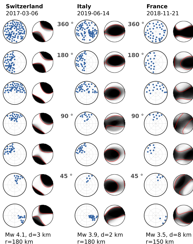
Figure 8. Resolution of the deviatoric MT depending on the azimuthal station coverage for three earthquakes with magnitude M_w , centroid depth d and event-station radius r given below (left, middle and right panels). The station coverage (blue dots in 1st, 3rd, 5th column) decreases from top to bottom as indicated in between the event-columns. The fuzzy MTs show the solution stability. They are composed of the superimposed P radiation pattern of the ensemble of solutions from the bootstrap chains.
