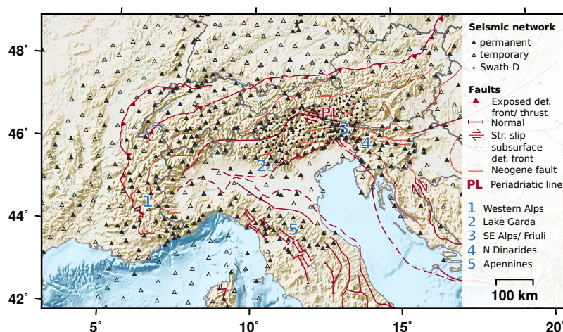
Figure 1. Study area and AlpArray seismic network. Subregions that are discussed in greater detail in this study are numbered. Exposed and subsurface faults simplified from Schmid et al. (2004, 2008); Handy et al. (2010, 2015) and Patacca et al. (2008). Topographic data from SRTM-3 (Farr et al., 2007) and ETOPO1 (Amante and Eakins, 2009) datasets).
