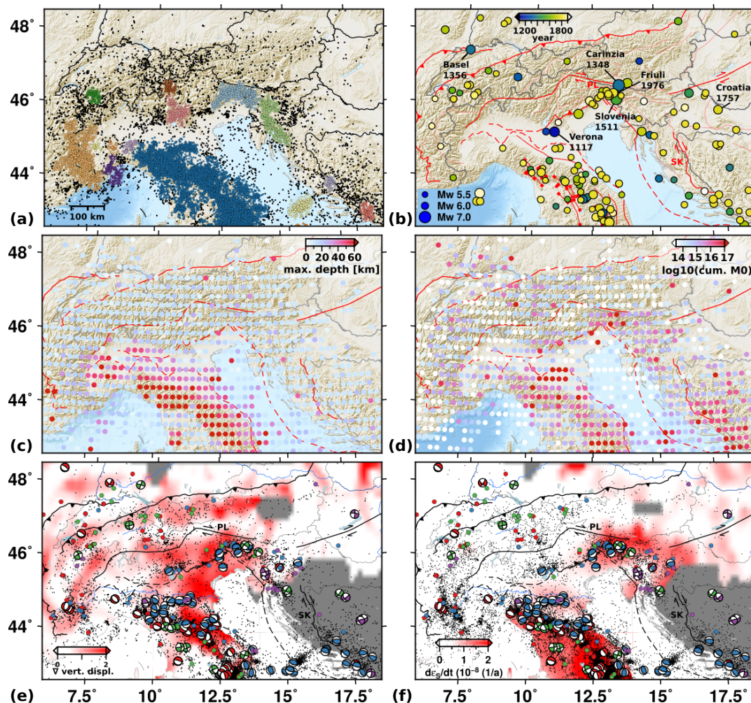
Figure 12. Characteristics of recent and historic seismicity and strain from GNSS data. (a) Seismic activity between 1978-2017, M_I > 2.0 , from GEOFON, INGV and gCMT catalogs, colored according to epicentral clusters of seismicity. (b) Historic earthquakes with M_w > 5.5 from the European Archive of Historical Earthquake Data 1000-1899 (AHEAD) (Locati et al., 2014; Rovida and Locati, 2015; Stucchi et al., 2013) and ISC-GEM catalog (1906-2016) (Storchak et al., 2013, 2015; Bondár et al., 2015; Di Giacomo et al., 2015, 2018). (c, d) Maximum event depth and the cumulative seismic moment on a grid with a spacing of 0.25 \times 0.25^\circ lat. and lon. (e, f) Absolute value of the spatial gradient of the relative uplift rate as a proxy for vertical strain rates and observed GNSS shear strain rate (max. shear strain). Both obtained from GNSS data of the EUREF WG on European Dense Velocities (Brockmann et al., 2019). Grey dots indicate earthquakes without MTs, as in (a). Events with MT solutions are color-coded as in Fig. 9. For simplicity, focal mechanisms are only plotted for representative events with M_w \geq 4.0 . Exposed and subsurface faults (solid and dashed lines) simplified from Schmid et al. (2004, 2008); Handy et al. (2010, 2015) and Patacca et al. (2008). 'PL' marks the Periadriatic line, 'SK' the Split-Karlovac Fault. Topographic data from SRTM-3 (Farr et al., 2007) and ETOPO1 (Amante and Eakins, 2009) datasets).
