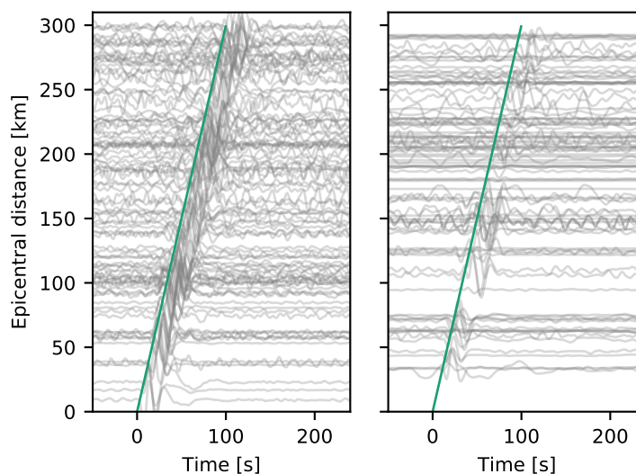
Figure 6. Vertical component seismograms of permanent AASN stations, sorted by distance. (left) 2017-03-06, Mw 4.1, Switzerland, (right) 2017-10-27, Mw 3.6, France. Time in seconds after origin time. Waveforms bandpass filtered between 0.02 and 0.07 Hz. Rayleigh waves dominate the seismograms in this frequency range with an average phase velocity of 3 km/s (green line).
