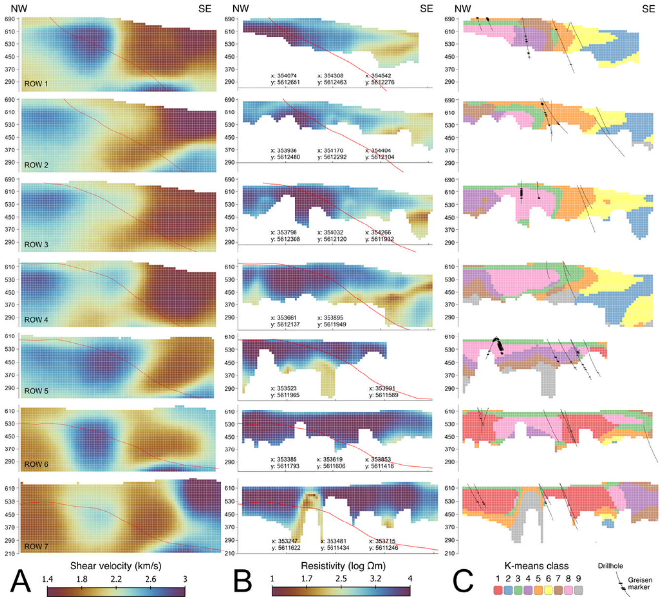
615 Figure 12: Vertical sections (220 m spacing) through the combined shear velocity–resistivity model showing (A) shear velocity, (B) resistivity, and (C) classification. Sections are oriented NW-SE. Northernmost section is at the top, southernmost at the bottom. Red line marks the transition between granite (NW) and two-mica schist (SE). Drill holes and greisen markers in (C) are projected into the section from a distance of up to 50 m.
