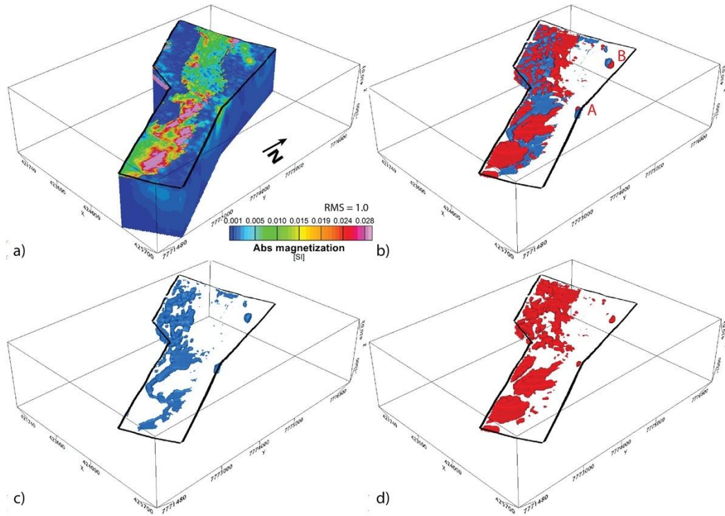
450 Figure 6. Results from the MVI test, where cells associated with sediment units were constrained towards a non-magnetic reference 455 model, while cells associated with magmatic rocks remained unconstrained. Only the shallow central part of the model down to a depth of 1000 m is shown which was covered by data from the fixed wing survey (black polygon). (a) The final magnetization distribution is presented as absolute values of the magnetization vectors. (b) Only cells with absolute magnetization values > 0.01 SI are shown as iso- surfaces. Blue and red colours are associated with locations where the z-component of the magnetization points out of the ground (z- component is positive) and into the ground (negative z-component), respectively. These two contributions are presented separately in (c) and (d).
