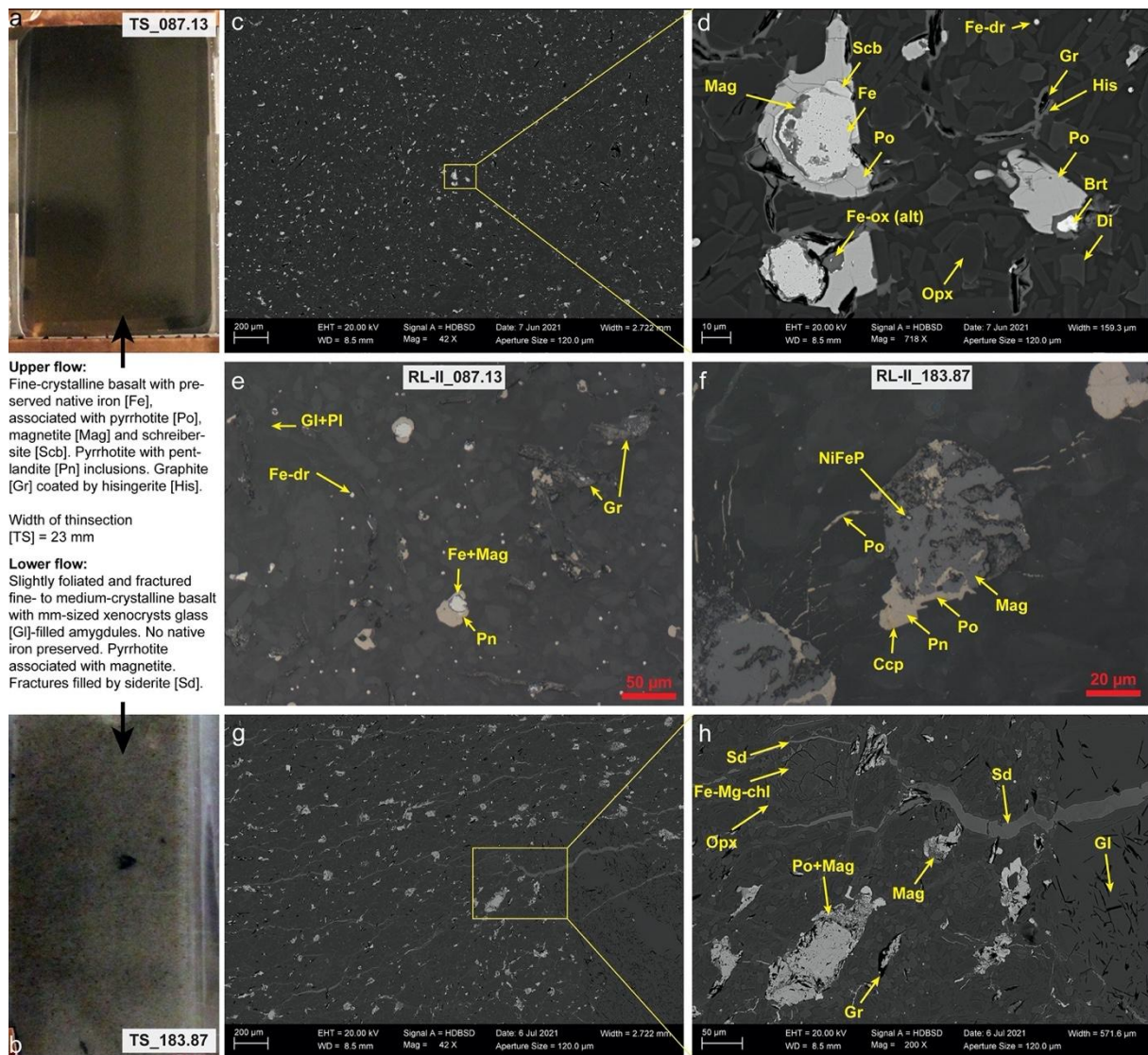
575 Figure 11. (a) Photograph of a polished thin section of a fine crystalline basalt sample from the upper flow (87.13 m core depth); (b) Photograph of a polished thin section of a fine to medium crystalline basalt sample from the lower flow (183.87 m core depth); (c) to (d) Backscatter electron micrographs (BSE) of sample at 87.13 m depth with preserved native iron (Fe) blebs and Fe-droplets (Fe-dr) and minor magnetite (Mag) and Fe-oxide (Fe-ox) in association with pyrrhotite (Po), schreibersite (Scb) and graphite (Gr) and hisingerite (His). Brt = barite, Di = diopside, Opx = orthopyroxene; (e) Reflected light micrograph of the same sample with larger native Fe blebs with a magnetite rim and association with pyrrhotite and smaller micron-sized Fe-droplets dispersed in matrix; (f) Reflected light micrograph of sample at 183.87 m core depth with no preserved native Fe, but magnetite in association with pyrrhotite. Pyrrhotite with pentlandite (Pn) flames and chalcopyrite inclusions; (g) to (h) Backscatter electron micrographs (BSE) of the same sample with pyrrhotite in association with magnetite and graphite and siderite (Sd)-filled fractures that also cross-cut a glass (Gl)-filled amygdule. Fe-Mg-chl = Fe-Mg-chlorite. 580
