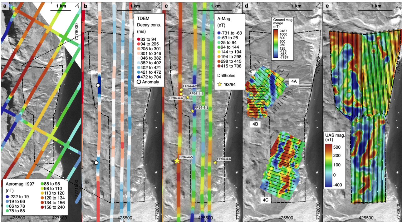
325 Figure 3. Overview of legacy airborne geophysical (time-domain electromagnetic (TDEM) and magnetic), ground-based magnetic and UAS-based magnetic data with the dashed line highlighting the UAS-based magnetic survey area of this study. The residual magnetic anomalies are shown (a) from the regional AEROMAG97 survey (Thorning and Stemp, 1998), (b, c) from the local exploration airborne survey (Olshefsky and Jerome, 1993) and (d) from ground-based surveys, conducted by Falconbridge Ltd. (grid 4A; Olshefsky and Jerome, 1995), and collected during our field campaign (grid 4B and 4C). The UAS-based magnetic anomaly map is shown in (e) for comparison. The decay constant determined from the electromagnetic data is shown in (b). Two conductivity anomalies were identified (white dots) that were considered as targets for further exploration (Olshefsky and Jerome, 1993). The flight trajectories are shown as black lines, and positions of legacy drillholes are indicated in (c) as stars.
