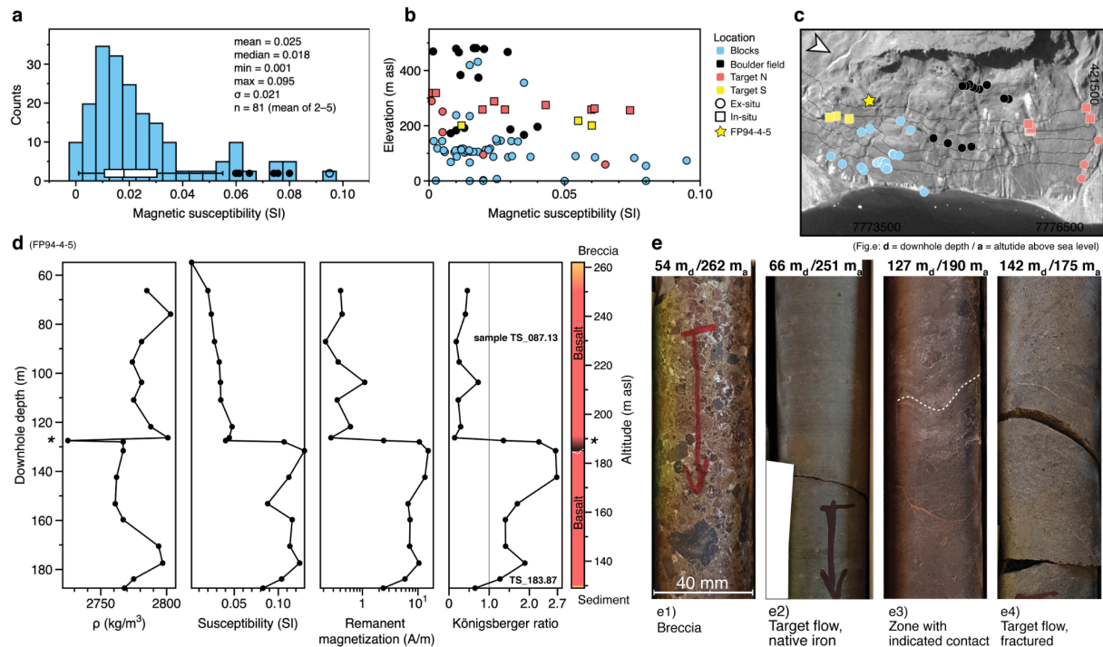
550 Figure 10. Ground-based susceptibility measurements and petrophysical logs from the drillhole FP94-4-5, based on our measurements. (a) Magnetic susceptibility distribution from handheld measurements. (b) Magnetic susceptibility is plotted against altitude (in m asl) with a
