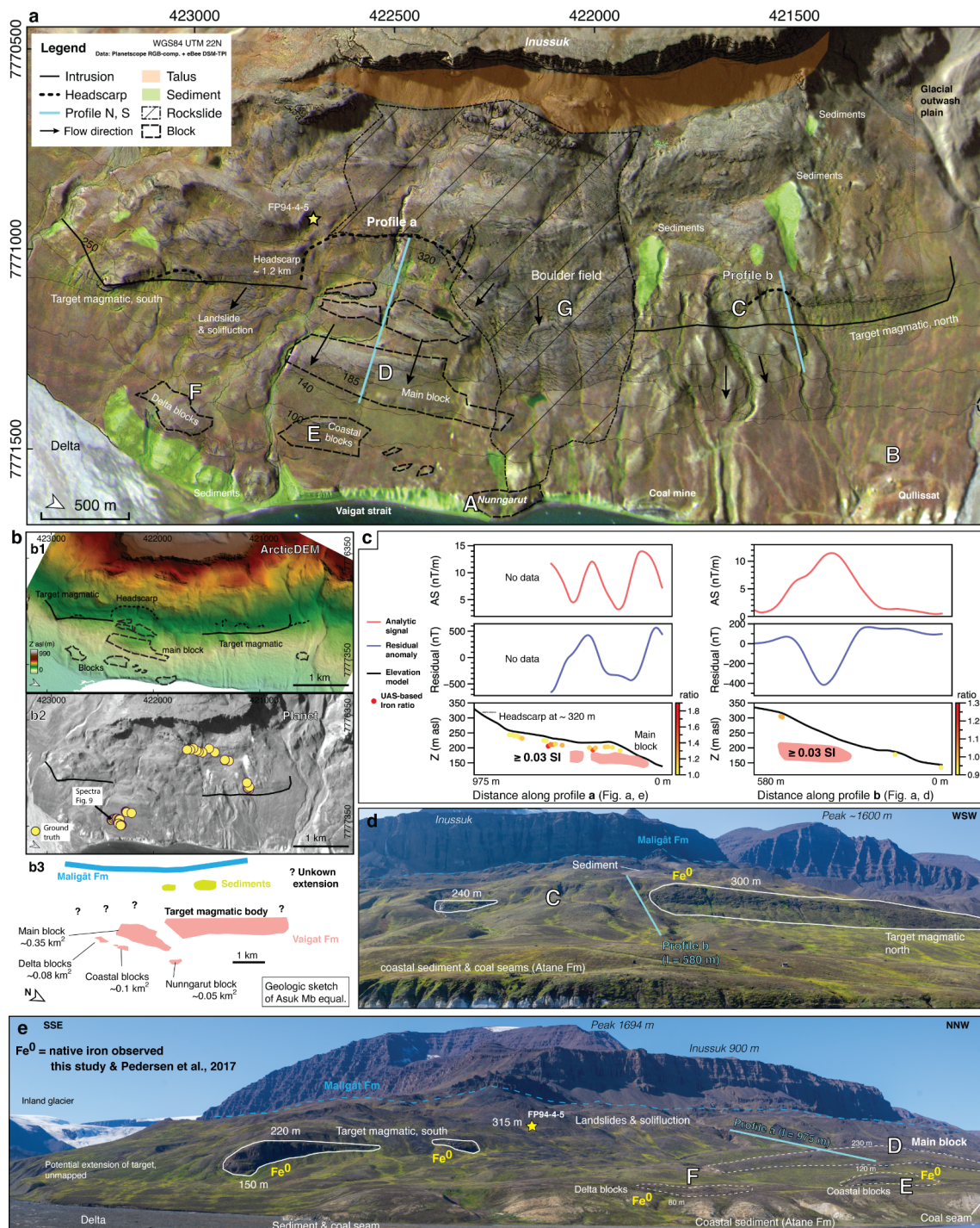
670 Figure 14. Integrated interpretation. (a) RGB-composite plot from PlanetScope images (Planet Team, 2021) that are merged with semi-transparent TPI from the eBee DSM to increase image contrast. Landslide features are marked as dashed lines with thin lines for larger blocks and thick lines for the main landslide scarp. Talus below the Inussuk and block fields are the source for numerous boulders in the whole area. Mapped sediments reach up till the foot of the Inussuk cliff. (b) Overview maps illustrate area in relation to the different data,
