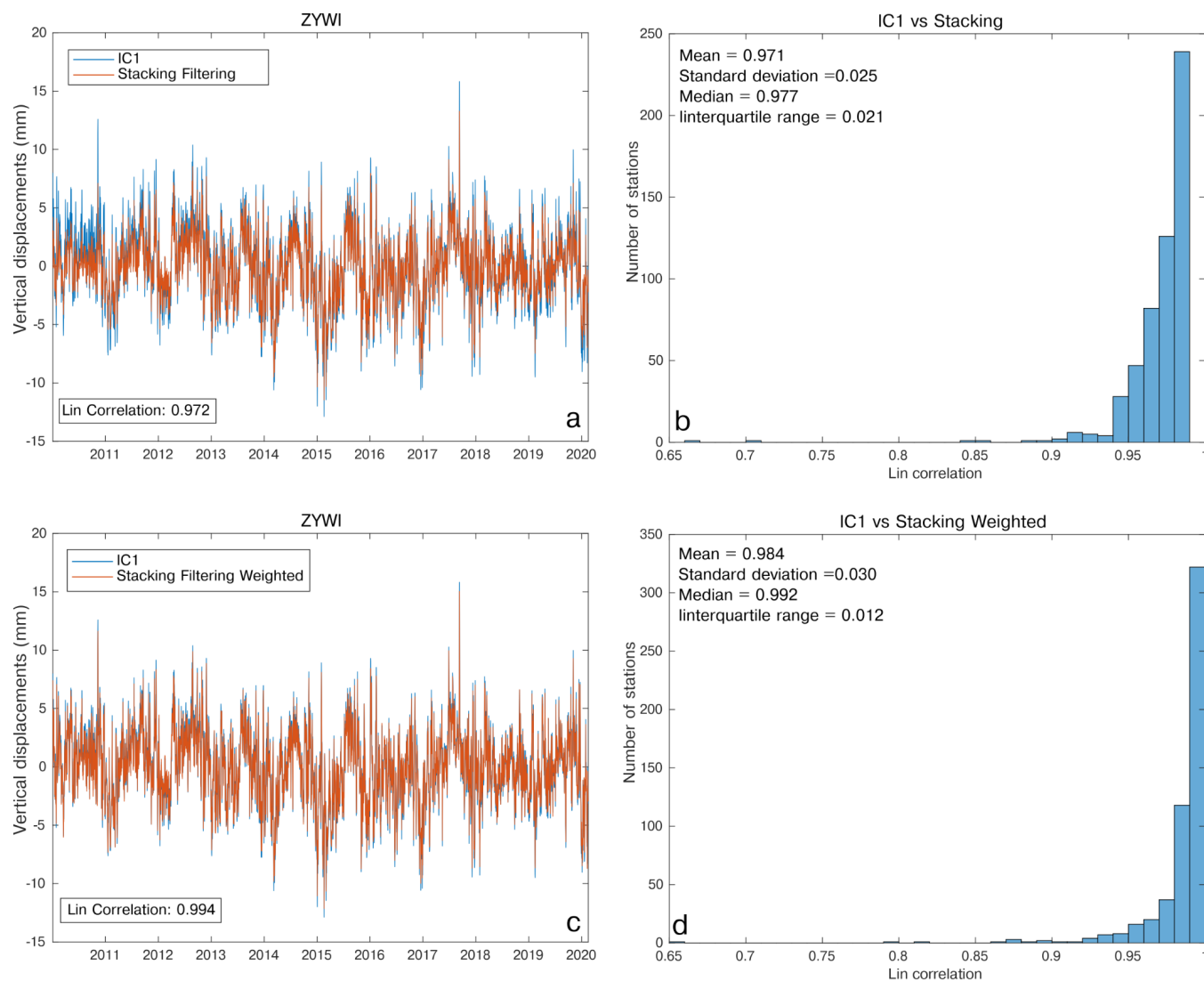
Figure 13: Comparison between the displacement associated with IC1 at the ZYWI site and the CME estimated with the Stacking Filtering Method (a) and the Weighted Stacking Filtering Method (c). We also show the histogram representing the Lin correlation between the displacements associated with the IC1 and the CME estimated with the Stacking Filtering Method (b) and the Weighted Stacking Filtering Method (d) at each site. We point out that the CME computed with the aforementioned methods is, by definition, the same at each station; whereas the
