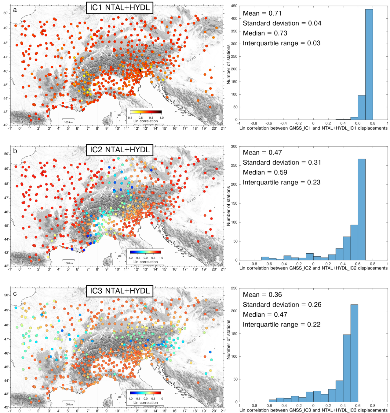
Figure 7: Lin correlation coefficients between: a) GNSS-IC1 and NTAL+HYDL_IC1; b) GNSS_IC2 and NTAL+HYDL_IC2; c) GNSS-IC3 and NTAL+HYDL_IC3. Histograms of the correlation coefficients are also reported.
