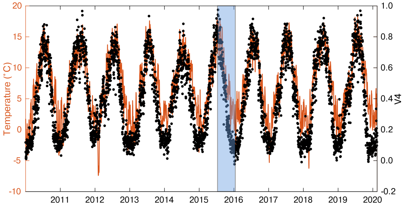
Figure 9: Comparison between the daily mean temperature of the study area (orange) and the temporal evolution of IC4 (black dots). The shaded area represents the time interval associated with the maximum displacements shown in Fig. S15.
