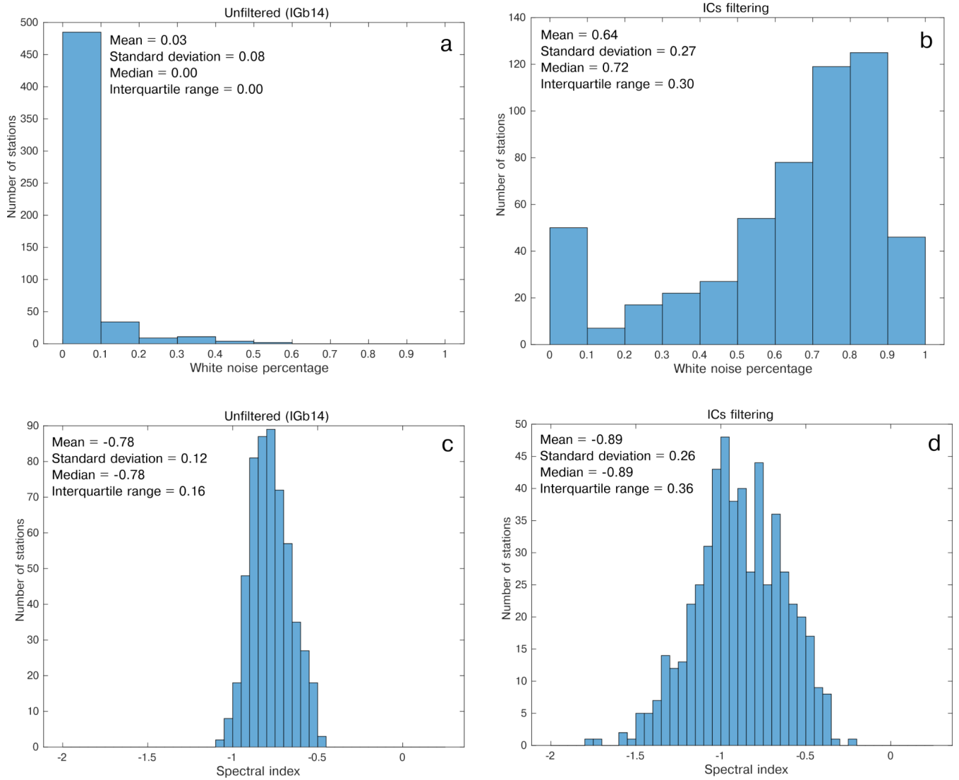
Figure 12: Histograms of: (a) white noise percentage in the unfiltered time-series and (b) filtered time-series. (c), (d) same as (a) and (b) for the spectral index. The filtering is done by subtracting the displacements associated with the first 4 ICs.
