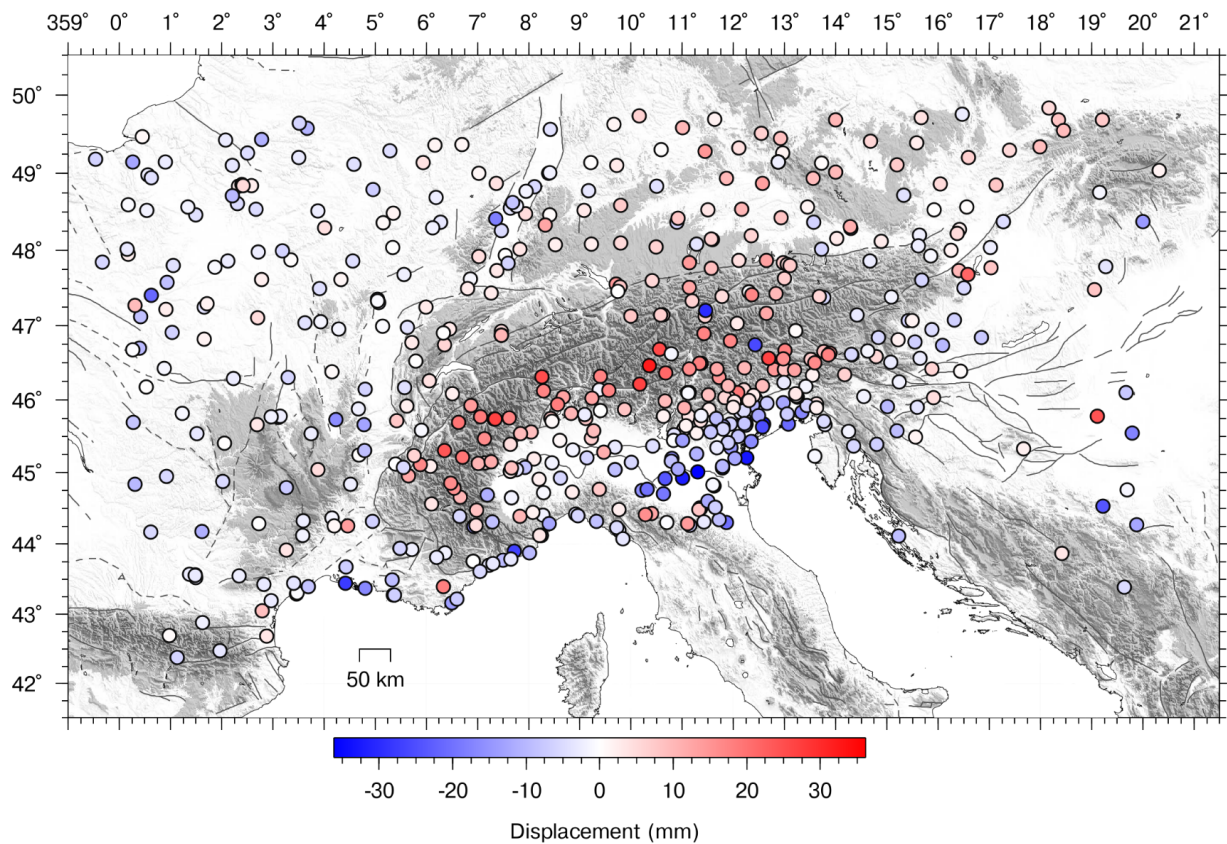
Figure 2: Temporal evolution and spatial response of the IC2 of the GNSS decomposition. Time series have been corrected only for instrumental offsets.
