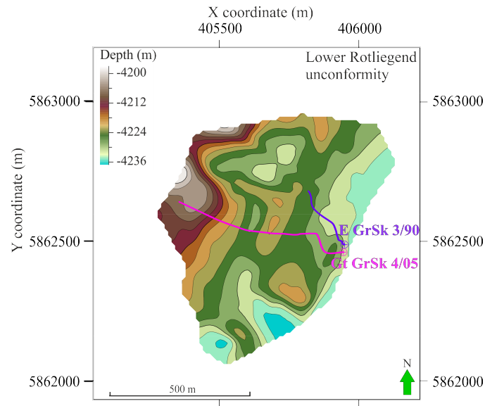
Figure 11. Spatial distribution of the unconformity boundary. Depth of the Lower Rotliegend unconformity.
