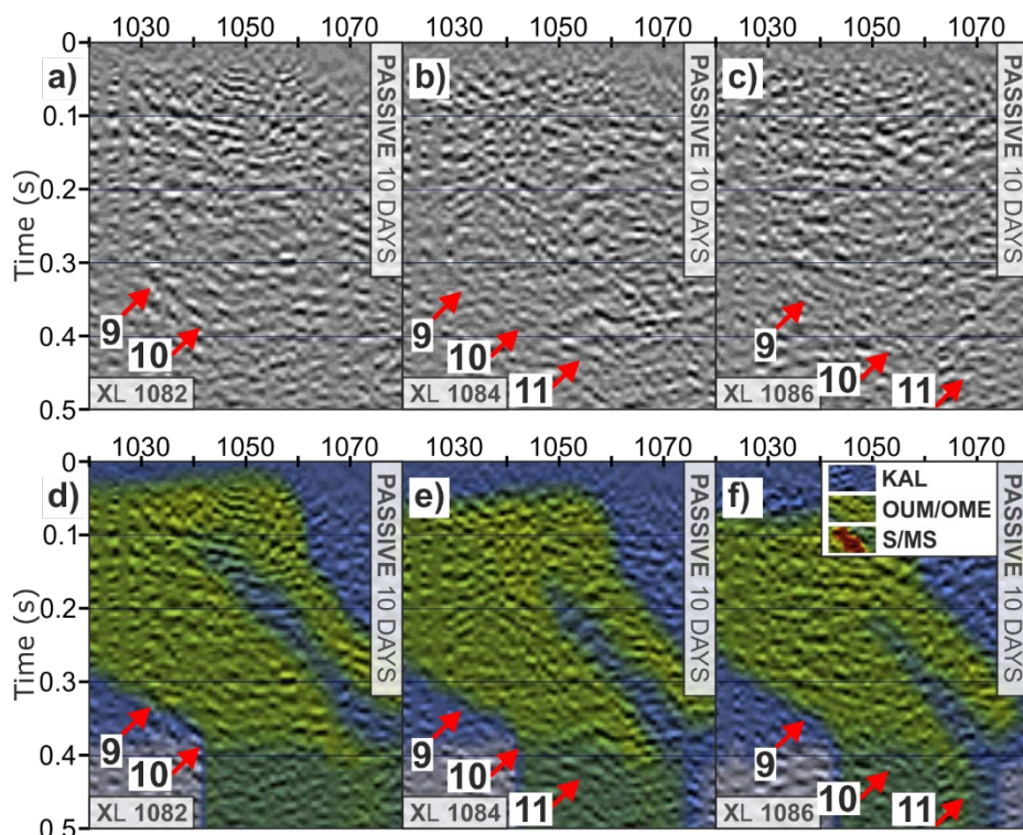
450 Figure 9: Comparison of post-stack migrated sections obtained from the 3D virtual-source survey along crosslines: 1082 (a) and (d), 1084 (b) and (e), 1086 (c) and (f). Red arrows mark the reflection events that are associated with a key contact within the Kylylahti formation (OUM/OME in contact with black schists (KAL)). Note that extent of the geological model shown is constrained by the borehole data, and the marked reflections are at the very edge of this extent. The Kylylahti formation continues beyond the shown extent with further repetitions of the OUM/OME units with black schist inter-layers. The arrows with numbers show reflections that are interpreted in the text. The geological model (described in section 2) displayed in the background is color-coded as follows: S/MS mineralisation (red); OUM/OME units (green); KAL unit (blue).
