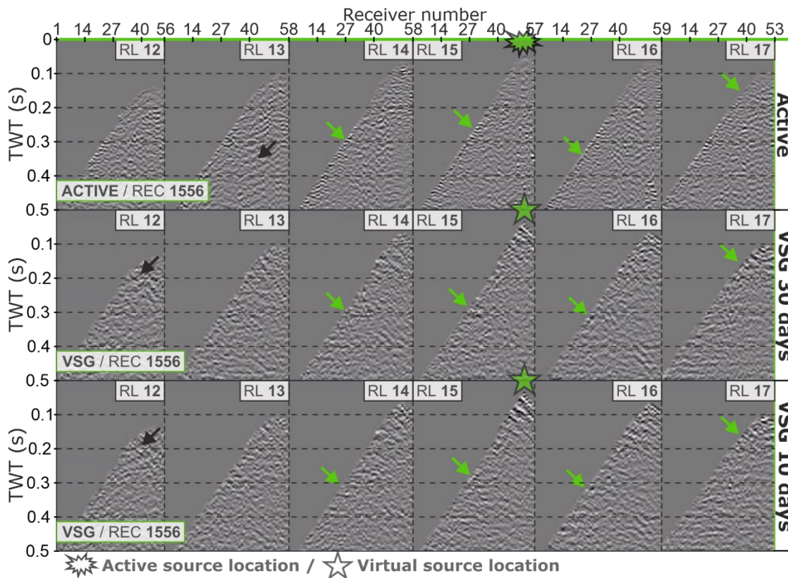
Figure 7: Comparison of exemplary co-located 3D common-source gathers using active and passive data. The active-shot gathers are filtered using bandpass filter (25-35-90-120 Hz) to have the frequency content of the passive data. For each gather, we show 6 receiver lines (RL). Common-source gathers collocated with receiver station 1556: (top row) active-shot gather, (middle row) VSGs obtained using 30 days of noise, (bottom row) VSGs obtained using 10 days of noise. The green arrows on both active and passive data highlight position of reflection arrivals observed in active source data and projected on collocated VSGs. Black arrows indicate artifacts characteristic for passive data. TWT stands for two-way travelttime.
