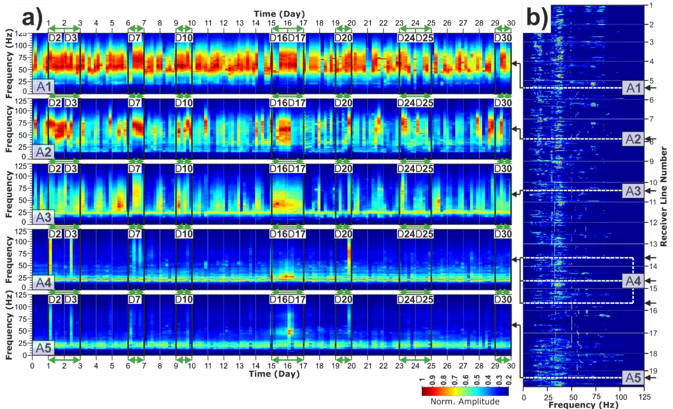
195 Figure 3: Temporal (a), and spatial (b) variation of noise spectrograms. a) Each panel represents power spectral densities (PSDs) computed for each day of recording using receiver stations located in the representative areas highlighted in Figure 1. Days highlighted with green arrows correspond to beamforming panels highlighted with green circles in Figure 4a. b) PSD for a single day of recording using every receiver station of the Kylylahti array. White dashed lines highlight receiver stations corresponding to the representative areas shown in (a). Amplitudes are independently normalized at each panel. Two regimes of high power density are observed at frequency ranges 10-30 Hz, and 40-90 Hz.
