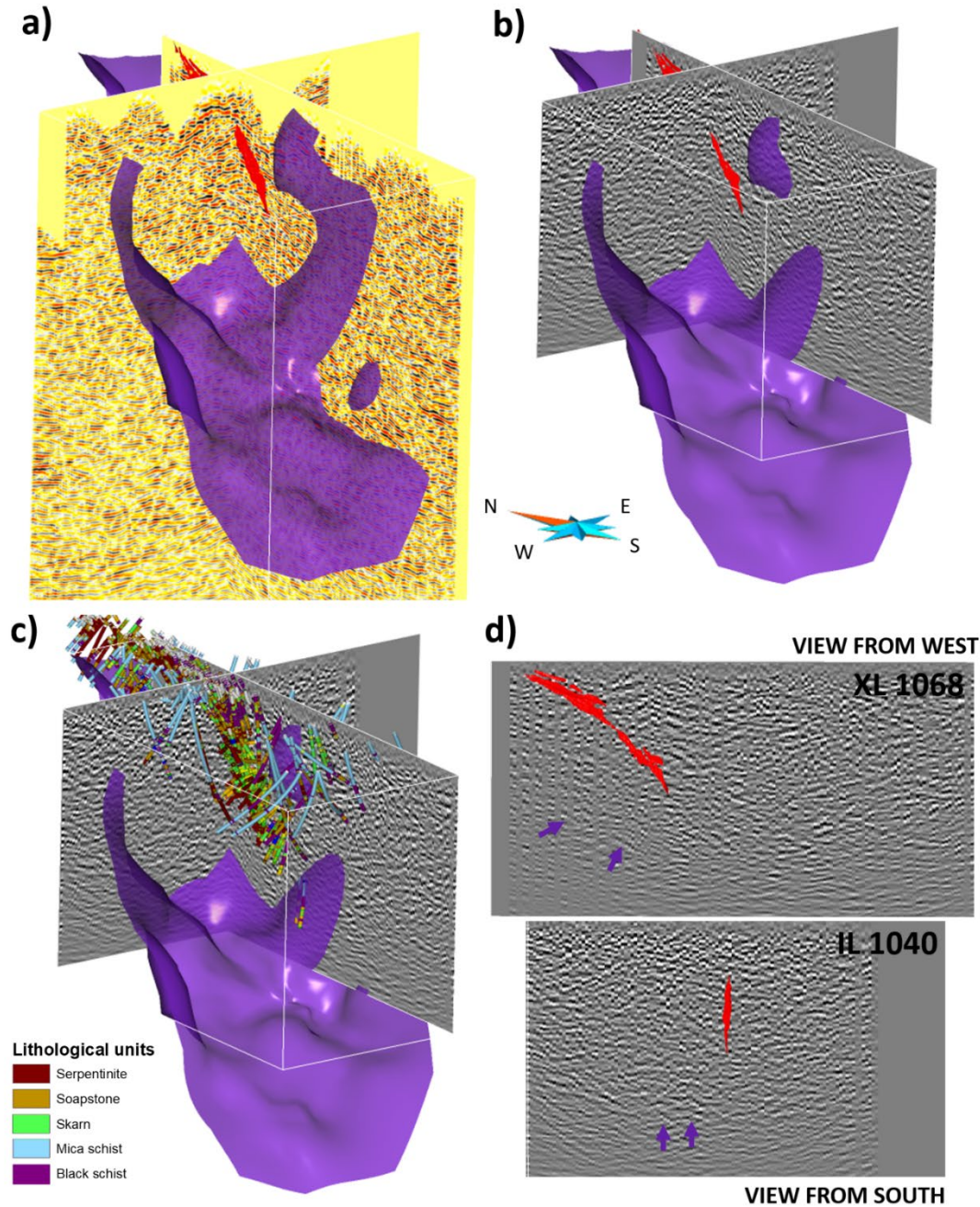
Figure 10: (a) The Kylylahti active-source 3D data processed with a similar 3D reflection seismic processing workflow as the passive 3D 10-day subset data shown on (b), and overlapping the crossline 1068 and inline 1040 of the passive 3D cube of figure (b). The purple surface
