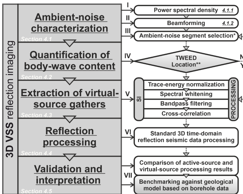
170 Figure 2: Summary of the 3D virtual-source survey methodology for the purpose of near-mine mineral exploration. The left column presents the core of the flowchart: it contains five main processing blocks representing subsections 4.1-4.5. The detailed processing steps performed within each main processing block are shown in the right column. The sequence of processing is indicated by roman numerals. Gray-gradient- colored blocks in the right column indicate our modifications of the state-of-the-art ambient-noise imaging workflow proposed by Draganov et al. (2013). Single star symbol denotes the user-dependent 'Ambient-noise segment selection' processing step, in which the initial selection is based on the beamforming results, and later verified by TWEED. Double star symbol denotes the location procedure, which supports the 175 TWEED verification, but is not mandatory.
