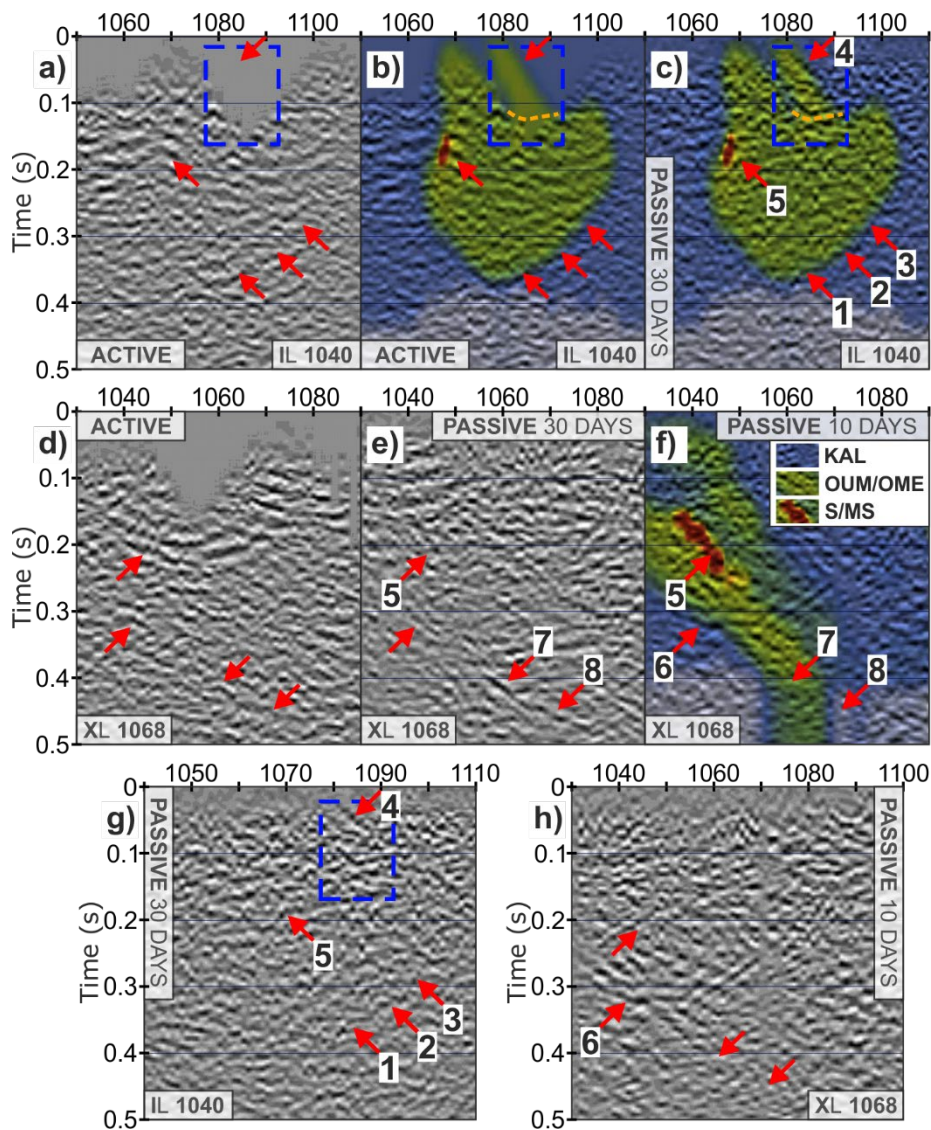
Figure 8: Comparison of post-stack migrated sections obtained from the active and passive surveys. Inline 1040 (a)-(c) and (g), and crossline: 1068 (d)-(f) and (h). (a)-(b) and (d) The active-source survey. (c) and (e)-(h) The 3D virtual-source survey. Red arrows mark the reflection events that are associated with the contacts in the geological model and confirmed with the active-source data. The arrows with numbers show reflections that are interpreted in the text. The geological model (described in section 2) displayed in the background is color-coded as follows: S/MS mineralisation (red); OUM/OME units (green); KAL unit (blue). Panels (g)-(h) show the same migrated stacks as in panels (c) and (f), respectively, but without the geological model and with broader spatial extent.
