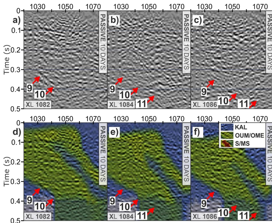
445 Figure 9: Comparison of post-stack migrated sections obtained from the 3D virtual-source survey along crosslines: 1082 (a) and (d), 1084 (b) and (e), 1086 (c) and (f). Red arrows mark the reflection events that are associated with a key contact within the Kylylahti formation (OUM/OME in contact with black schists (KAL)). Note that extent of the geological model shown is constrained by the borehole data, and the marked reflections are at the very edge of this extent. The Kylylahti formation continues beyond the shown extent with further repetitions of the OUM/OME units with black schist inter-layers. The arrows with numbers show reflections that are interpreted in the text. The 450 geological model (described in section 2) displayed in the background is color-coded as follows: S/MS mineralisation (red); OUM/OME units (green); KAL unit (blue).
