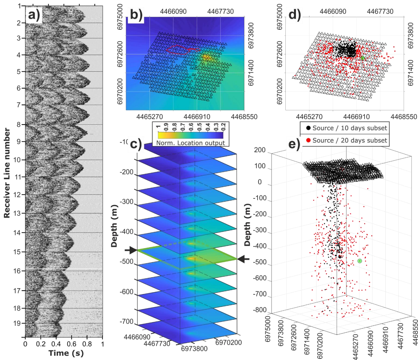
Figure 5: Performance of the combined TWEED and Interloc processing scheme. (a) Scheduled mine event (underground blast) detected with TWEED, and representing the typical body-wave event recorded by the Kylylahti array. Horizontal, black lines mark the spatial extent of 19 receiver lines forming the complete Kylylahti array. (b) Interloc output computed for the body-wave event shown in (a) using a 10-second-long recording detected with TWEED. Color scale represents the normalized amplitude of the Interloc output. Black triangles indicate geophone locations and the red polygon corresponds to the mine location. (c) Interloc output for set of discrete depth intervals. Each result in (c) was normalized using the global maximum from all evaluated depth intervals. The XY-section at -450 m depth exhibiting the clearest focus and highest amplitudes, is highlighted with black arrows, and represents the most probable depth of the event shown in (a) . (d) X-Y and (e) 3D spatial distribution of the collection of sources at depth estimated during the thirty recording days projected on a map with the Kylylahti array (black triangles) and geographical coordinates. Dots represent the locations of the maximum Interloc values of each detected body-wave event. Location of the event shown in (a) is denoted with green circle. Black dots indicate location of events, which were detected inside the subset of 10 days, highlighted in Figures 3 and 4 and used to evaluate the SI selective stacking performance. Red dots show the locations of events from the remaining 20 days.
