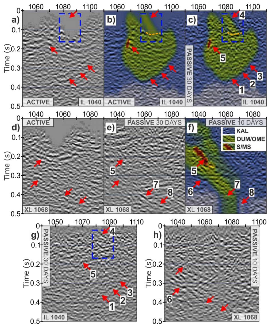
440 Figure 8: Comparison of post-stack migrated sections obtained from the active and passive surveys. Inline 1040 (a)-(c) and (g), and crossline: 1068 (d)-(f) and (h). (a)-(b) and (d) The active-source survey. (c) and (e)-(h) The 3D virtual-source survey. Red arrows mark the reflection events that are associated with the contacts in the geological model and confirmed with the active-source data. The arrows with numbers show reflections that are interpreted in the text. The geological model (described in section 2) displayed in the background is color-coded as follows: S/MS mineralisation (red); OUM/OME units (green); KAL unit (blue). Panels (g)-(h) show the same migrated stacks as in panels 445 (c) and (f), respectively, but without the geological model and with broader spatial extent.
