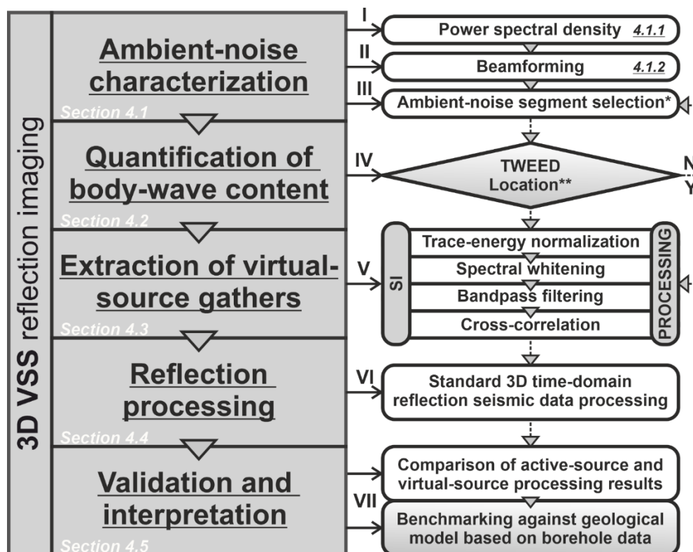
170 Figure 2: Location of the Summary of the 3D virtual-source survey methodology for the purpose of near-mine mineral exploration. The left column presents the core of the flowchart: it contains five main processing blocks representing subsections 4.1–4.5. The detailed processing 175 steps performed within each main processing block are shown in the right column. The sequence of processing is indicated by roman numerals. Gray-gradient-colored blocks in the right column indicate our modifications of the state-of-the-art ambient-noise imaging workflow proposed by Draganov et al. (2013). Single star symbol denotes the user-dependent ‘Ambient-noise segment selection’ processing step, in which the initial selection is based on the beamforming results, and later verified by TWEED. Double star symbol denotes the location procedure, which supports the TWEED verification, but is not mandatory.
