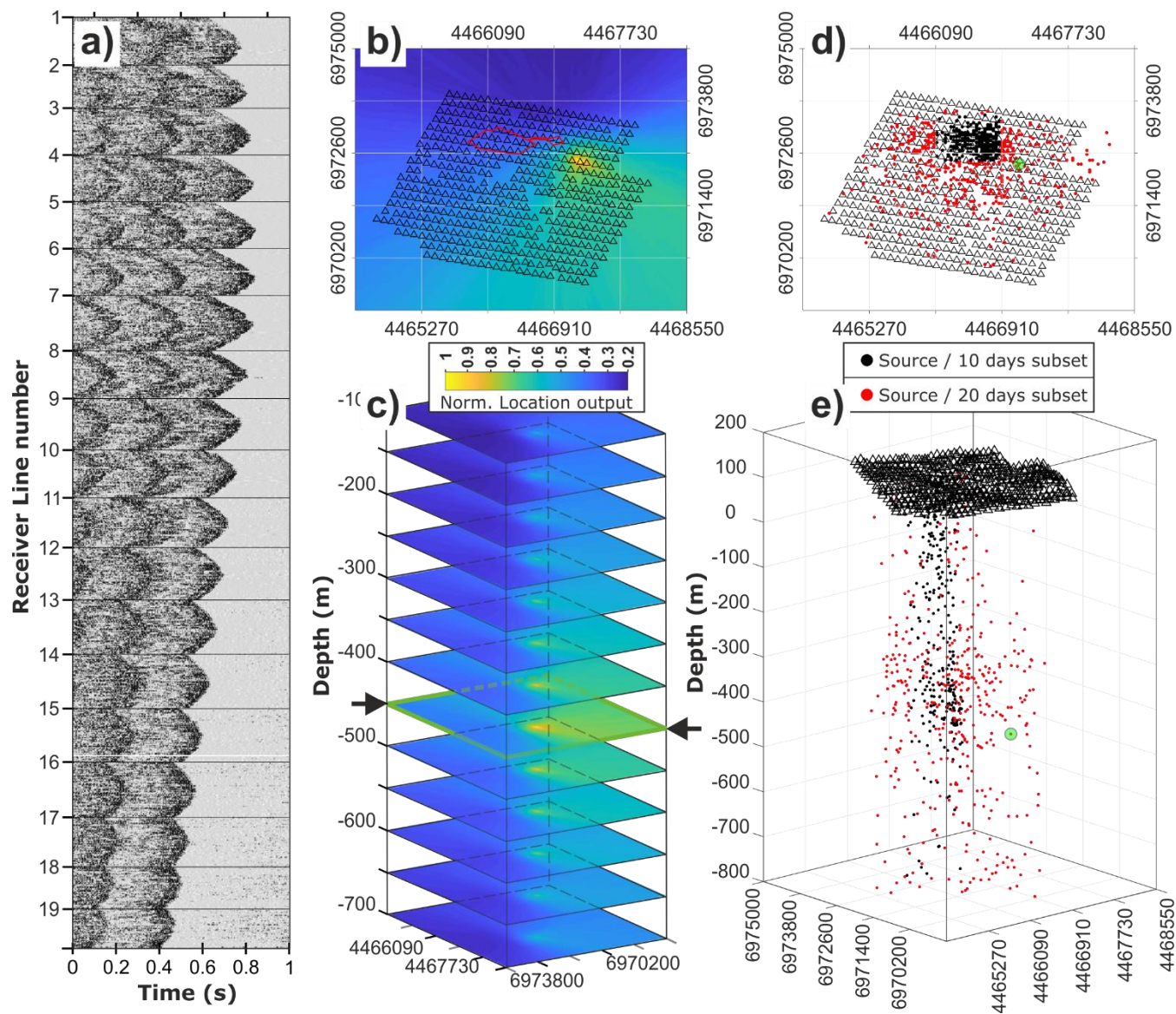
285 Figure 5: Performance of the combined TWEED and Interloc processing scheme. (a) Scheduled mine event (underground blast) detected with TWEED, and representing the typical body-wave event recorded by the Kylylahti array. Horizontal, black lines mark the spatial extent of 19 receiver lines forming the complete Kylylahti array. (b) Interloc output computed for the body-wave event shown in (a) using a 10- second-long recording detected with TWEED. Color scale represents the normalized amplitude of the Interloc output. Black triangles indicate geophone locations and the red polygon corresponds to the mine location. (c) Interloc output for set of discrete depth intervals. Each result in (c) was normalized using the global maximum from all evaluated depth intervals. The XY-section at -450 m depth exhibiting the clearest focus and highest amplitudes, is highlighted with black arrows, and represents the most probable depth of the event shown in (a). (d) X-Y 290 and (e) 3D spatial distribution of the collection of sources at depth estimated during the thirty recording days projected on a map with the Kylylahti array (black triangles) and geographical coordinates. Dots represent the locations of the maximum Interloc values of each detected body-wave event. Location of the event shown in (a) is denoted with green circle. Black dots indicate location of events, which were detected inside the subset of 10 days, highlighted in Figures 3 and 4 and used to evaluate the SI selective stacking performance. Red dots show the locations of events from the remaining 20 days.
