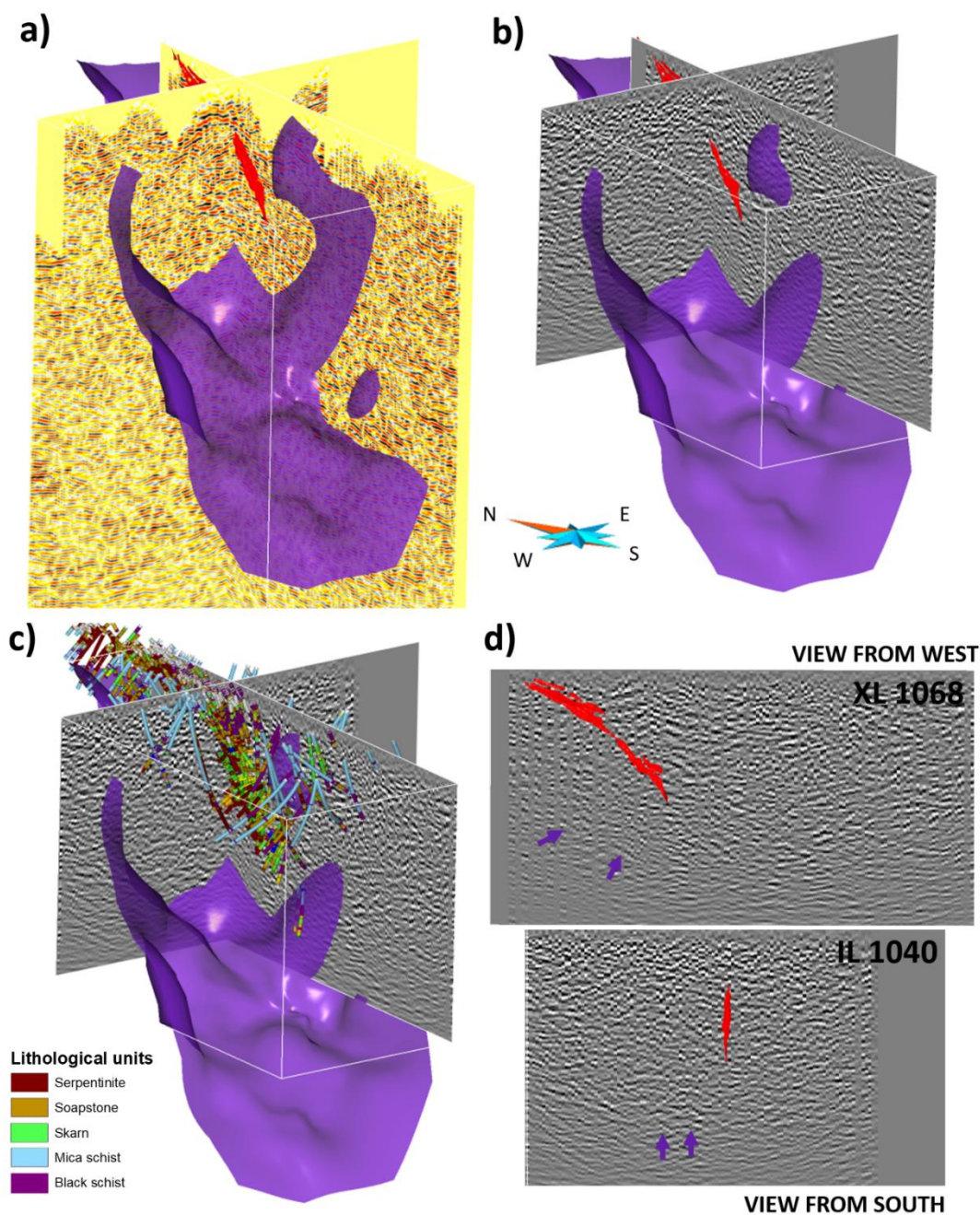
465 Figure 10: (a) The Kylylahti active-source 3D data processed with a similar 3D reflection seismic processing workflow as the passive 3D 10-day subset data shown on (b), and overlapping the crossline 1068 and inline 1040 of the passive 3D cube of figure (b). The purple surface is the base of the Kylylahti formation interpreted from the COGITO-MIN 2D and 3D active-source data and the available borehole data (c). The red surface is the Kylylahti semi-massive to massive sulphide mineralization. (d) Reflection signals associated with the base of the Kylylahti formation on the crossline 1068 and inline 1040 of the passive 3D cube highlighted with purple arrows.
