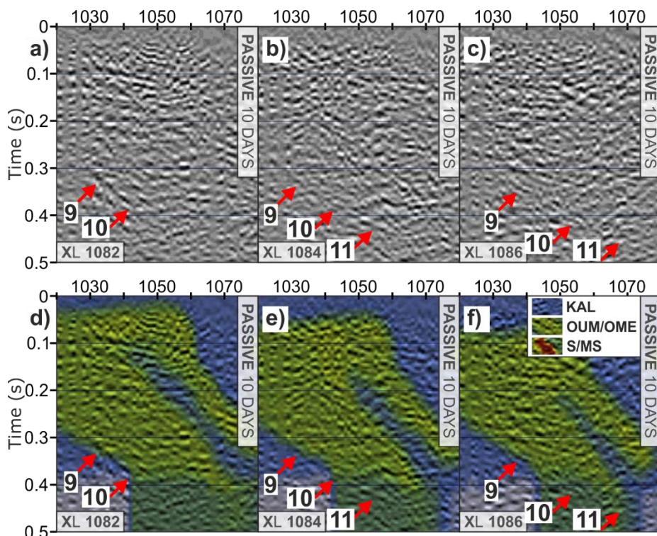
Figure 9: Comparison of post-stack migrated sections obtained from the 3D virtual-source survey along crosslines: 1082 (a) and (d), 1084 (b) and (e), 1086 (c) and (f). Red arrows mark the reflection events that are associated with a key contact within the Kylylahti formation (OUM/OME in contact with black schists (KAL)). Note that extent of the geological model shown is constrained by the borehole data, and the marked reflections are at the very edge of this extent. The Kylylahti formation continues beyond the shown extent with further repetitions of the OUM/OME units with black schist inter-layers. The arrows with numbers show reflections that are interpreted in the text. The geological model (described in section 2) displayed in the background is color-coded as follows: S/MS mineralisation (red); OUM/OME units (green); KAL unit (blue).
