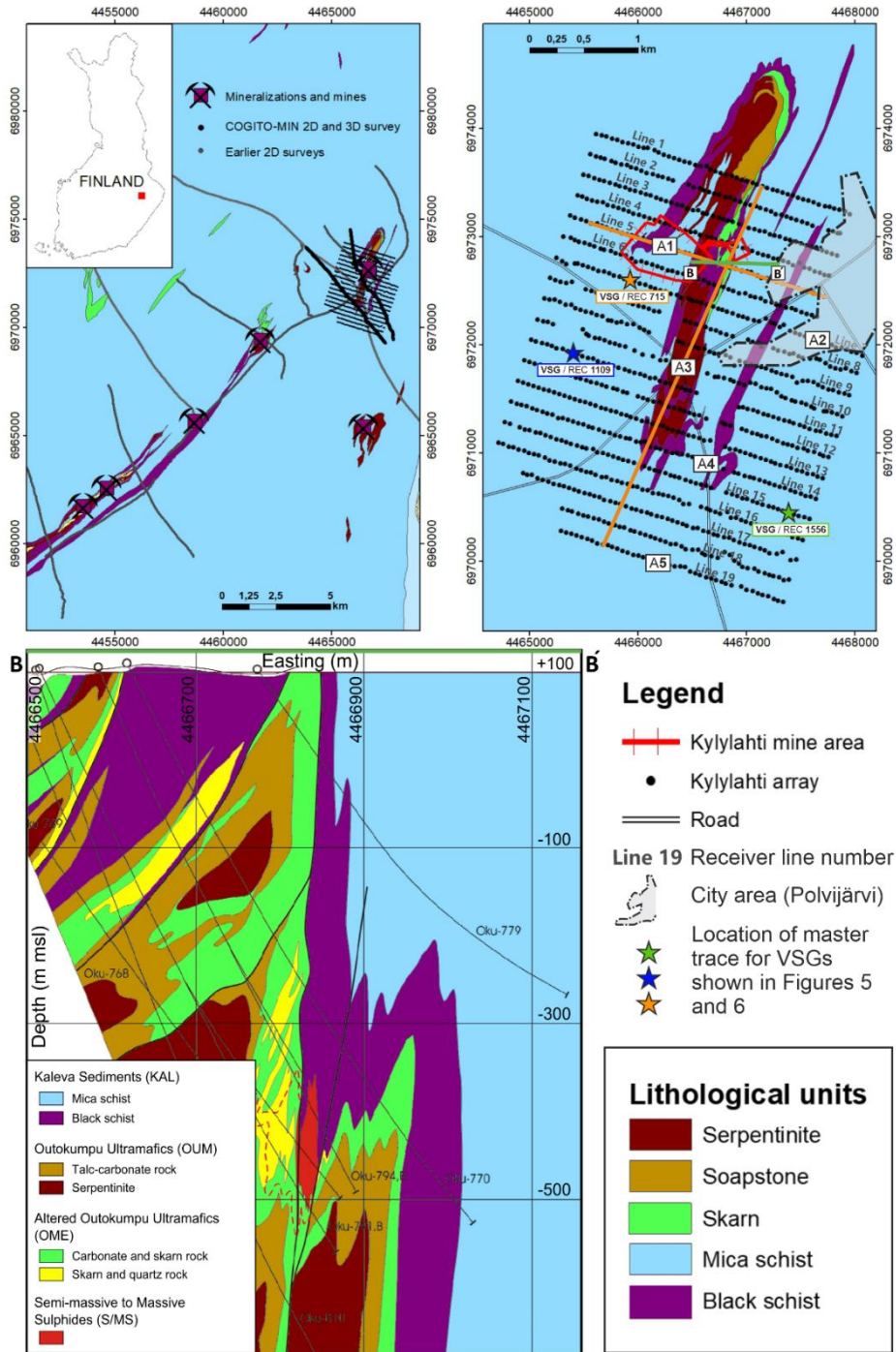
100 Figure 1: Location of the Kylylahti mine and Kylylahti array in the Outokumpu belt (top left panel). Location of the 3D passive seismic survey (top right panel). B-B' is a cross-section through the Kylylahti deposit (bottom left panel; modified after Peltonen et al. (2008) and Riedel et al. (2018)). Orange lines mark a representative crossline and inline location of the 3D passive seismic volume. A1-A5 denote five representative areas of ambient noise in the Kylylahti area that are used to compute power spectral density (PSD) in Figure 3a: the mine (A1), a city (A2), a roundabout (A3), a road (A4), and a quiet area (A5).
