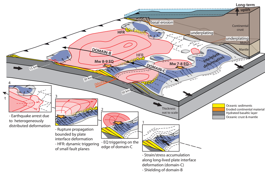
Figure 7. 3D view onto the subduction plate interface depicting the mutual spatial relationships between earthquake ruptures ( in red ) and longer-lived deformation determined from the CTT analysis (blue patches) . Stages 1-4 illustrate how this deformation controls the triggering and limits seismic ruptures. See text for further discussion.
