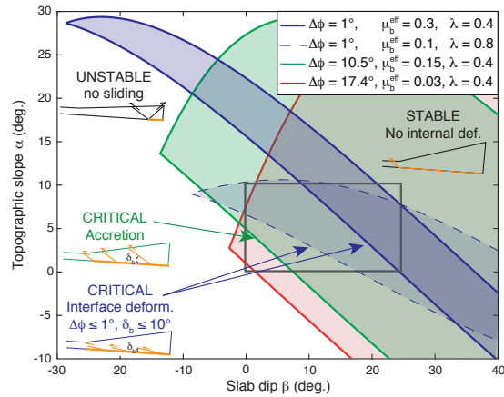
Figure 2. (a) Critical taper theory with different mechanical states. The grey rectangle represents the standard range of topographic slope \alpha and slab dip \beta of subduction zones. With extremely low effective friction along the megathrust (red curve), the wedge systematically falls in the stable domain. With larger effective friction, and large difference of effective friction between the megathrust and the wedge (green curve), the wedge can reach the accretionary critical state characterized by internal faulting. With a reduced difference (blue curves), a wedge can still reach the critical state but the dip of internal faults within the wedge will decrease and become parallel to the plate interface. High pore fluid pressure facilitates interface deformation for low slab dips (dashed blue curve), whereas lower pore fluid pressure induces interface deformation at larger slab dip (plain blue curve). (b) Topographic slope ( \alpha ) versus slab dip ( \beta ) for a swath profile along the Iquique segment and (c) along the Tocopilla segment (locations on Fig. 1b and Suppl. Mat. fig. 1). Segments at critical state, according to inversion, are shown in blue: light blue when probably erosive, dark blue for probable underplating. Grey: swath plus or minus standard deviation. Properties of each segment are provided in Suppl. Mat. table 1.
