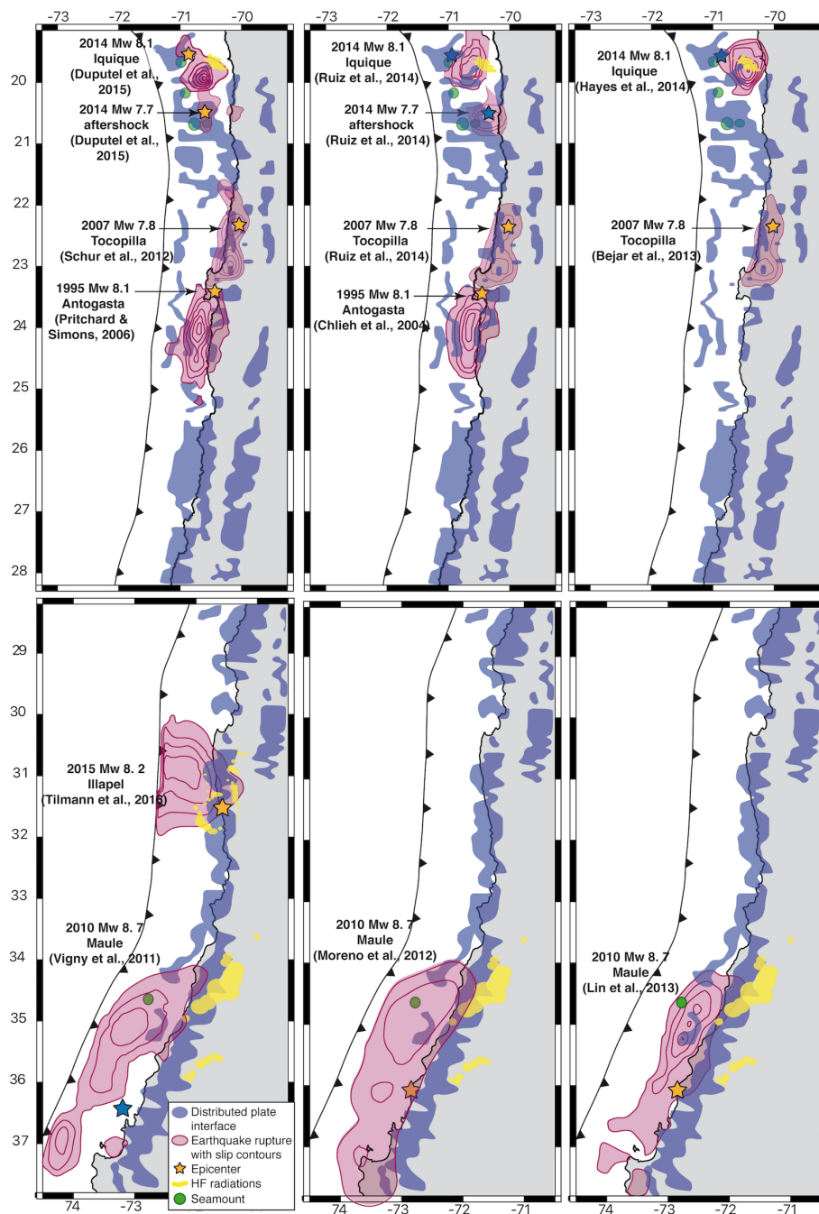
Figure 5. Areas prone to distributed deformation along the plate interface compared to various published co-seismic slip models (Duputel et al., 2015; Schurr et al., 2012; Pritchard and Simons, 2006; Tilmann et al., 2016; Vigny et al., 2011; Ruiz et al., 2014b; Chlieh et al., 2004; Moreno et al., 2010; Hayes et al., 2014; Béjar-Pizarro et al., 2013; Lin et al., 2013). Orange stars: gCMT solution, blue stars: CSN solution.
