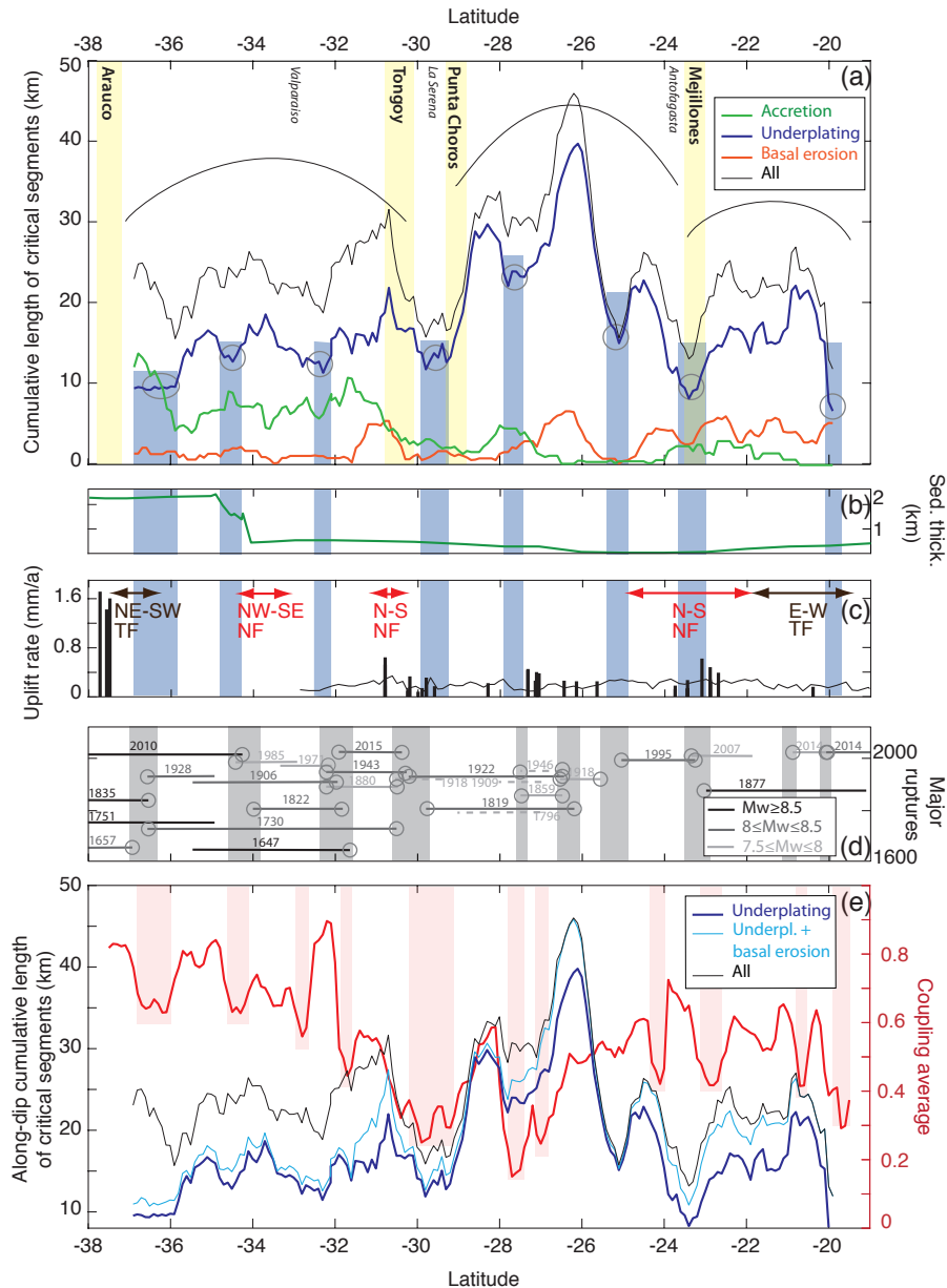
Figure 4. (a) Along-dip cumulative length of segments at accretionary (green), underplating (blue) or basal erosion (orange) critical state (length smoothed by a rectangular window over 8 profiles). Regions with limited underplating length are represented by blue bands. (b) Thickness of sediment income (green, Santibáñez et al., 2018; Tréhu et al., 2019). (c) Quaternary uplift rates of marine terraces (black bars, largest average rate since terrace abandonment, Saillard et al., 2017), coastal uplift rate obtained from a landscape evolution model (black curve, Melnick, 2016) and extent of known active faults (NF: normal fault, TF: thrust fault, Santibáñez et al., 2018). (d) Along-strike extent of historical megathrust ruptures (Saillard et al., 2017). (e) Comparison between the cumulative length of segments at critical state (thin black), with underplating (thick blue), with both underplating and basal erosion (light blue) and the average coupling value along profiles from Metois et al. (2016) corrected by Klein et al. (2018) between 24.5°S and 28°S (plain red curve). Red bands show segments of decreasing coupling. Correlation factor between coupling and underplating: r = -0.36 , between coupling and underplating + basal erosion: r = -0.39 .
