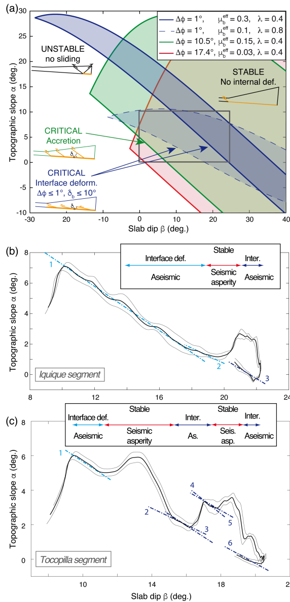
Figure 2. (a) Critical taper theory with different mechanical states. The grey rectangle represents the standard range of topographic slope \alpha and slab dip \beta of subduction zones. With extremely low effective friction along the megathrust (red curve), the wedge systematically falls in the stable domain. With larger effective friction, and large difference of effective friction between the megathrust and the wedge (green curve), the wedge can reach the accretionary critical state characterized by internal faulting. With a reduced difference (blue curves), a wedge can still reach the critical state but the dip of internal faults within the wedge will decrease and become parallel to the plate interface. High pore fluid pressure facilitates interface deformation for low slab dips (dashed blue curve), whereas lower pore fluid pressure induces interface deformation at larger slab dip (plain blue curve). (b) Topographic slope ( \alpha ) versus slab dip ( \beta ) for a swath profile along the Iquique segment and (c) along the Tocopilla segment (locations on Fig. 1b and Suppl. Mat. fig. 1). Segments at critical state, according to inversion, are shown in blue: light blue when probably erosive, dark blue for probable underplating. Grey: swath plus or minus standard deviation. Properties of each segment are provided in Suppl. Mat. table 1.
