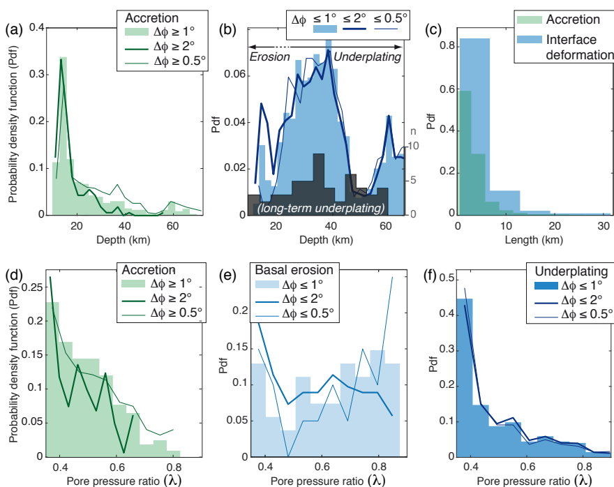
Figure 3. (a) Mean depth of segments at accretionary critical state and (b) distributed plate interface deformation critical state, compared to a compilation of the maximum burial depth reached by exhumed tectonic slicing (grey, Agard et al., 2018) (c) Length of segments at accretionary and distributed plate interface deformation critical state. (d), (e) and (f) Pore fluid ratio \lambda of segments at accretionary, basal erosion or underplating critical state. Histograms are shown for a 1^\circ difference of internal and basal effective friction, thin line for a 0.5^\circ difference, bold line for 2^\circ .
