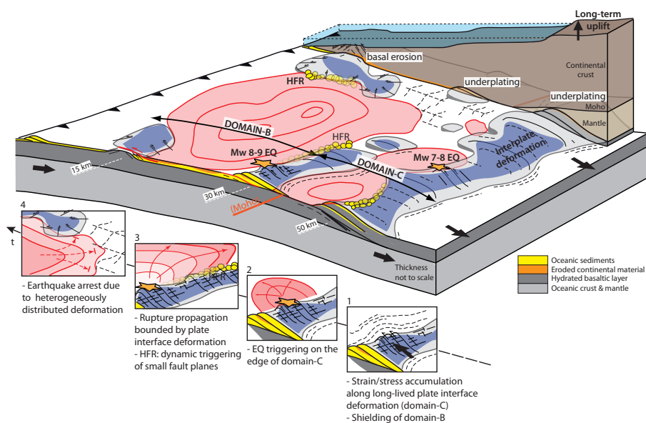
Figure 6. 3D view onto the subduction plate interface depicting the mutual spatial relationships between earthquake ruptures and longer-lived deformation. Stages 1-4 illustrate how this deformation controls the triggering and limits seismic ruptures. See text for further discussion.
