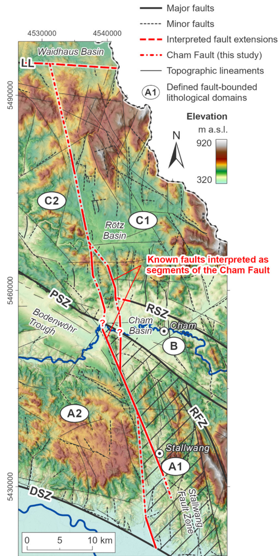
390 Figure 7 Detailed map of the Cham Fault as inferred from the DEM. Several faults known from the geological map are interpreted as segments of the Cham Fault (faults from Teipel et al., 2008 and Galadí-Enríquez et al., 2009b). Note the uncertainty in the location of the southernmost part of the fault, which is due to enhanced erosion along the Stallwang Fault Zone. Fault zones: DSZ Danube Shear Zone, LL Luhe Line, PSZ Pfahl Shear Zone, RSZ Runding Shear Zone, RFZ Rattenberg Fault Zone.
