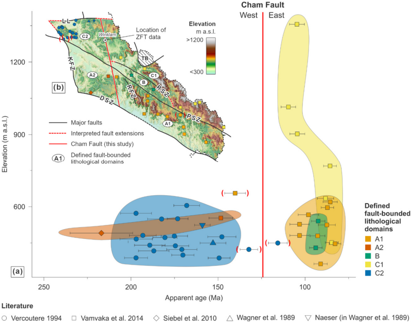
Figure 9 Compilation of published Apatite Fission Track (AFT) data (Wagner et al., 1989; Vercoutere, 1994; Siebel et al., 2010; Vamvaka et al., 2014). (a) Age-elevation plot color-coded according to the sample’s domain affiliation. Note that the Cham Fault separates two distinct clusters of AFT apparent ages. Calculation of the sample altitudes has been done based on a DEM with a 1-meter horizontal resolution using the sample location coordinates. (b) Locations of the samples shown in (a) superimposed on a DEM. Note that the village of Winklarn depicts the sample locations of published ZFT data, with one sample located at each side of the Cham Fault within a 2 km distance (see text for details). Fault zones: DSZ Danube Shear Zone, KFZ Keilberg Fault Zone, LL Luhe Line, PSZ Pfahl Shear Zone, RSZ Runding Shear Zone, RFZ Rattenberg Fault Zone. TB Teplá-Barrandian.
