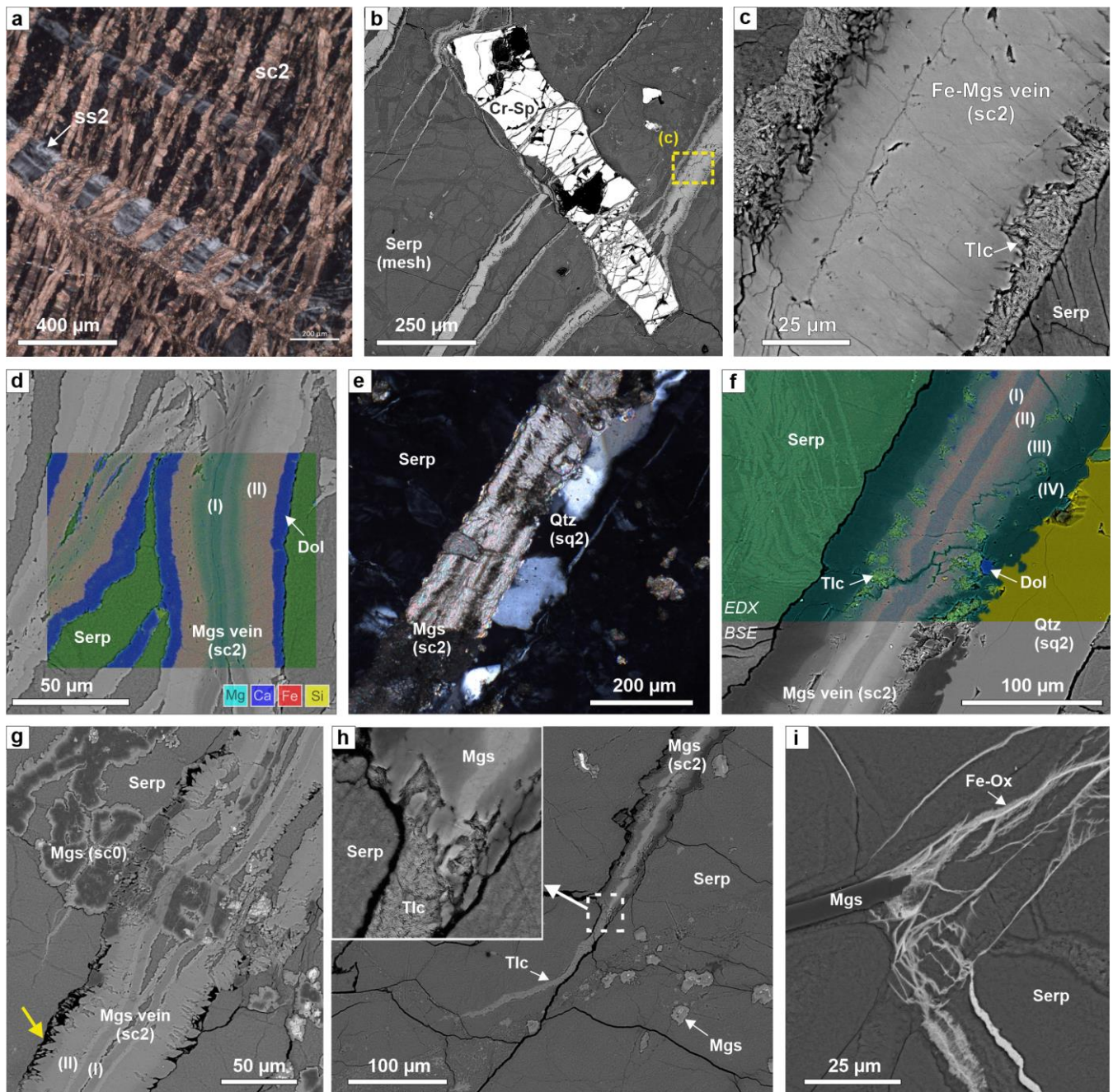
Figure 4: Microstructures of zoned magnesite veins (sc2) in serpentinite. (a) close spacing of carbonate; the veins are deflected where they cut a crack-seal serpentinite vein (xpol). (b) Elongated Cr-spinel and serpentinite mesh cut by zoned, Fe-magnesite-talc veins (BSE image). (c) Detail of b, showing talc seams along vein walls. (d) Composite-color EDX map superposed on a BSE image of zoned sc2 veins with dolomite rims (I: Ca-bearing magnesite; II: Fe-magnesite); phase legend see Fig. 3c. (e) Quartz vein exploiting the vein-host interface of a zoned magnesite vein (xpol). (f) Composite-color EDS map superposed on a BSE image of a part of the vein in e, with zones: (I) Ca-bearing magnesite, (II) Fe-magnesite, (III) Fe-bearing magnesite with talc inclusions, (IV) Fe-poor magnesite. Small Mg/Si variations show thin serpentine veins in the matrix. (g) Complex cross-cutting relations between zoned sc2 vein and earlier mesh-pseudomorphous magnesite (sc0), showing that the core of sc2 veins formed by opening while the vein rims are micro-reaction fronts, with euhedral crystal terminations at the vein walls (yellow arrow). (h) Tip of zoned sc2 carbonate vein in serpentinite. At the termination of magnesite, a talc veinlet continues over a short distance. This talc veinlet does not correspond to the open micro-cracks in serpentinite (black lines), showing that those are later and not related to vein formation of the zoned magnesite vein. (h) Fe-oxides/hydroxides veinlets emanating from magnesite vein tip. (a, d, g: BT1B_44-2_47-50; b, c, e, g, h: BT1B_44-3_9-11; i: BT1B_39-3_9-13)
