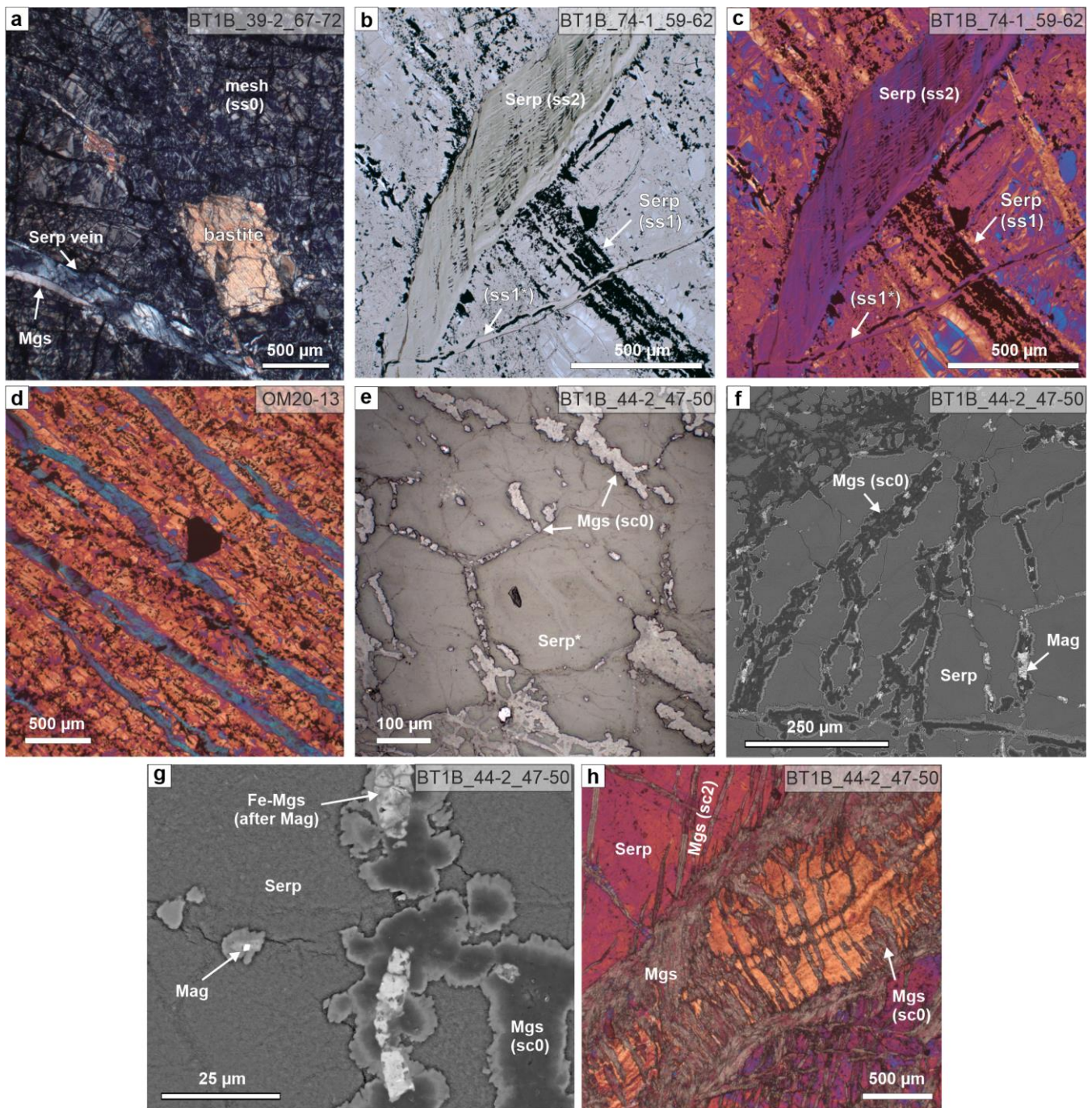
Figure 2: Serpentine veins (a - d), and pseudomorphous carbonate microstructures after serpentine textures (e & f) in serpentinite. (a) Mesh (ss0) and bastite textured serpentinite, cut by serpentine vein; a magnesite vein exploits the vein-host rock interface of the serpentine vein under crossed polarizers (xpol). (b) Plane-polarized (ppol) micrograph of wide serpentine-magnetite vein (ss1) cut by a light-green, banded serpentine crack-seal vein (ss2), which is in turn cut by a narrow serpentine-magnetite vein (ss1*). (c) Same area as in b, with xpol and 1λ-plate. (d) Clustered cleavage-parallel serpentine veins in foliated serpentinite north of site BT1 with strong crystallographic preferred orientation and flattened magnetite mesh cells. The large black grain is Cr-spinel. (xpol with 1λ-plate). (e) Reflected light image and (f) BSE image of magnesite vein network (sc0) tracing polygonal serpentine mesh (Serp*) delineated by former magnetite in serpentinite. (g) Detailed BSE image of sc0 magnesite showing pseudomorphic replacement of magnetite by Fe-magnesite (similar replacements are known from listvenites elsewhere; Menzel et al., 2018), and compositional zoning with Fe-bearing euhedral to dendritic magnesite rims. (h) Serpentine crack-seal vein (orange) in serpentinite, with partial pseudomorphic replacement by magnesite and crosscut by zoned magnesite-dolomite veins (sc2) (xpol with 1λ-plate). For abbreviations of minerals and vein generations used in all figures, see Tables 1 & 2.
