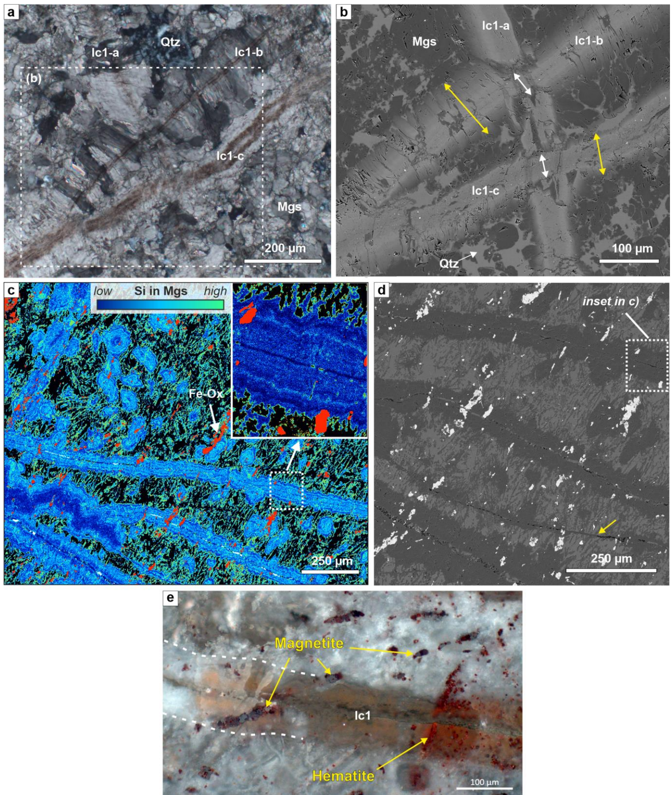
Figure 8: Microstructures showing the extent of opening versus host rock replacement by zoned magnesite veins. (a) Different generations of zoned magnesite veins with brown, Fe-enriched median zone, showing fibrous (lc1-a, lc1-b) and wide-blocky (lc1-c) habits (xpol). (b) BSE image of the area marked in a), showing that the true vein aperture via opening at the intersection with the earlier vein lc1-a corresponds to inclusion-bearing median zones only (white arrows), while fibrous to euhedral overgrowths indicate that a significant fraction of the total vein thickness (yellow arrows) must have formed due to replacement of the host rock (BT1B_14-1_7-11). (c) Si content in magnesite from EDX mapping (with Fe-oxides in red; quartz - black; minor dolomite - white), showing vein-parallel zoning in carbonate veins and concentric zoning in matrix magnesite ellipsoids. Only the median zone of veins cut the oblique Fe-oxides. Local folding of an Si-poor vein core in the lower left. (b) BSE image of part of the area in c); the yellow arrow marks a thin vein that did not develop the common replacement rim. (e) Crossed-polarized, reflected light image of relationship between wide-blocky zoned magnesite vein (lc1), magnetite and hematite. (c, d & e: BT1B_21-3_35-40).
