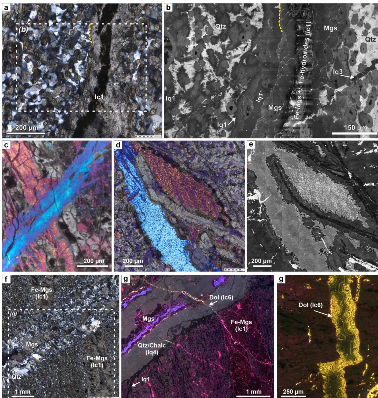
Figure 9: Quartz and late dolomite veins in listvenite. (a) Crossed polarized micrograph of cryptic quartz vein adjacent to a zoned magnesite vein (lc1). (b) SEM-CL image of the marked area in a, showing two generations of dark luminescent cryptic quartz veins (lq1 and lq1*) in bright luminescent matrix quartz and exploiting the zoned magnesite vein interface. Cryptic quartz veins do not cut magnesite ellipsoids in the matrix. A later quartz vein (lq3) cuts both magnesite ellipsoids and the zoned magnesite vein. (c) Two crosscutting generations of micro-crystalline quartz veins with distinct crystal preferred orientations (xpol with 1λ-plate). (d & e) Crosscutting relationship between zoned magnesite veins and micro-crystalline quartz (d: ViP xpol with 1λ-plate; e: SEM-CL); dendritic magnesite overgrowths on the carbonate vein are undisturbed by the micro-crystalline quartz. (f & g) Crossed polarized micrograph and optical CL mosaic image of a quartz/chalcedony-magnesite vein (lq4) cutting a zoned magnesite vein. Magnesite in the vein has distinct luminescence from that in the listvenite matrix. A late, thin dolomite vein cuts all other vein generations. (g) Optical CL mosaic image of a late syntaxial lc6 dolomite vein in listvenite, showing dull to bright yellow oscillatory growth zoning into an open fracture. The vein is roughly oriented vertical (parallel with respect to the core orientation). (a, b, f, g: sample BT1B_14-3_77-80, see marked areas in Fig. 7 a; c: BT1B_56-4_45-50; e, f: BT1B_67-2_36-40; g: BT1B_32-1_17-19).
