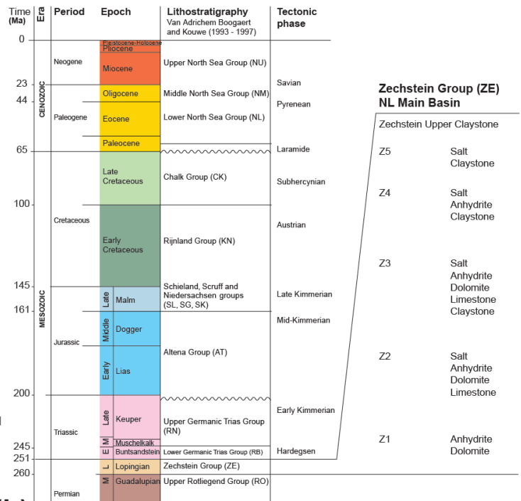
Figure 2. (a) Study area in the NE of the Netherlands and 3D seismic coverage. 3D block Groningen used for quality control. Lines X-X' and Y-Y' shown in Figure 3. BE = Belgium; GER = Germany; NL = The Netherlands. (b) Stratigraphy of the study area (after Van Adrichem Boogaert and Kouwe, 1993). Detailed lithostratigraphic subdivision of the Zechstein Group on the right. Stratigraphic abbreviations used on following figures.
