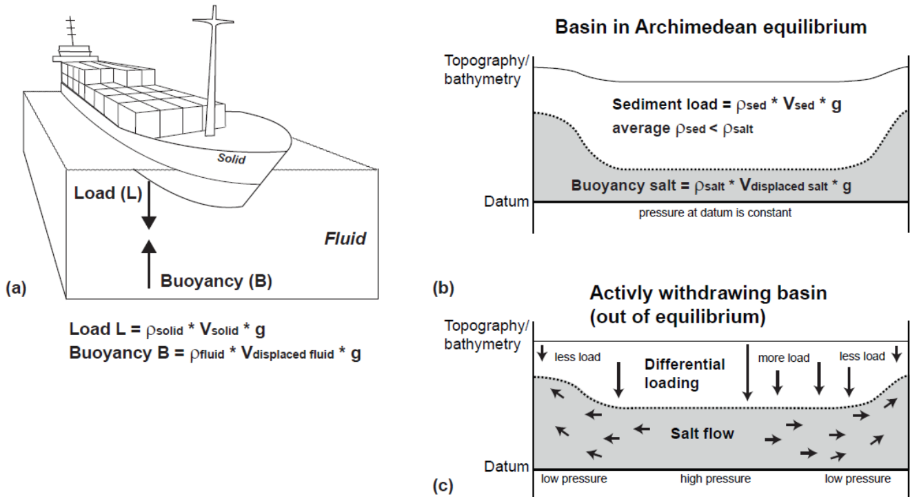
30 Figure 1. Archimedes' principle. (a) Ship loaded and unloaded floating on water. Buoyancy as upward force exerted by the fluid (water) that opposes the weight of the partially immersed ship. (b) Basin above subsurface evaporites in Archimedean equilibrium. Salt treated as dense pseudo-fluid (= 2.2 g/cm 3 ) loaded by cumulatively lighter overburden rocks (solid). Backstripping corresponds to incremental unloading of the overburden (sensu Maystrenko et al. 2013). Archimedean restoration of the Zechstein Basin example justified by slow subsurface salt flow. c) Basin out of equilibrium by major differential loading with significant salt flow and high differential pressure at datum level.
