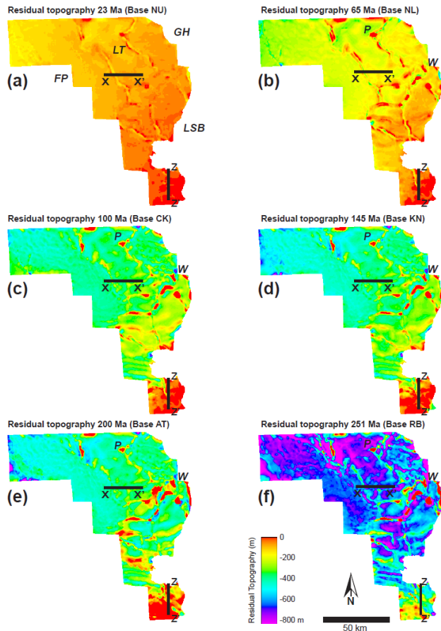
255 Figure 10. Residual 3D topography after each reconstruction step in scenario 2 (unloading and decompaction; submarine conditions). Depth position of respective model top at (a) 23Ma; (b) 65Ma; (c) 100Ma; (d) 145Ma; (e) 200Ma; and (f) 251 Ma. Note that residual topography does not represent palaeo-bathymetry. Incremental backstripping results in increasingly flat basin-floor topographies away from salt diapirs and ridges. Note piercement salt diapirs Pieterburen (P) and Winschoten (W) that remain unbalanced throughout restoration. For balanced sections X-X' and Z-Z' see Figure 5.
