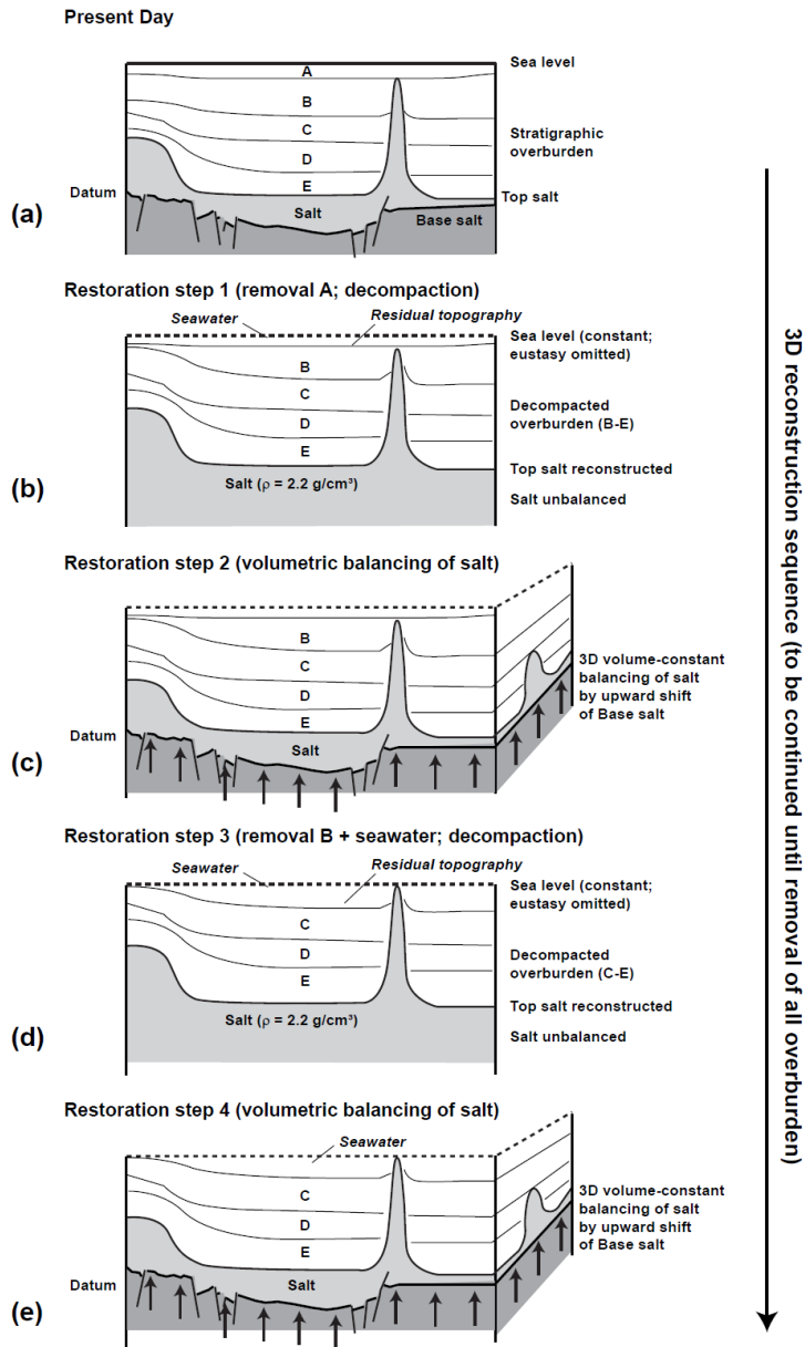
120 Figure 4. Restoration methodology. (a) Present-day situation. (b) Restoration step 1: Removal of top layer A. Airy-type vertical unloading of sedimentary column down to Top salt. Decompaction of sedimentary column down to Top salt (only restoration scenarios 2 and 3). Salt unit remains unbalanced. Residual topography flooded with seawater. (c) Restoration step 2: Upward vertical shift of unbalanced Base salt into new position constrained by keeping salt volume constant. (d) Same as restoration step 1 but removal of new top layer B. (e) Same as restoration step 2 with remaining stratigraphy. Entire 3D unloading procedure to be continued until removal of all salt overburden (Fig. 5).
