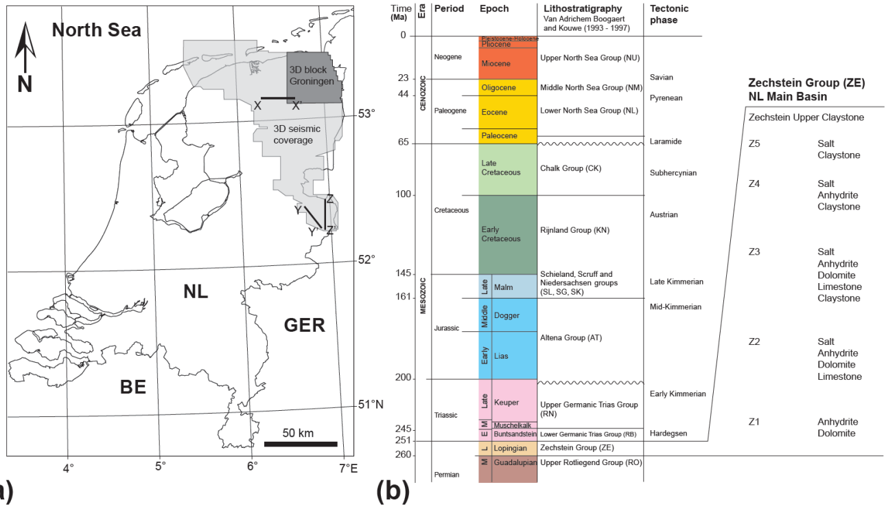
Figure 2. (a) Study area in the NE of the Netherlands and 3D seismic coverage. 3D block Groningen used for quality control. Lines X-X' and Y-Y' shown in Figure 3. BE = Belgium; GER = Germany; NL = The Netherlands. (b) Stratigraphy of the study area (after Van Adrichem Boogaert and Kouwe, 1993). Detailed lithostratigraphic subdivision of the Zechstein Group on the right. Stratigraphic abbreviations used on following figures.
