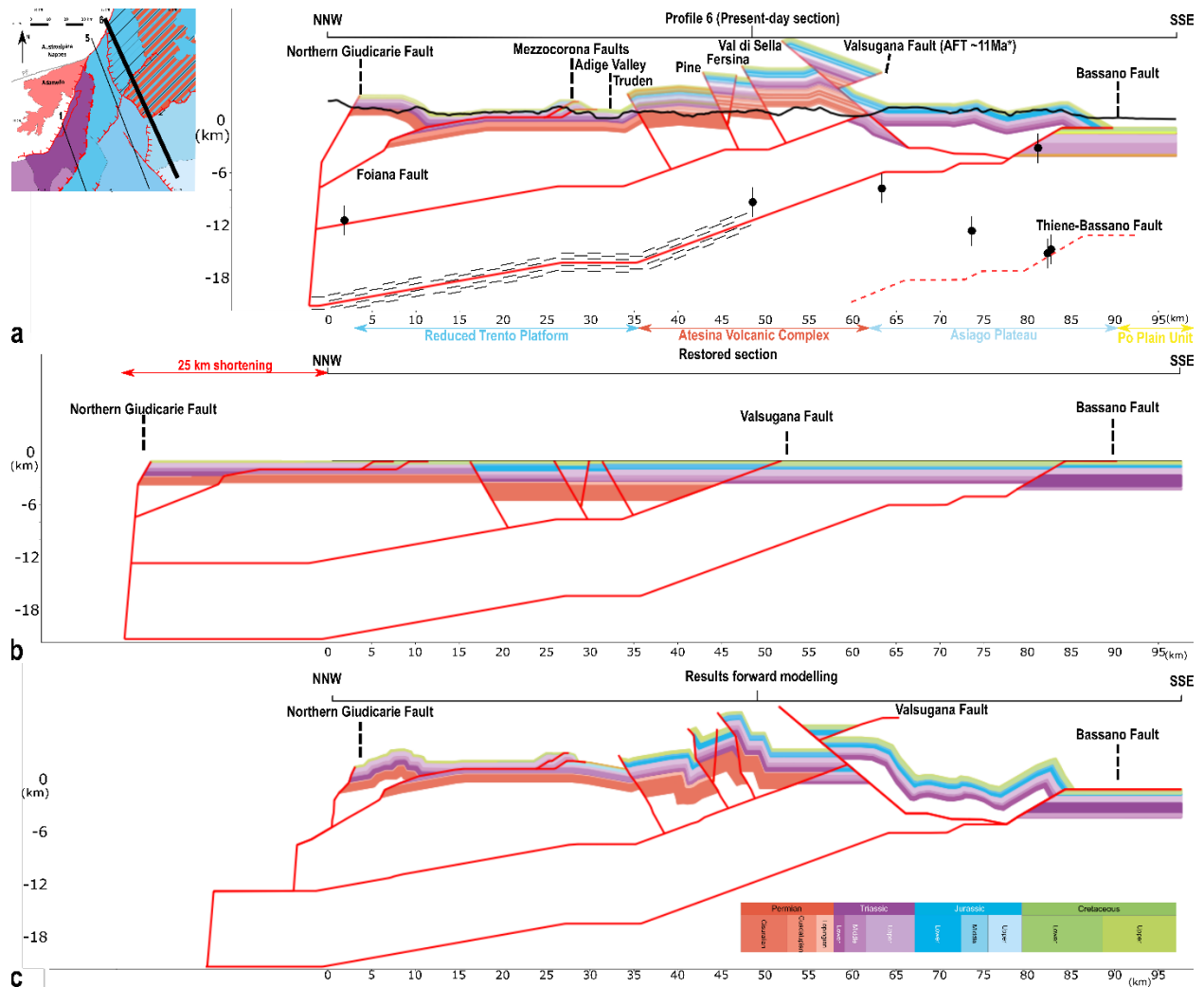
Figure 9: (a) Profile 6 across the Reduced Trento Platform, Atesina Volcanic Complex and the Asiago Plateau (AFT age for Valsugana Fault from Heberer et al. 2016; (b) Profile 6 retro-deformed to a layer-cake stratigraphy; (c) Results of forward modelling. Colors in legend modified after the International Chronostratigraphic Chart with pre-Permian basement beneath in white. Black dots indicate hypocenters of seismic events during 2017-2018 (SWATH-D Network; Jozi Najafabadi et al., 2020; vertical bars indicate the average error range on hypocenter depths), projected from a swath extending to 6 km on either side of the profile. Dashed black lines below ~10 km indicate ductile deformation.
