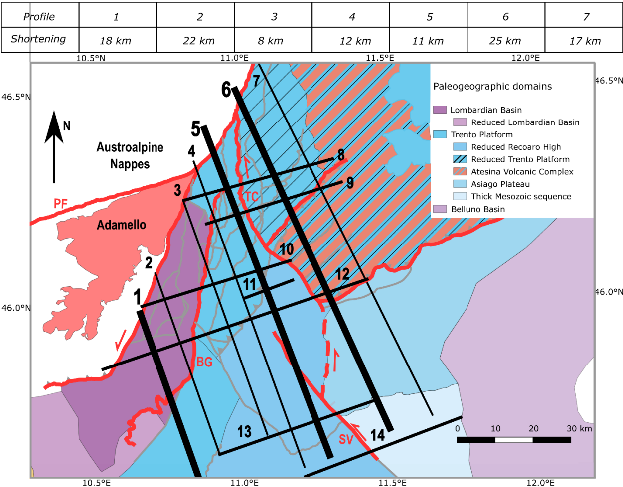
Figure 6: Traces of cross sections constructed and balanced in this study. Details of profile reconstructions for profiles 1, 5 and 6 (thick black lines) is shown on Fig. 7, 8 and 9, respectively. Profiles not shown in Fig. 7, 8, 9 and 10 are available in the supplementary material. Abbr. BG: Ballino-Garda Fault; PF=Periadriatic Fault; SV: Schio-Vicenza Fault; TC: Trento-Cles Fault.
