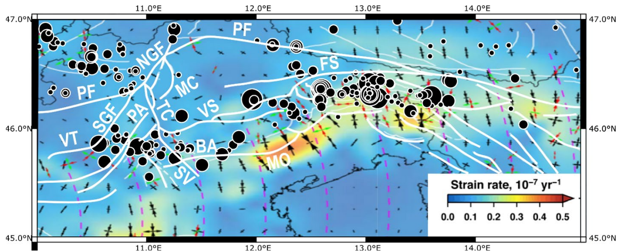
Figure 13: Epicenters of seismic events from 2017-2018 ( M_L \geq 1 ; size of black dots indicates earthquake magnitudes up to M_L 4.2) compiled from the SWATH-D Network (Jozì Najafabadi et al., 2020) superposed on strain rates determined from GPS velocities (after Serpelloni et al., 2016). Note that the area in the center with the highest strain rates (vicinity of the Montello Thrust) coincides with lower seismic activity, although clustering of low-magnitude events has been reported (Moratto et al., 2019; Romano et al., 2019). Abbr.: FS=Fella-Sava Fault; see Fig. 1 for the other fault abbreviations.
