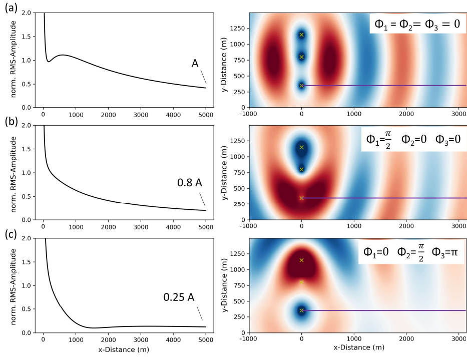
Figure 8: Calculated amplitude decay curves (in direction of the magenta line) for three scenarios with different source signal phase compositions using (a) \Phi_1 = \Phi_2 = \Phi_3 = 0 (vibration in phase), (b) \Phi_1 = \pi/2 , \Phi_2 = 0 , \Phi_3 = 0 and (c) \Phi_1 = 0 , \Phi_2 = \pi/2 , \Phi_3 = \pi . Index 1 represents the source point S1. All decay curves are normalized to the amplitude at x = 300 m.
