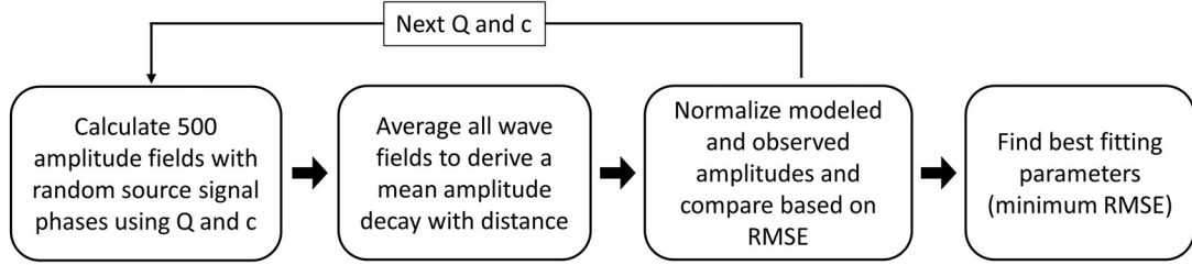
Figure 9: Description of the fitting process to find best model parameters from the comparison of calculated and observed amplitudes.
