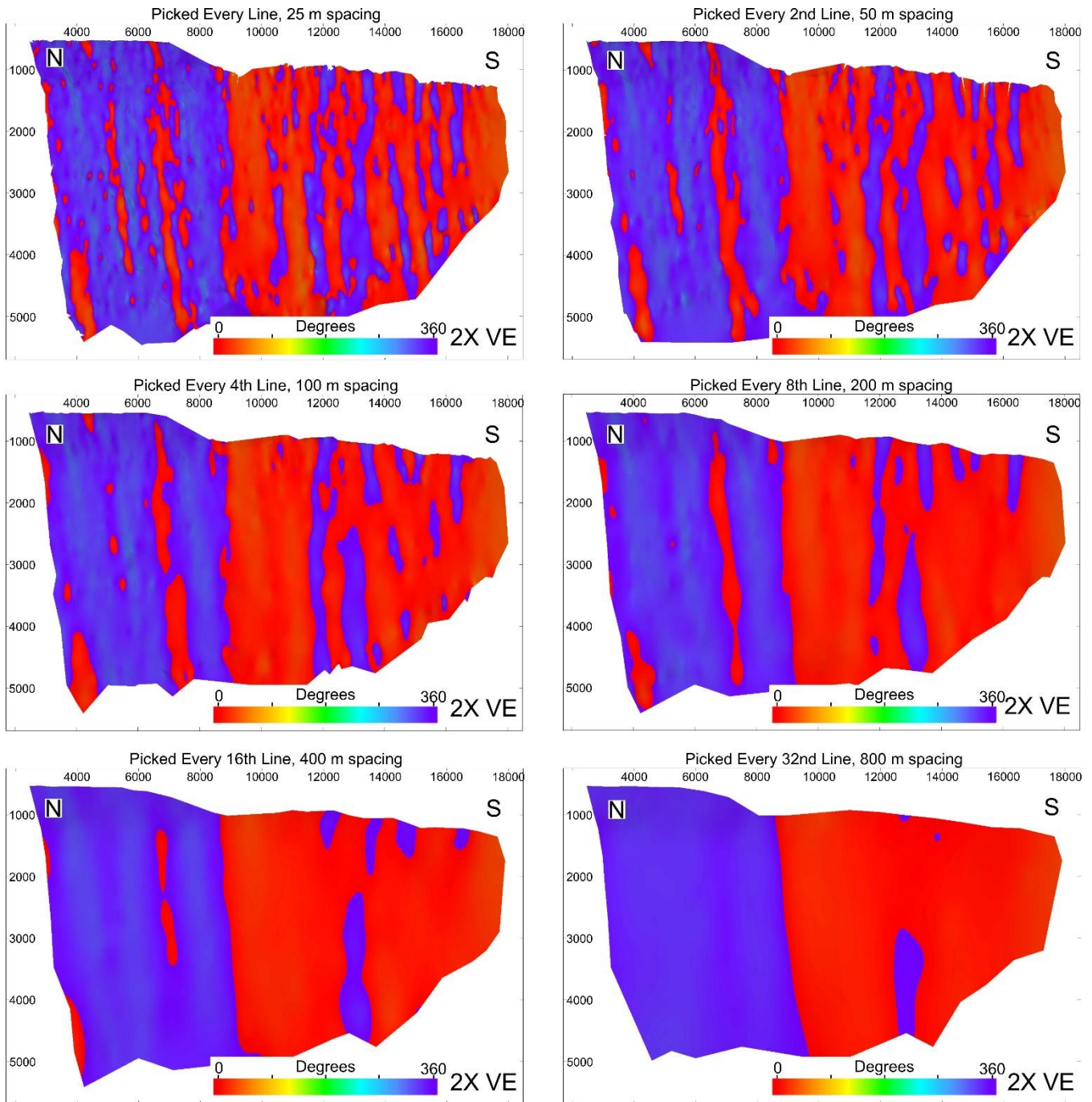
Figure 9. Fault plane diagrams showing fault strike attribute displayed on the fault surfaces for each picking strategy: 25 m, 50 m, 100 m, 200 m, 400 m and 800 m line spacing 1, 2, 4, 8, 16 and 32 lines. Fault strike is observed to vary with line spacing used for fault picking. A highly irregular fault surface is observed when every line is used for picking, when compared to the overly smooth surface
