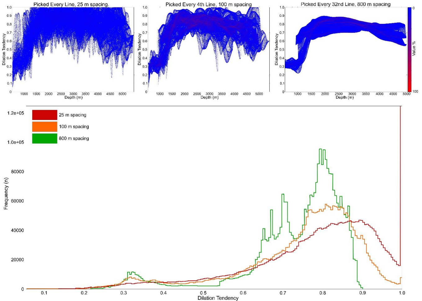
Figure 14. A-C: plots showing dilation tendency with depth, for scenarios with a line spacing of 25 m picked on every line (A), 100 m every 4 th line (B) and 800 m every 32 nd line (C). Colour intensity reflects the frequency of those values, where blue is 1% and red is 100% frequency. D: Histogram showing frequency of dilation tendency for scenarios picked with a line spacing of 25 m on every line (red), 100 m every 4 th lines (orange) and 800 m every 32 nd line (green). Note that when every line is picked, a large portion of the values are above 1 (i.e. in failure). This decreases as the spacing decreases.
