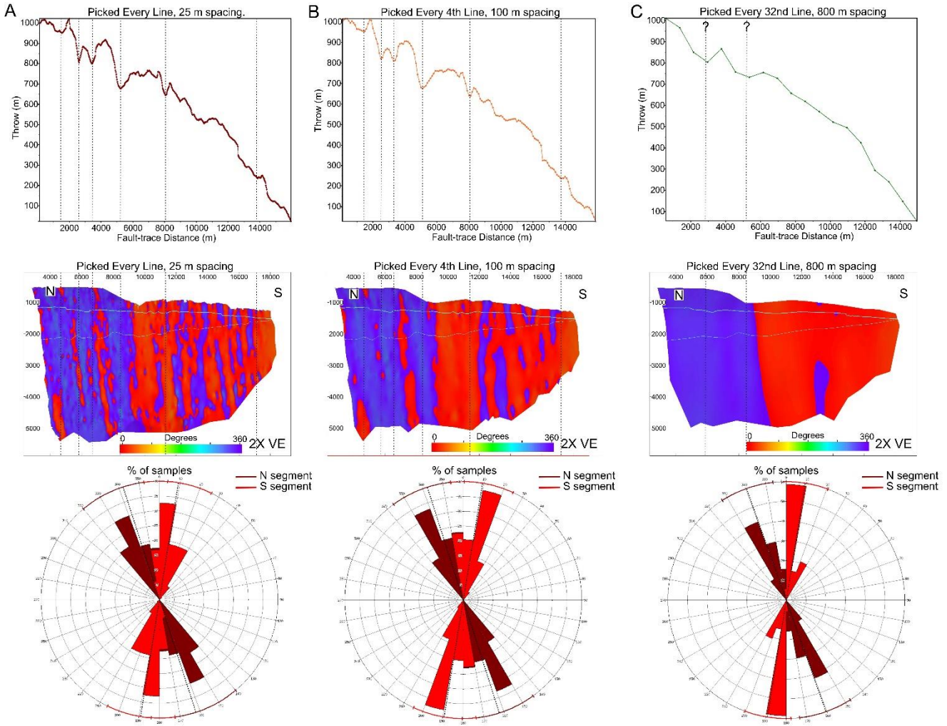
Figure 10. TD plots, fault plane diagrams showing strike, and rose diagrams for scenarios picked on a line spacing of 25 mevery line (A), 100 mevery 4 th lines (B) and 800 mevery 32 nd line (C). Areas where fault segmentation has been picked using the TD plots have been extrapolated onto the fault plane diagrams in order to assess whether areas of strike irregularities are fault corrugations highlighting areas of segmentation. Blue lines on fault plane diagrams shows level of the top Sognefjord as HW- (thicker lines) and FW- (thinner lines) cutoffs. Rose diagrams illustrating the orientation and range of orientation for each scenario. Note that unconstrained triangulation is used for fault surface generation.
