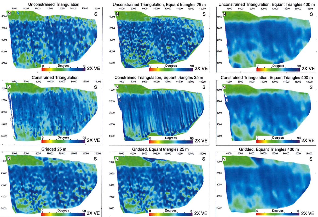
975 Figure 16. Fault plane diagrams created using different triangulation methods for the picking strategy where every line has been interpreted, showing dip attribute. Unconstrained, constrained and gridded triangulation methods have been used, with irregular triangles and equant triangles of different sizes. We can see that vastly different surfaces are created using different techniques, leading to differences in the dip attribute.
