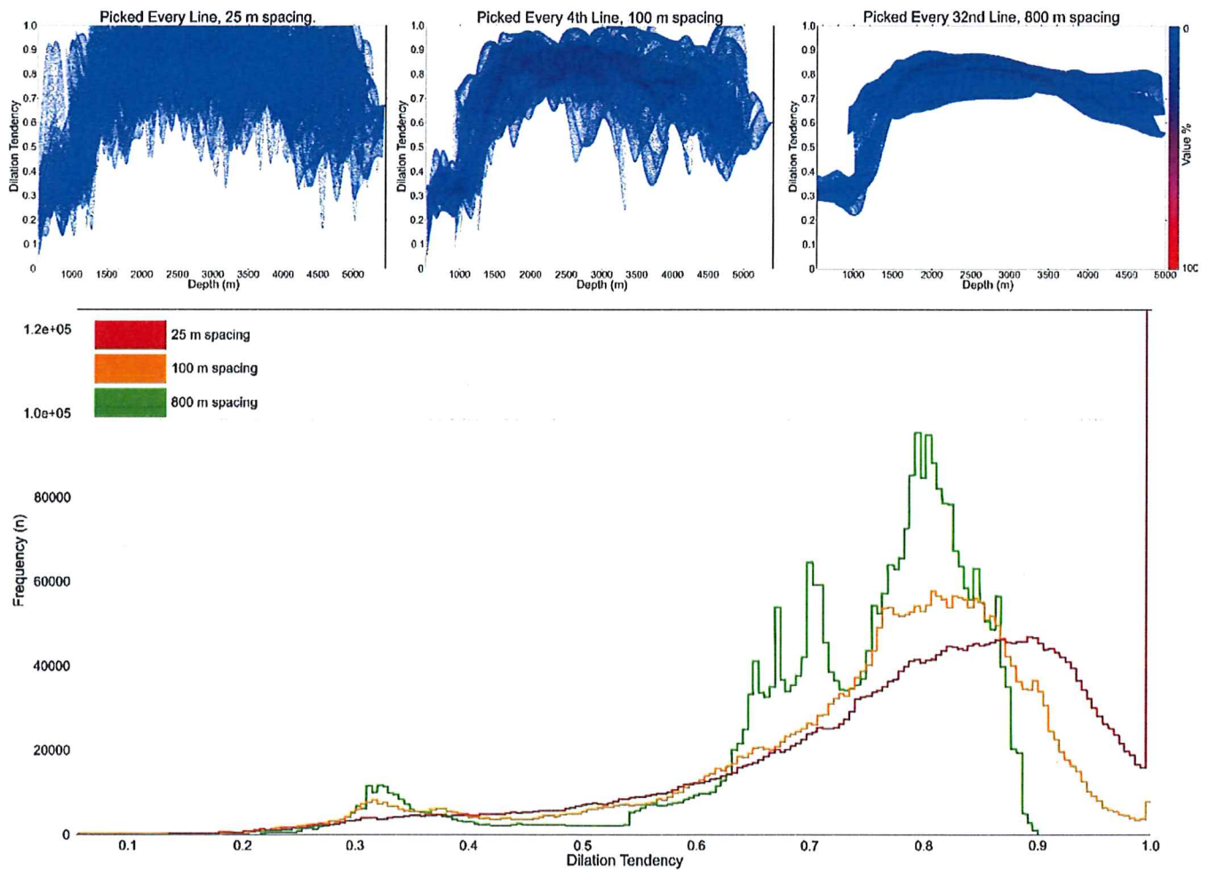
955 Figure 13. A-C: plots showing dilation tendency with depth, for scenarios picked on every line (A), every 4 th line (B) and every 32 nd line (C). Colour intensity reflects the frequency of those values, where blue is 1% and red is 100% frequency. D: Histogram showing frequency of dilation tendency for scenarios picked on every line (red), every 4 th lines (orange) and every 32 nd line (green). Note that when every line is picked, a large portion of the values are above 1 (i.e. in failure). This decreases as the spacing decreases.
