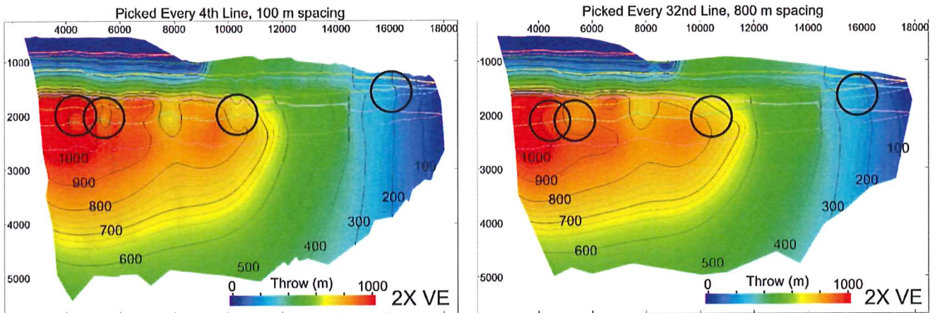
905 Figure 7. Top: Fault throw-distance profile for the Vette fault picked on every 4 th and 32 nd line. The x-axis has been normalized for distance along fault-trace (Length/Length max), in order to directly compare the two scenarios. Bottom: Contoured fault throw plots displaced on a fault surface picked on every 4 th line (left) and 32 nd line (right). Circles highlighted in the throw-distance graph correspond to the same circles highlighted on the fault throw plots. We can observe the four fault segments that are not recorded when a picking strategy of 32 nd line spacing is used. These fault segments are recorded in the throw profile when a narrower spacing 910 strategy is used, but are smoothed out and lost when a wider spacing strategy is used. Note that unconstrained triangulation is used for fault surface generation.
