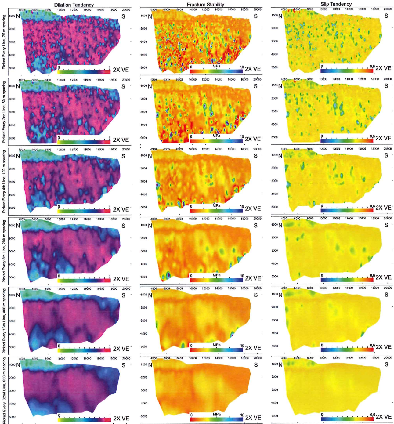
Figure 12. Fault plane diagrams showing the fault reactivation potential, specifically dilation tendency, fracture stability and slip tendency, for each picking strategy: 1, 2, 4, 8, 16 and 32. Different conclusions regarding fault stability occurs due to differing picking strategies. When using narrow spaced lines for fault picking, the fault shows a lesser likelihood of failing by either tensile
