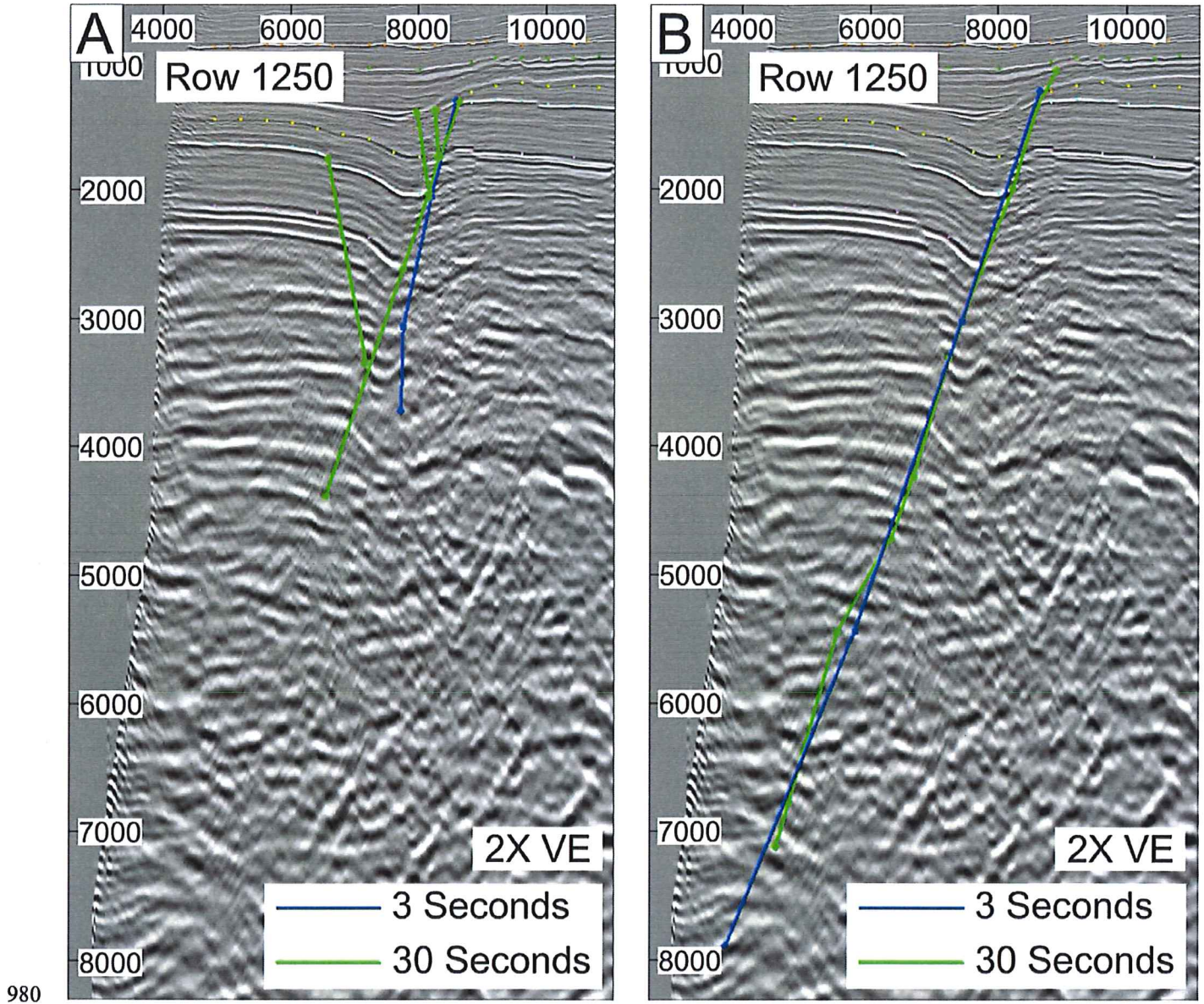
Figure 17. Differences in fault picking with different time constraints (3 seconds versus 30 seconds), shown by two separate interpreters (A and B), picked on the same row (row 1250).
