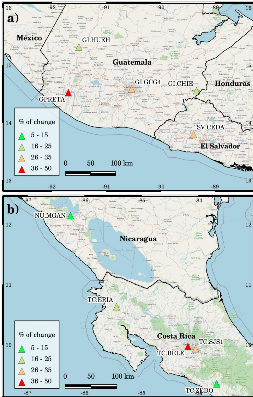
640 641 Figure 6. Percent of change of the high-frequency seismic anthropogenic noise displacement (HFSAND-RMS) 642 in the band 4-14Hz during the period from January 15 to March 15, 2020 (before lockdown measures) with respect 643 to the time interval from March 16 to May 15, 2020 (after the lockdown measures were applied). a) Percent of 644 change in seismic stations of Guatemala and El Salvador. b) Percent of change in seismic stations of Nicaragua 645 and Costa Rica. © OpenStreetMap contributors 2020. Distributed under the Open Data Commons Open Database 646 License (ODbL) v1.0.
