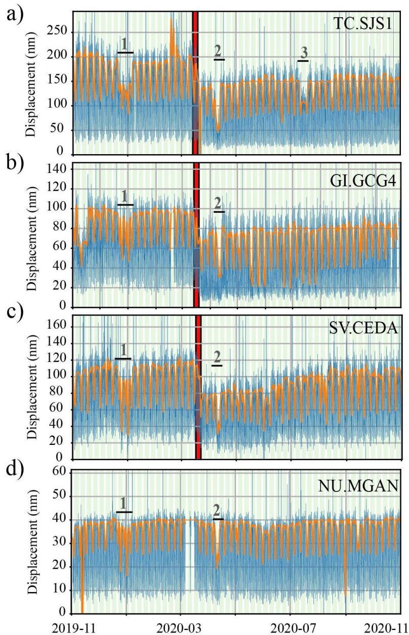
614 Figure 3. High-frequency seismic anthropogenic noise displacement (HFSAND-RMS) evolution at the seismic 615 stations near capitals of the countries studied. a) TC.SJS1 station in San Jose, Costa Rica. b) GI.GCG4 station in 616 Guatemala City, Guatemala. c) SV.CEDA station, near San Salvador in the city of La Libertad. d) NU.MGAN 617 station in Managua, Nicaragua. The blue line corresponds to the RMS amplitude time series of the vertical 618 component, filtered between 4 and 14 Hz, and the orange line corresponds to median day-time, between the 6 and 619 16 hours of local time. Gaps correspond to periods for which seismic data were unavailable and the vertical red 620 lines indicate the time when the first lockdown measures started in Central America. The numbers 1, 2, and 3, 621 show the New Year holidays of 2019, Easter of 2020, and a brief period in July 2020 when a strict return of 622 lockdown measures was implemented in Costa Rica, respectively. 623
