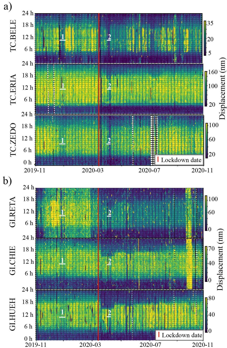
626 Figure 4. High-frequency seismic anthropogenic noise displacement (HFSAND-RMS) evolution for specific sites 627 in Costa Rica and Guatemala in an hourly grid representation. a) TC.BELE (central Costa Rica, near Juan 628 Santamaria international airport), TC.ERIA (northern Costa Rica, urban area), and TC.ZEDO (southern Costa 629 Rica, urban area). b) GI.HUEH (northwest of Guatemala, urban area), GI.RETA (southwest of Guatemala, urban 630 area), and GI.CHIE (east of Guatemala, urban area). The gaps correspond to the time periods for which seismic 631 data were unavailable and the vertical red lines indicate the time when the first lockdown measures started in 632 Central America. The numbers 1 and 2 show the New Year holidays of 2019 and Easter of 2020, respectively. 633
