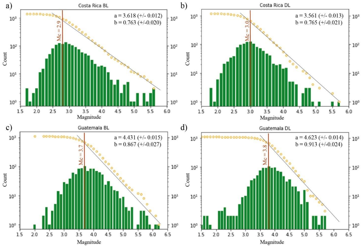
Figure 8. Magnitude-frequency distribution for earthquakes. a) Costa Rica before lockdown. b) Costa Rica during lockdown. c) Guatemala before lockdown. d) Guatemala during lockdown. Green bars represent the incremental (non-cumulative) number of earthquakes and yellow circles the cumulative distribution of events. The grey solid line fits the data points for the cumulative distribution above the magnitude of completeness ( M_c ). Vertical lines indicate the M_c estimated from the maximum curvature (MAXC) method.
