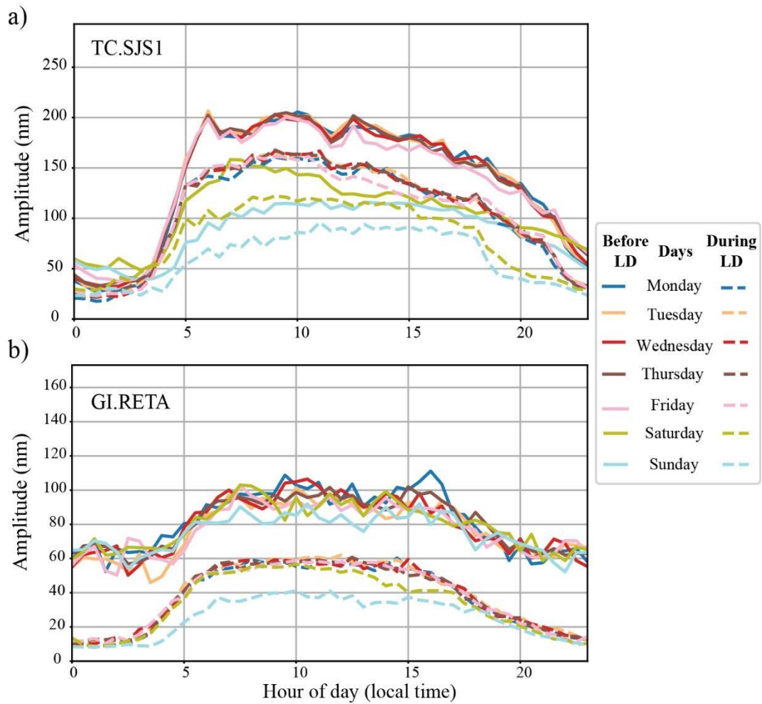
Figure 5. Daily variation of the median seismic noise per weekday, before and during the lockdown (LD). a) TC.SJS1 station in San Jose, Costa Rica. b) GI.RETA station in Retalhuleu, southwest of Guatemala.
