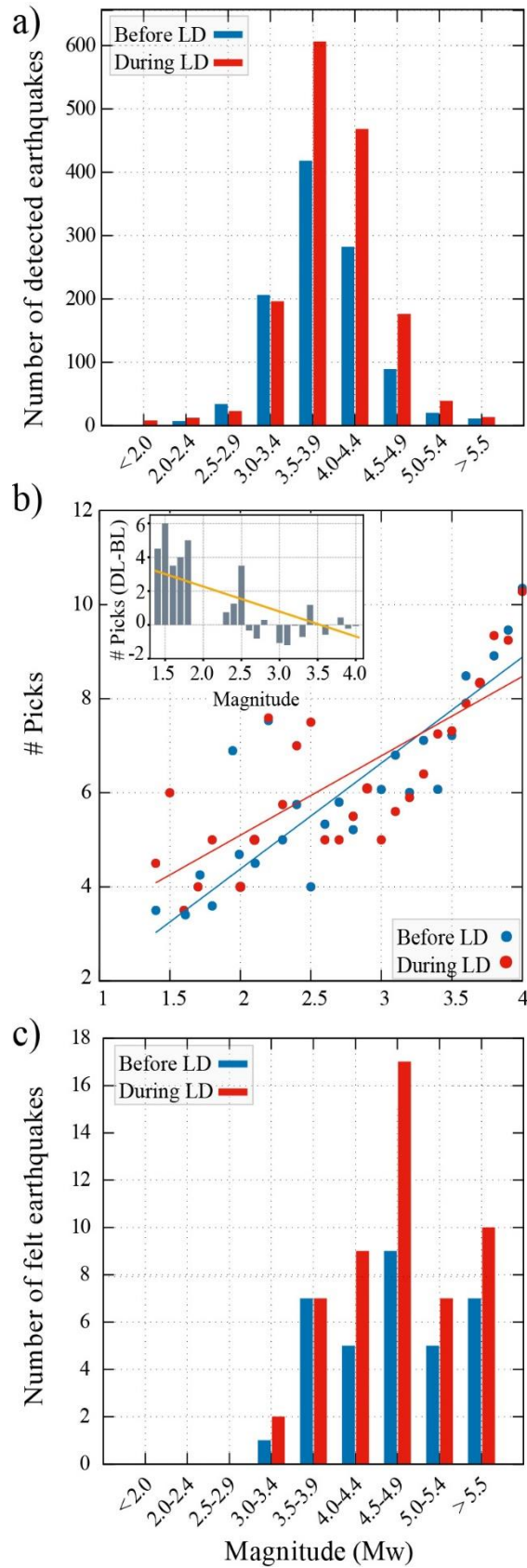
Figure 10. Event detection and felt earthquakes reported in Guatemala before (1 Nov 2019-15 Mar 2020) and during (16 Mar-31 Jul 2020) lockdown (LD) measures. a) Number of detected earthquakes. b) Earthquakes magnitude versus the average number of P-wave picks per Mw for the events with Mw < 4.0, and the corresponding linear fits. The inset graph shows the average difference in the number of picks for magnitude bins for the periods before (BL) and during (DL) lockdown. c) Number of felt earthquakes in Guatemala.
