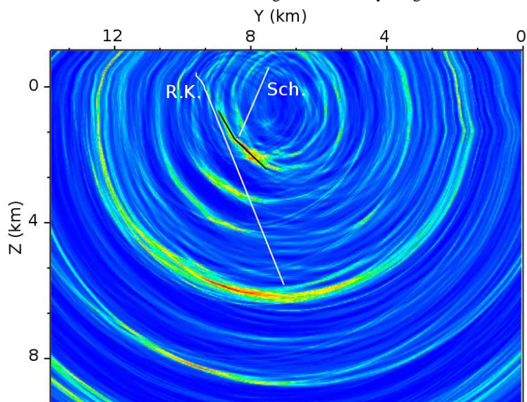
Figure 11: Comparison of the coherency image with the presumed Roter Kamm fault (R.K.) and Schwerin fault (Sch.) as derived from the geology map of the area. The deeper parts of these two structures are only extrapolated and not known.
