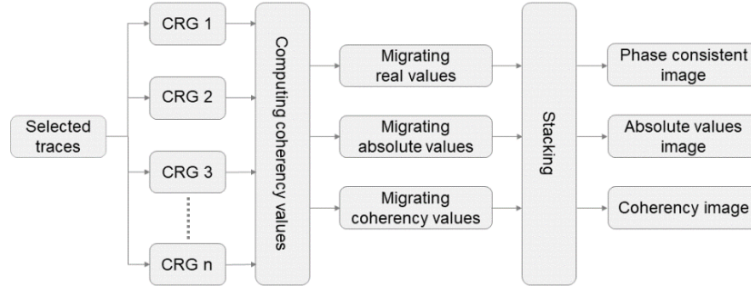
220 Figure 6: Schematic sketch of the imaging procedure.
