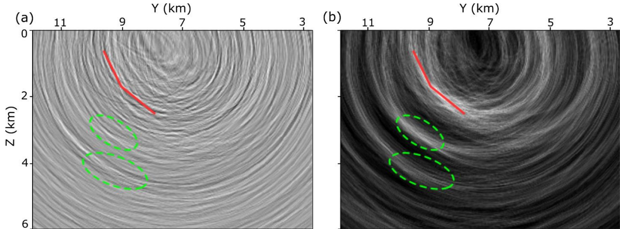
Figure 8: Zoomed-in illustration of the vertical slices through the phase-consistent image (a) and absolute values image (b) shown in figure 7. The red solid line shows the imaged part of the Roter Kamm fault and the green dashed ellipses refer to the reflectors B and D in figures 12 and 13.
