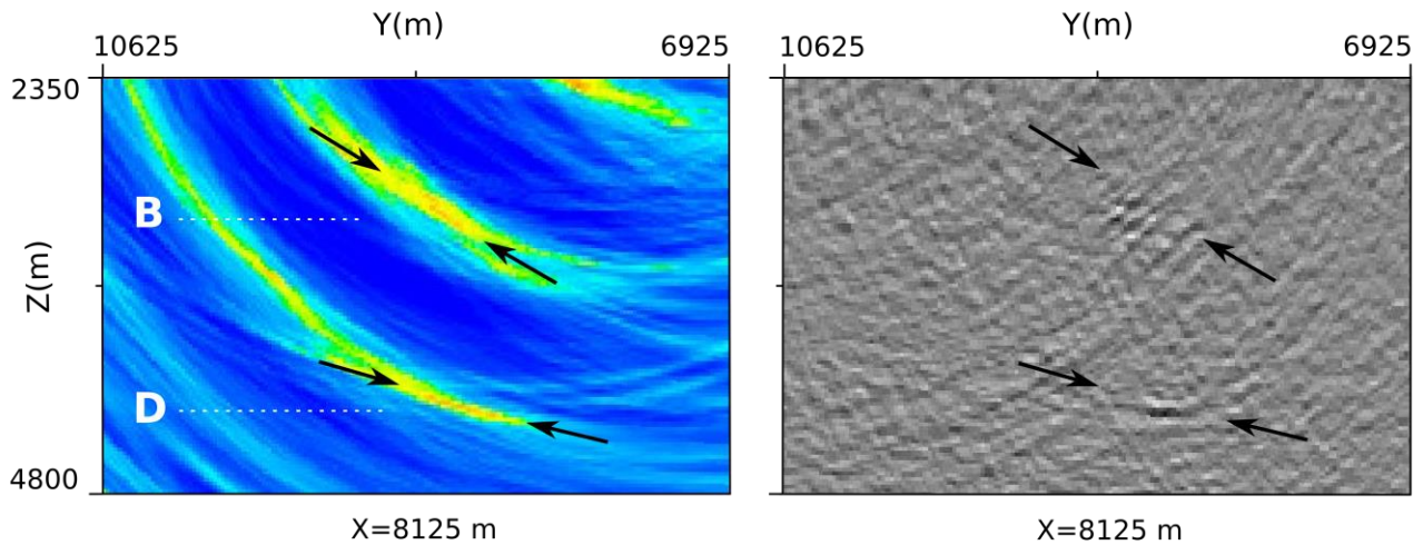
Figure 13: A zoomed illustration of the reflectors B and D (left) and their position shown by the arrows on the phase consistent active seismic image (right). Note that these slices are located at a distance of 250 m in x direction to the slices in figure 12.
