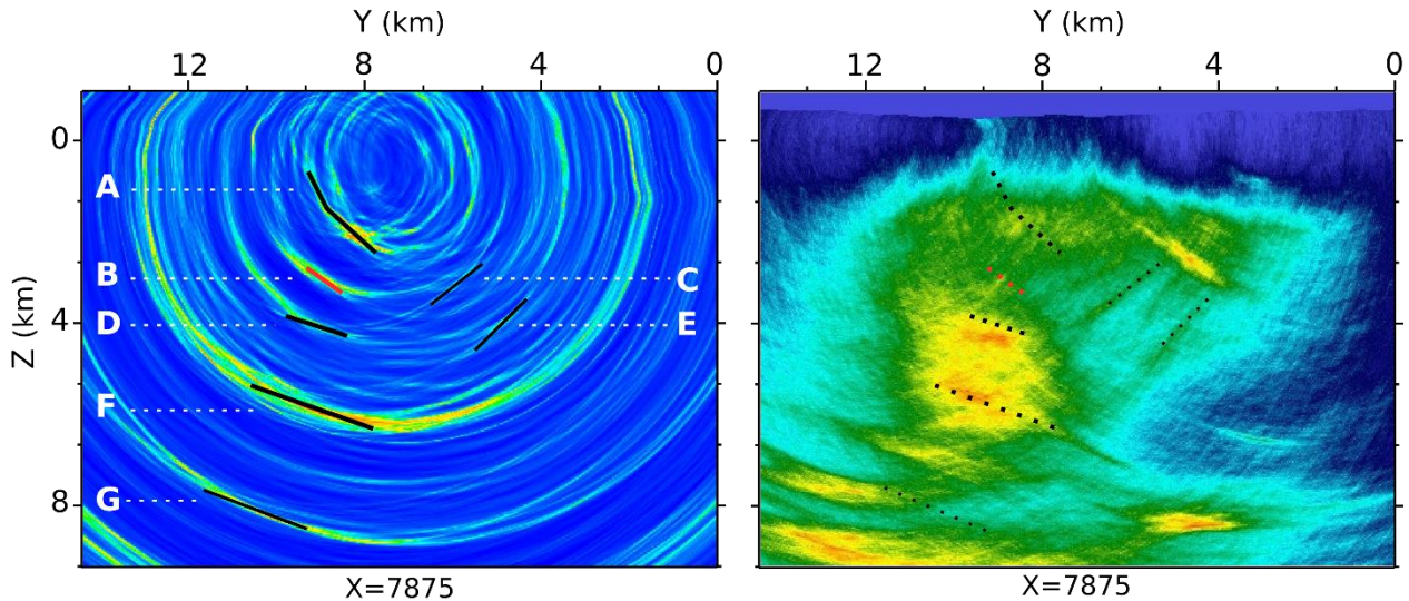
Figure 12: Comparison of the imaged structures in the coherency image (left) to the results of the active seismic survey in the area (right). The thick solid lines show the reflectors with higher image value, the thin solid lines mark the reflectors with a lower image value and the black dashed lines show them projected onto the active seismic image.
