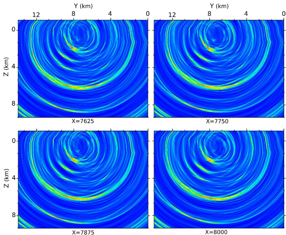
Figure 10: Sequential slices over a 375 m interval in x direction through the coherency image cube.
