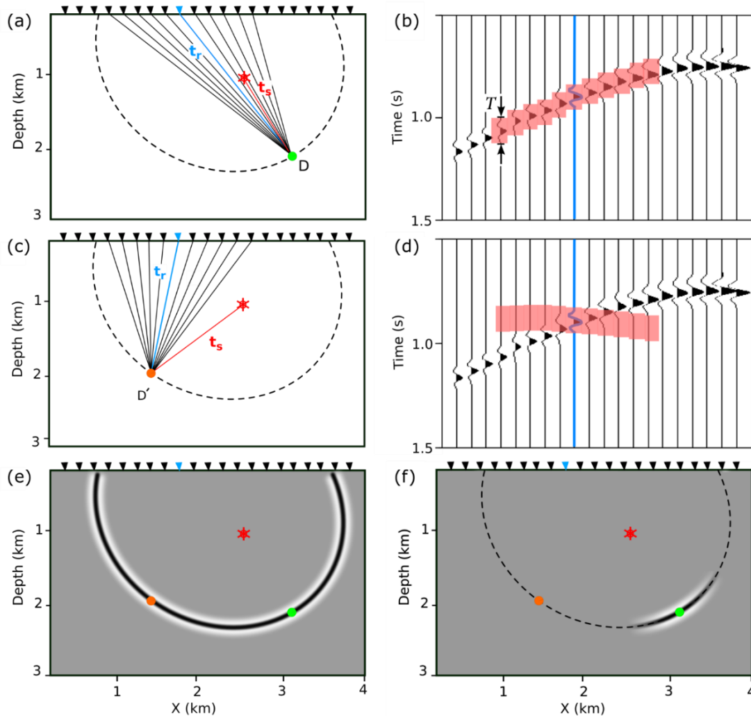
145 Figure 3: Concept of coherency migration. The red asterisk shows the source position and the triangles are surface receivers. The red boxes in (b) and (d) are the time windows with the length T defined on the neighbouring traces, with respect to the traveltime of the image point. For detailed description see text.
