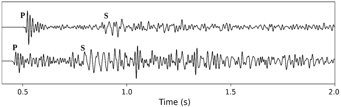
Figure 9: An example of the recorded waveforms used in the migration procedure. The P- and S- direct waves are marked for comparing the frequency content.
