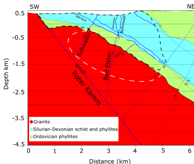
110 Figure 2: Vertical profile of the investigation area developed by Wallner et al. (2009). The black dashed line shows the approximate border of the mining area and the white ellipse shows the area where the hypocenters used in this study are located. For simplification, not all of the known faults are depicted in this figure.
