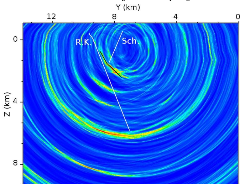
275 Figure 10: Comparison of the coherency image with the presumable Roter Kamm fault (R.K.) and Schwerin fault (Sch.) as derived from the geology map of the area. The deeper parts of these two structures are only extrapolated and not known.
