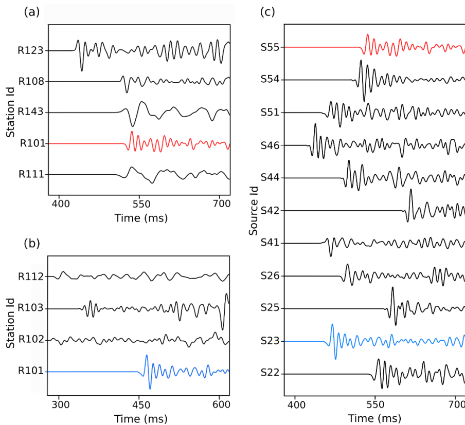
195 Figure 4: A comparison between common source gathers S55 and S23 (a and b) (same events, different receivers) and a common receiver gather R101 (c) (same receiver, different events). R101 is marked in red and blue for events S55 and S23, respectively.
