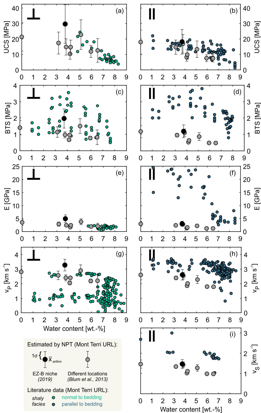
410 Figure 6: Comparison of estimated geomechanical and geophysical parameters of the Opalinus Clay in the EZ-B niche of the Mont Terri URL (black symbols, this study) with literature data for the shaly facies, normal (a–g) and parallel (b–i) to bedding. In addition, a second NPT dataset of Blum et al. (2013) from various locations in the URL (shaly facies) is shown (gray symbols). Literature data (green and blue symbols) originate from other niches in the Mont Terri URL and are mainly adapted after Jaeggi and Bossart (2014) and references herein (the full list of source documents is provided in Appendix A).
