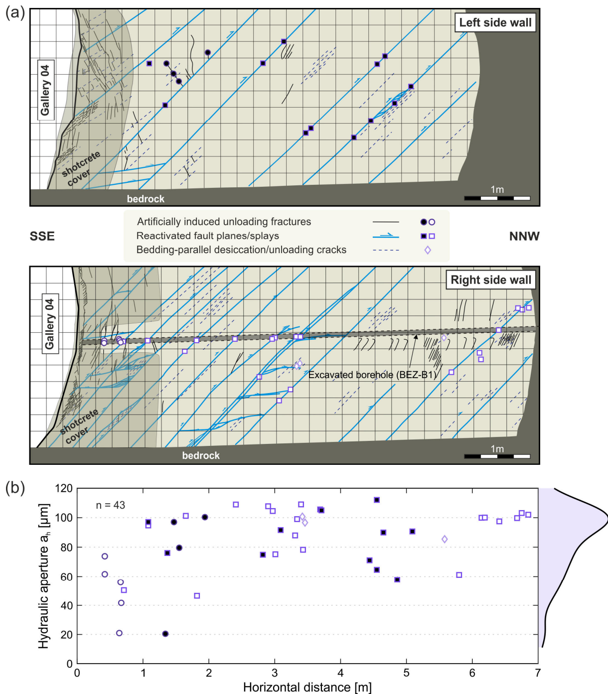
245 Figure 3: (a) Structural maps of the EZ-B niche with measurement points for hydraulic and mechanical aperture determination on the left (closed symbols) and right side wall (open symbols), modified after Nussbaum et al. (2005). (b) Hydraulic fracture apertures measured by air permeameter plotted against distance to Gallery 04. On the right side, the distribution of a_h is visualized by a probability density function obtained by Kernel density estimation (KDE).
