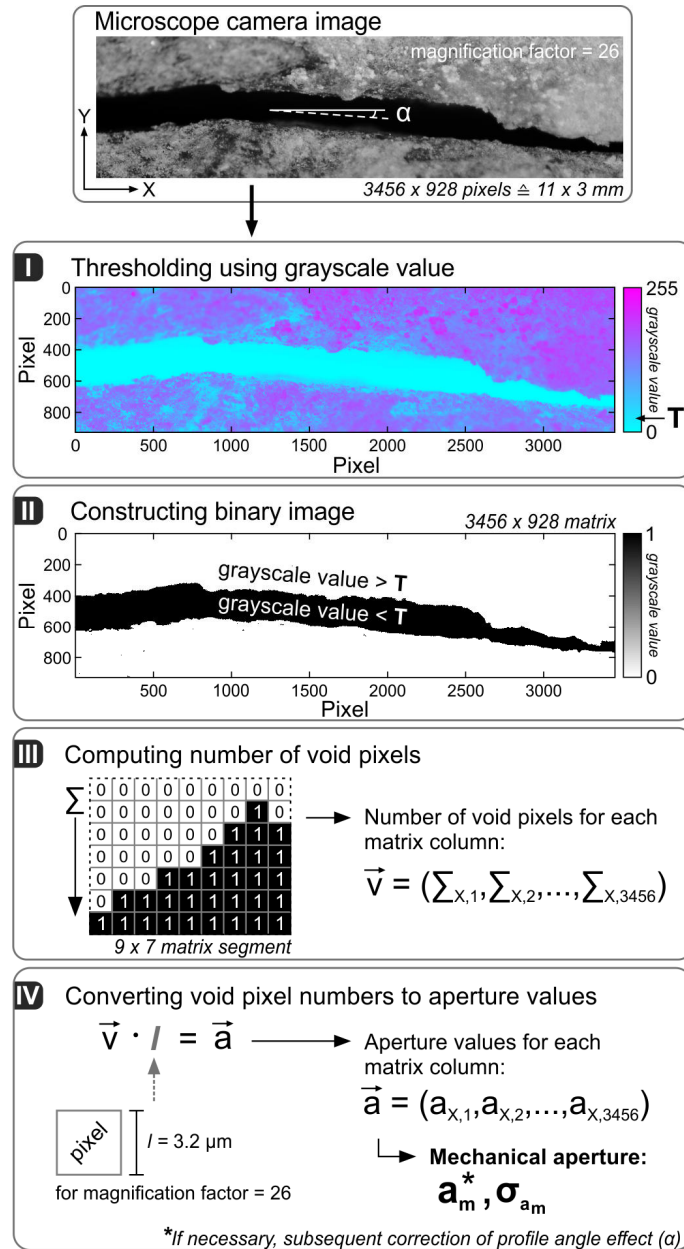
190 Figure 2: Workflow of the automatic approach for determining the mechanical fracture aperture based on microscope camera images of fracture trace segments.
