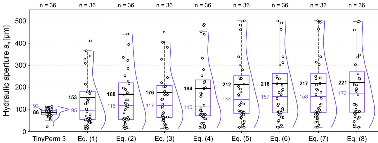
360 Figure 5: Comparison of hydraulic fracture apertures measured by air permeameter (TinyPerm 3) and estimated based on mean mechanical fracture apertures and standard deviations from microscopic fracture trace analysis. For each dataset, the arithmetic mean (bold black line), the median (thin purple line) and the probability density function (obtained by Kernel density estimation) is shown. Values above 550 \mu\text{m} are excluded from the graph.
