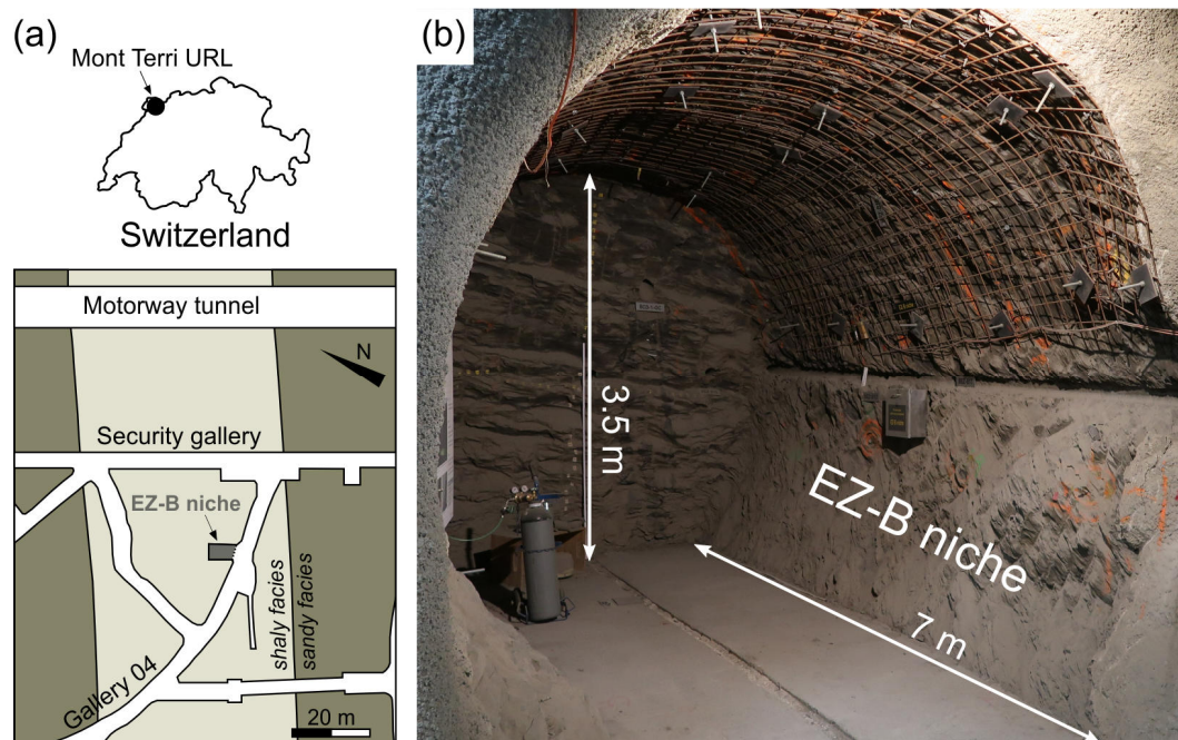
150 Figure 1: (a) Location of the Mont Terri Underground Rock Laboratory (URL) alongside the security gallery of the Mont Terri motorway tunnel and the EZ-B niche situated in the shaly facies of the Opalinus Clay. (b) Photo and dimensions of the EZ-B niche, where data acquisition was conducted. In the entrance area, shotcrete partly covers the rock surface on the left and right side wall.
