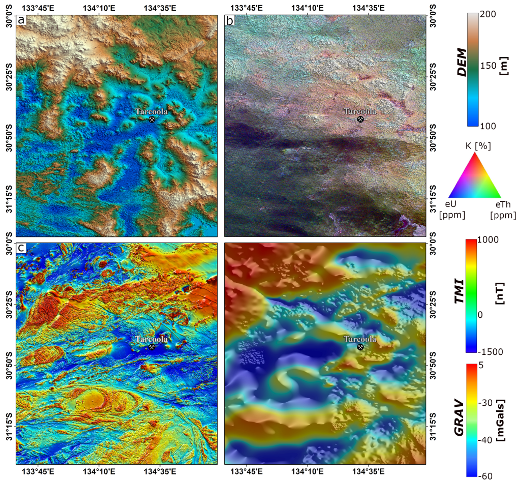
Figure 5. a Colour digital elevation model (laser altimeter) [min: 84.08 m; max: 365.33 m], b color radiometric dose rate (NASVD corrected) [min: 0.074 nGy/hr; max: 239.30 nGy/hr], c color total magnetic intensity (reduced to pole) [min: -1978.16 nT; max: 21638.8 nT], and d color and hillshaded Bouguer Anomaly gravity image (Katona, 2017) [min: -158.15; max: 64.74]. Data source: GCAS Region 9A, SARIG 2020
