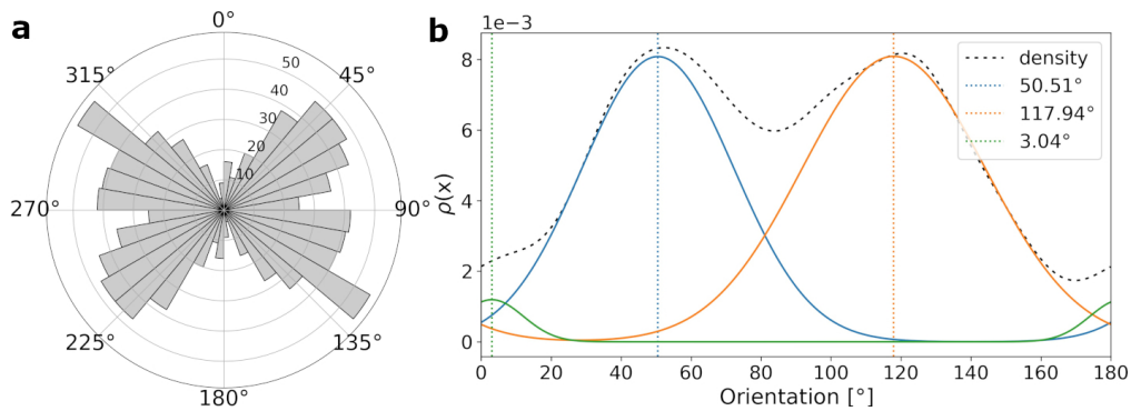
Figure 5. Directional analysis of structural interpretation (Figure 2a). a Rose diagram showing the distribution of strike directions of the data with a bin size of 10 degrees. b Gaussian distributions fitted to the probability density function obtained via kernel density estimation.
