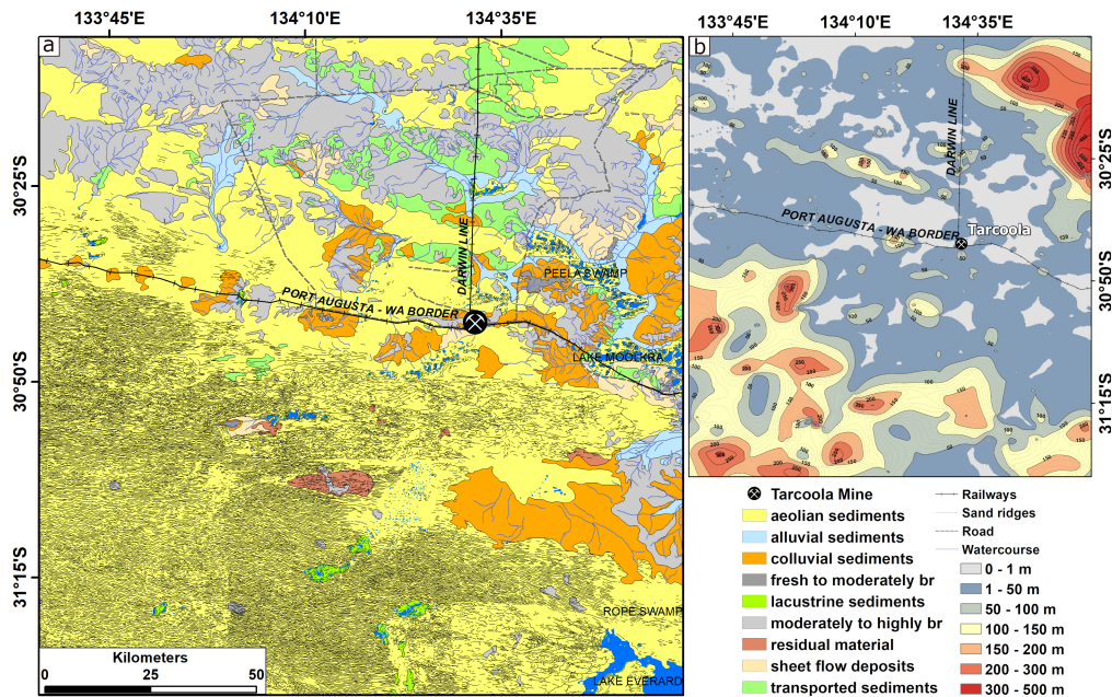
Figure 3. a Surface feature map displaying regolith material (Krapf et al., 2012), roads, watercourses and sand ridges. Especially linear structures such as roads and sand ridges are expected to strongly influence the automated lineament extraction process. b Depth to basement map (Cowley et al., 2018).
