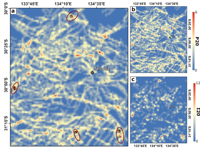
Figure 11. a Targeting map derived from “Surface manual” combined with the structural interpretation (Figure 2a). b Lineament density map (P20). c Intersection density map (I20). Potential targeting areas that are indicated by red ellipses.
