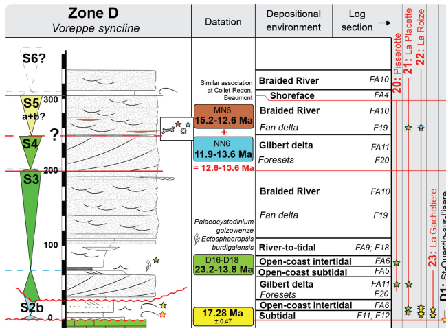
Figure A4: Synthetic section of the Mioene of the Voreppe syncline (Zone D). See Fig. 3 for location of the sedimentological sections and Fig. A13 for legend. For more details, see section 6.3.4. and appendix 39 in Kalifi (2020) and references therein.
