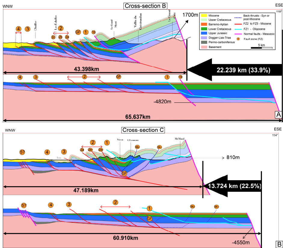
1125 Figure 18: Balanced cross-sections throughout the Chartreuse massif using the Move software. To facilitate the restoration, we assume that the ZF2 to ZF4 are rooted below a single Belledonne basal thrust. (A) Cross-section B (Fig. 11B). (B) Cross-section C (Fig. 11C). See Fig. 1B for locations.
