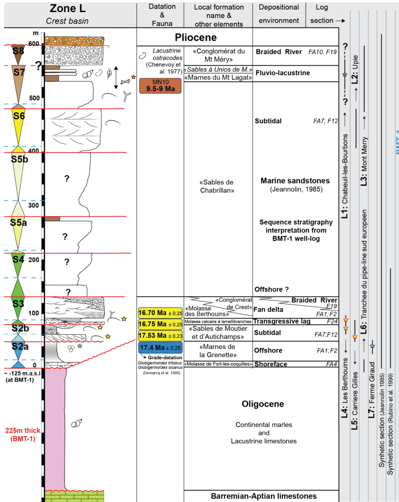
Figure A12: Synthetic section of the Miocene of the Crest basin (Zone L). See Fig. 3 for location of the sedimentological sections and Fig. A13 for legend. For more details, see section 6.4.5, and appendix 82 in Kalifi (2020) and references therein.
