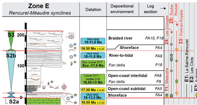
Figure A5: Synthetic section of the Mioene of the Rencurel-Méaudre synclines (Zone E). See Fig. 3 for location of the sedimentological sections and Fig. A13 for legend. For more details, see section 6.3.5. and appendix 44 in Kalifi (2020) and references therein.
