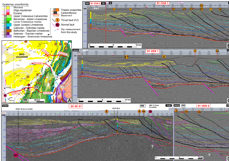
560 Figure 9: Seismic profiles along the Vercors and Chartreuse massifs (seismic lines published by Deville et al. [2021] and 565 reinterpreted ). (A) Geographical and geological locations of the interpreted seismic lines. (B) Seismic profiles 91CHA1 and 91CHA2. Interpretation is proposed using PA-1 well data and fieldwork data. Note that the Outherans blind thrust corresponds further north to the GF thrust. (C) Seismic profiles 91VER1. Interpretation is proposed using BR-1 well data and fieldwork data. (D) Seismic profiles 82SE01-91VER2. Interpretation is proposed using SLF-2, SL-2 and extrapolated BB1 and GVA-1 well data and fieldwork data.
