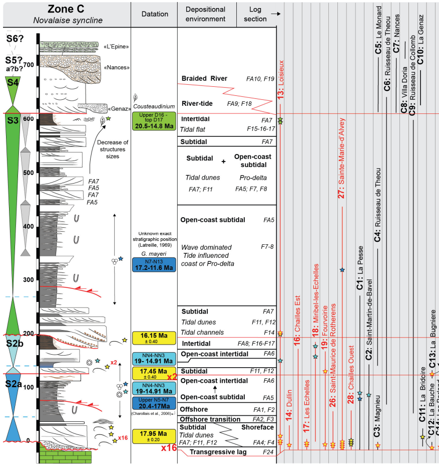
190 Figure A3: Synthetic section of the Miocene of the Novalaise syncline (Zone C). See Fig. 3 for location of the sedimentological sections and Fig. A13 for legend. For more details, see section 6.3.3. and appendix 30 in Kalifi (2020) and references therein.
