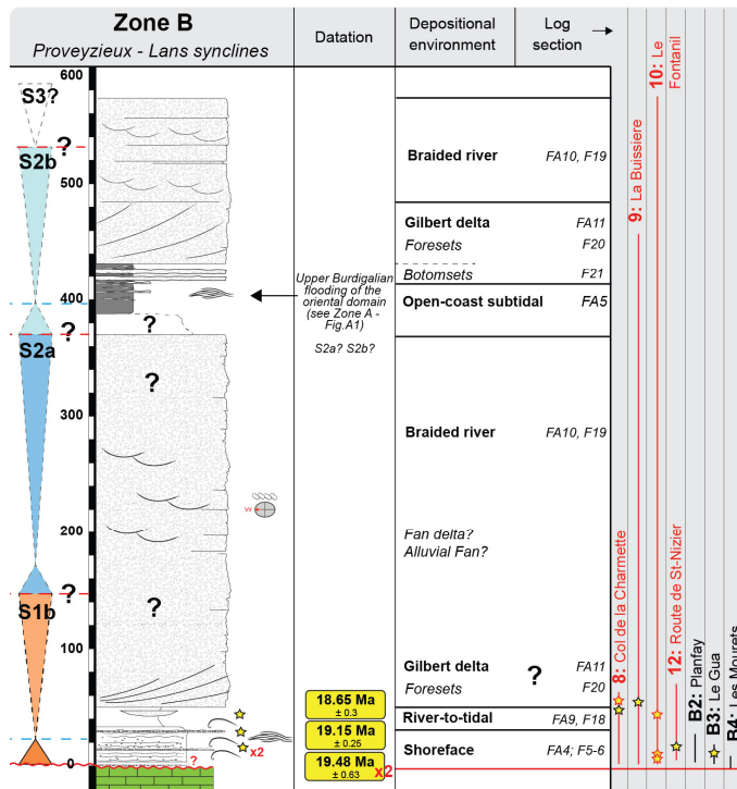
185 Figure A2: Synthetic section of the Miocene of the Proveyzieux-Lans synclines (Zone B). See Fig. 3 for location of the sedimentological sections and Fig. A13 for legend. For more details, see section 6.3.2. and appendix 26 in Kalifi (2020) and references therein.
