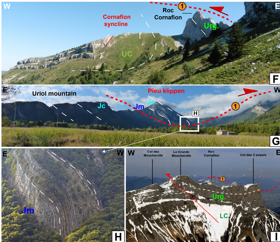
Figure 6: Field and aircraft pictures of the Chartreuse Orientale and Moucherotte thrusts (FZ1) in southern Chartreuse and northern Vercors. Geographical and geological locations of viewpoints A to I locations in Fig. 7A. m= Miocene; UC= Upper Cretaceous; Urg.= Urganian (Barremian-Aptian limestones); LC= Lower Cretaceous; Jc= Upper Jurassic limestones; Jm= Upper Jurassic marls. Dashed white lines underline the stratifications. Thrust faults in red. Geographical and geological locations of viewpoints A to I in Fig. 7A. Orange circle= Fault zone (FZ1). (A, B) The Néron and Moucherotte thrusts, aerial views from the N. The Provezieux Miocene deposits are underthrust below the Néron syncline. Beyond the Isère valley, the Sassenage fold capped with Miocene deposits is underthrust below the Moucherotte massif. Note that Provezieux syncline corresponds to two synclines separated by an anticline. (C) View towards the south of the Col de l'Arc and the Crête des Crocs: the folded Urganian is thrust above the Upper Cretaceous. (D) Urganian limestones of the Moucherotte anticline in the FZ1 hangingwall. (E) View towards the west of the eastern flank of the Moucherotte massif with the FZ1 geometry. (F) View towards the north of the Cornafion syncline. The Urganian is overturned, in the FZ1 footwall. (G) Duplication of the Jurassic series in the Pieu klippen, view from the North; (H) Zoom on the anticline on the hangingwall of the FZ1 in the Pieu klippen. (I) View towards the north of the Grande Moucherolle, where autochthonous series are weakly deformed.
