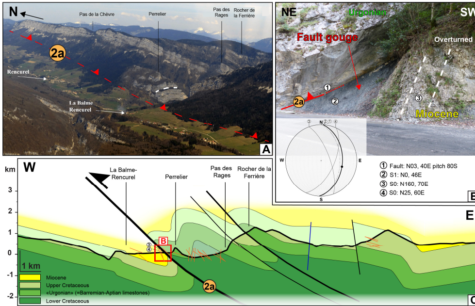
540 Figure 8: The Rencurel thrust in the Vercors massif. Orange lines= projected dip measurements. Blue line = Right-lateral strike slip fault. Black line = Thrust. (A) The N-S Rencurel thrust that juxtaposes Cretaceous units on top of Miocene Molasse deposits. (B) Outcrop of the Rencurel thrust along the D103 road, SE to the La Balme-Rencurel village, exhibiting Barremian-Aptian limestones thrusting on top of overturned Miocene deposits striking N160, 70°E. Corresponding stereographic diagram (lower hemisphere) at the bottom. (C) E-W cross-section along the “gorges de la Bourne”. See Fig. 7A for location of the cross-section and dip measures on map view.
