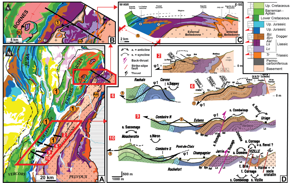
Figure B1B2: The FZ1 along the western edge of the Belledonne massif (A) Localization of the cross-sections; (B) Close-up view of the FZ1 between the eastern border of the Bauges and Belledonne massifs. Localization of the ESE-WNW cross-section of Gidon (2004) presented in (C). SU= Sulens klippen. Am= Internal Belledonne thrust. (D) The FZ1 along the Gresivaudan hills adapted from Barf y and Gidon (1996).
