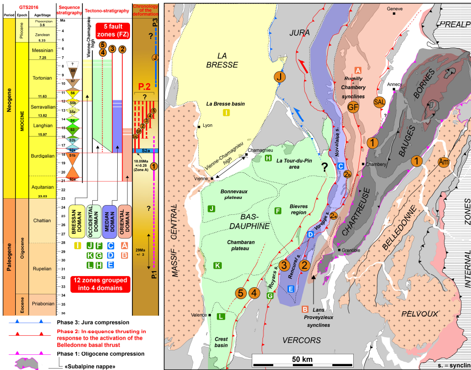
Figure 16: Summary of the structural, chronostratigraphical and tectonostratigraphic results of this study. The 11 sedimentary sequences revealed 12 palaeogeographical zones, themselves grouped into 4 palaeogeographical domains. 5 fault zones (FZ1-5) were identified. Based on the established tectono-sedimentary evolution, three compressive phases were identified. The main phase corresponds to Phase 2, which involved the progressive onset, from east to west, of the SAL fault to FZ5 in response to the onset of the Belledonne basal thrust.
