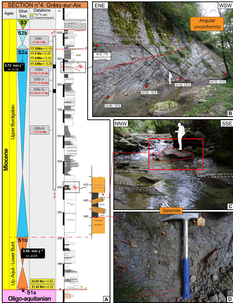
720 | Figure 12: (A) Grésy-sur-Aix sedimentological section with sequence S2a syntectonic deposits indicated: seismite near the bottom (see also C and D) and angular unconformity near the top (see also B). The S2a sequence boundary was observed and dated in the Forezan section (5, Fig. 2). Legend in Fig. 5. Black box= Average sedimentation rate of the sequence; (B) The angular unconformity has established between 17.53 and 17.23 Ma within Chron C5Dn. White dashed lines = bedding. Red line = erosive surface. Red
