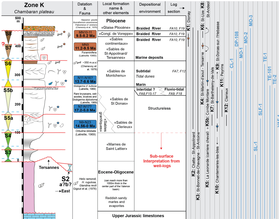
Figure A11: Synthetic section of the Miocene of the Chambaran plateau (Zone K). See Fig. 3 for location of the sedimentological sections and Fig. A13 for legend. For more details, see section 6.4.4. and appendix 69 in Kalifi (2020) and references therein.
