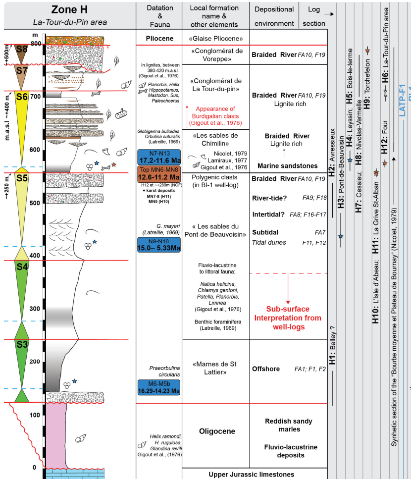
Figure A8: Synthetic section of the Miocene of the La-tour-du-Pin area (Zone H). See Fig. 3 for location of the sedimentological sections and Fig. A13 for legend. For more details, see section 6.4.1. and appendix 59 in Kalifi (2020) and references therein.
