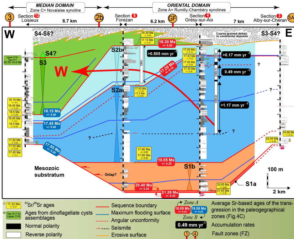
755 Figure 13: Westward migration of the depocenter during the lower Miocene (red curved arrow). The sedimentological sections were projected on a E-W axis, which corresponds to a direction orthogonal to the thrusts. See Fig. 3 for location of the transect and sedimentological sections. Red squares = sedimentological sections quoted in the text and used for correlations. The dashed red line corresponds to the angular unconformity presented in Fig. 12B.
