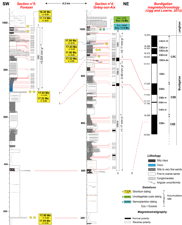
295 Figure 2: Magnetostratigraphy of the Forézán and Grésy-sur-Aix sections, integrated with Strontium and biostratigraphic dating.
