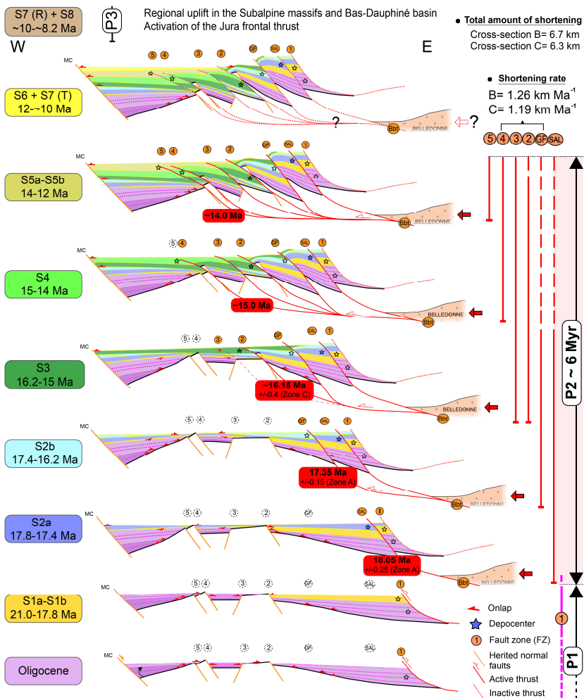
Figure 17: Schematic framework summarizing the main phases of thrust propagation at the western alpine front, and their chronology, based on a thorough revision of the regional chronostratigraphy between the Oligocene and the late Miocene. The horizontal and vertical scales are not respected. MC= Massif Central; P= Tectonic phase; T= Transgressive deposits; R= Regressive deposits. The colored boxes on the left side correspond to the homogenized ages of the eustatic-driven depositional sequences (Fig. 4A, B). Red boxes highlight the timing of fault initiation deduced from depocenter migration (Fig. 13). Vertical lines on the right represent the proposed timing of activity for each fault.
