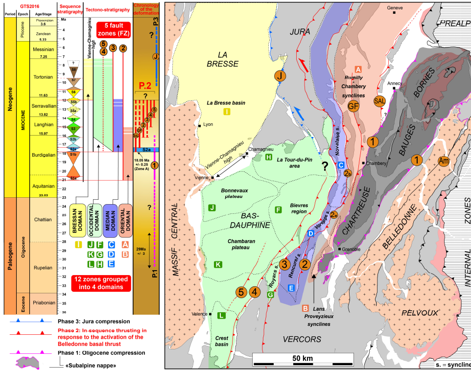
775 Figure 16: Summary of the structural, chronostratigraphical and tectonostratigraphic results of this study. The 11 sedimentary sequences revealed 12 paleogeographical zones, themselves grouped into 4 paleogeographical domains. 5 fault zones (FZ1-5) were identified. Based on the established tectono-sedimentary evolution, three compressive phases were identified. The main phase corresponds to Phase 2, which involved the progressive onset, from east to west, of the SAL fault to FZ5 in response to the onset of the Belledonne basal thrust.
