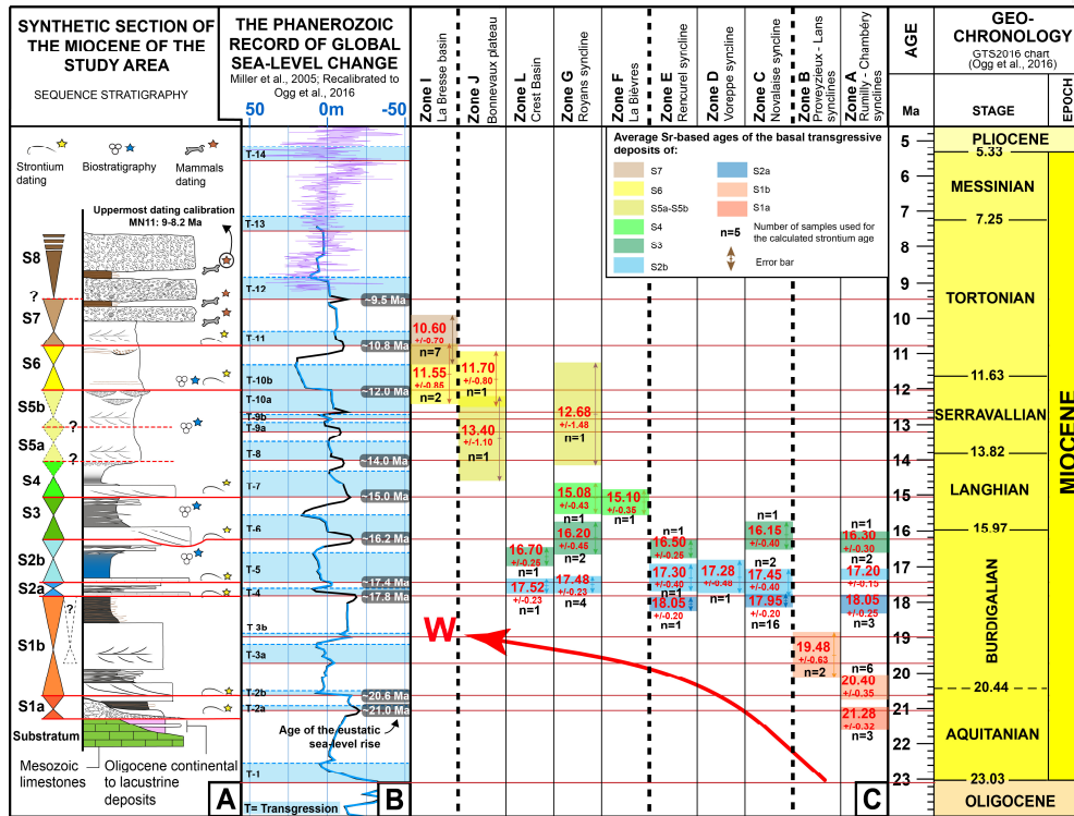
305 Figure 4: The Miocene chronostratigraphy of the subalpine massifs, southern Jura and adjacent basins (Bas-Dauphiné, La Bresse, Crest). (A) Synthetic section of the Miocene of the study area and the 11 Miocene depositional sequences. Legend in Fig. 5; (B) The eustatic curve of Miller et al. (2005) recalibrated with the Global Time Scale (GTS) of Ogg et al. (2016); (C) Average Sr-based ages of the transgressions in the paleogeographical/paleogeographical zones. n: number of age values. Only ages of samples with \delta^{13}C values >1\% (Table S2) are considered here (maximum confidence zone). Red curved arrow= Westward migration of the marine deposits during the lower Miocene. 310
