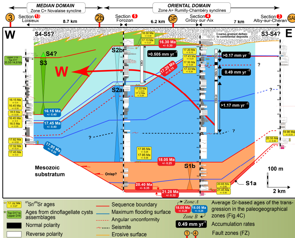
670 Figure 13: Westward migration of the depocenter during the lower Miocene (red curved arrow). The sedimentological sections were projected on a E-W axis, which corresponds to a direction orthogonal to the thrusts. See Fig. 3 for location of the transect and sedimentological sections. Red squares = sedimentological sections quoted in the text and used for correlations. The dashed red line corresponds to the angular unconformity presented in Fig. 12B.
