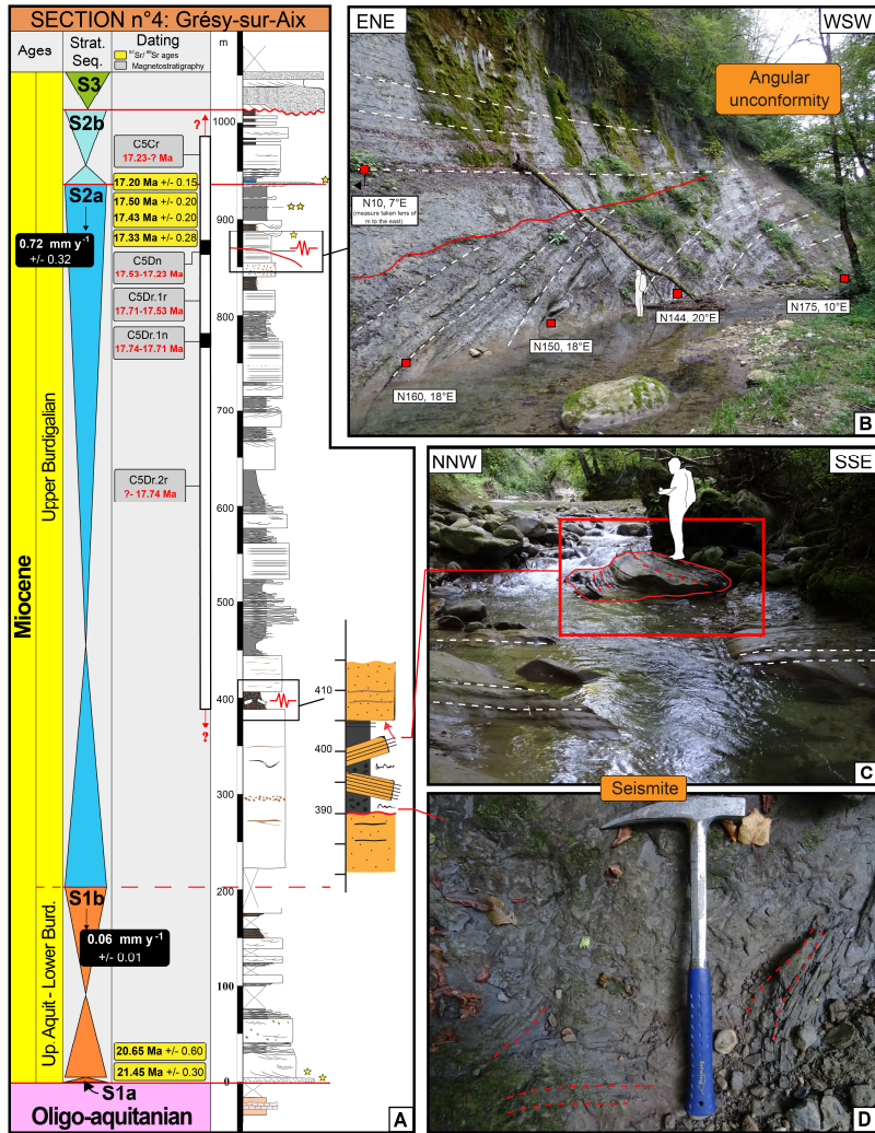
Figure 12: (A) Grésey-sur-Aix sedimentological section with sequence S2a syntectonic deposits indicated: seismite near the bottom (see also C and D) and angular unconformity near the top (see also B). The S2a sequence boundary was observed and dated in the Forezan section (5, Fig. 2). Legend in Fig. 5. Black box= Average sedimentation rate of the sequence; (B) The angular unconformity has established between 17.53 and 17.23 Ma within Chron C5Dn. White dashed lines = bedding. Red line = erosive surface. Red
