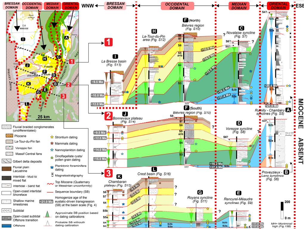
320 Figure 5: Spatio-temporal distribution of the Miocene depositional sequences of the sub-alpine massifs, southern Jura synclines, Bas-Dauphiné, Crest and La Bresse, which highlight the four depositional domains resulting from the sequence stratigraphical interpretation of the 12 palaeogeographical/palaeogeographical zones (presented in details in Fig. S5 to Fig. S17).
