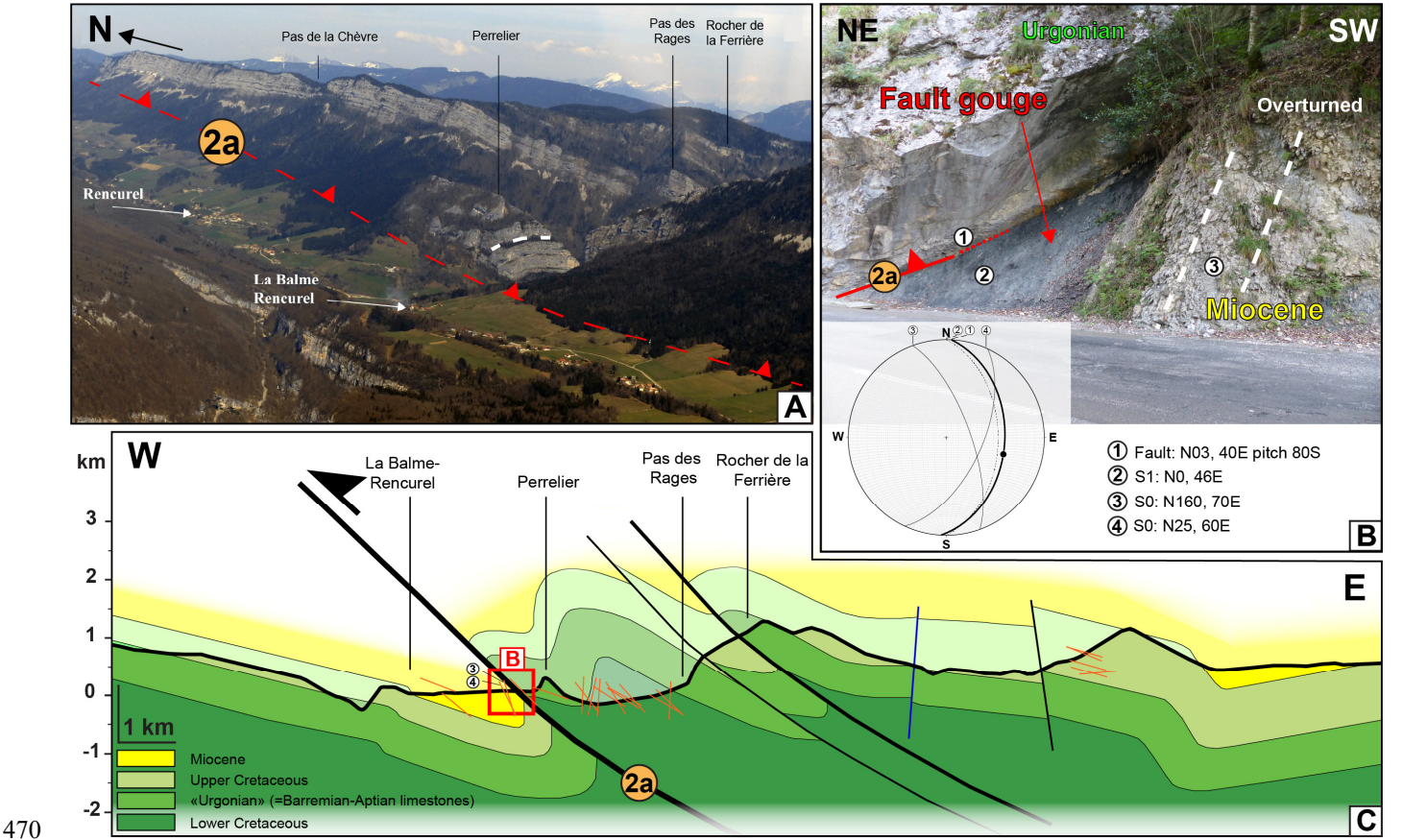
Figure 8: The Rencurel thrust in the Vercors massif. Orange lines= projected dip measurements. Blue line = Right-lateral strike slip fault. Black line = Thrust. (A) The N-S Rencurel thrust that juxtaposes Cretaceous units on top of Miocene Molasse deposits. (B) Outcrop of the Rencurel thrust along the D103 road, SE to the La Balme-Rencurel village, exhibiting Barremian-Aptian limestones thrust on top of overturned Miocene deposits. Corresponding stereographic diagram (lower hemisphere) at the bottom. (C) E-W cross-section along the “gorges de la Bourne”. See Fig. 7A for location of the cross-section and dip measures on map view.
