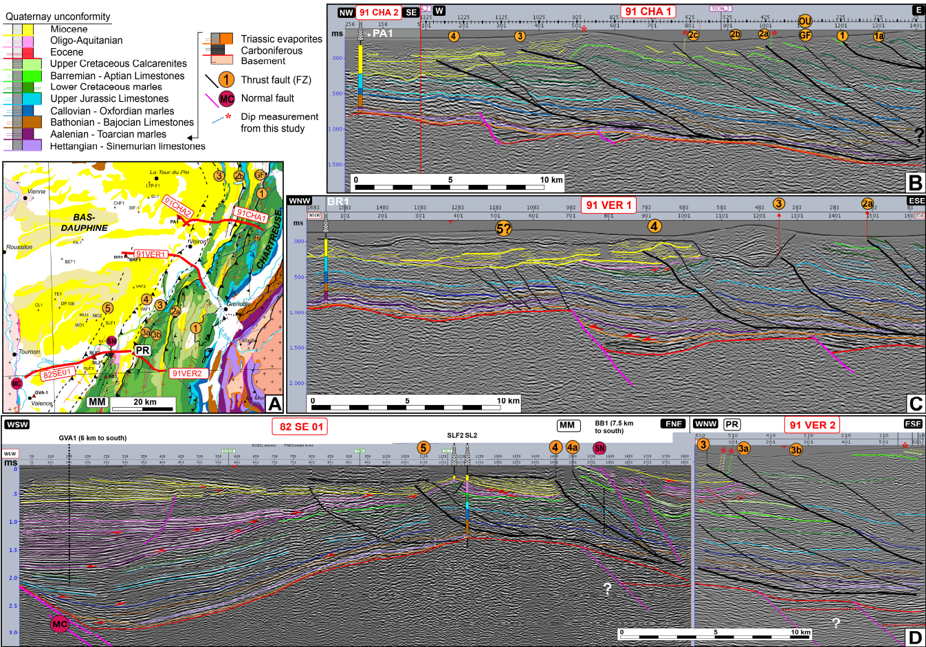
Figure 9: Seismic profiles along the Vercors and Chartreuse massifs (seismic lines published by Deville et al. [2021] and reinterpreted). (A) Geographical and geological locations of the interpreted seismic lines. (B) Seismic profiles 91CHA1 and 91CHA2. Interpretation is proposed using PA-1 well data and fieldwork data. Note that the Outherans blind thrust corresponds further north
