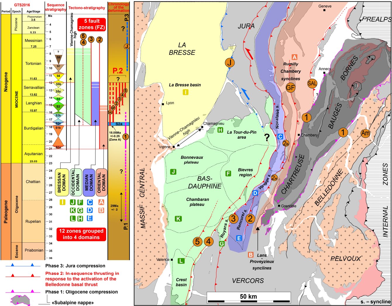
Figure 16: Summary of the structural, chronostratigraphical and tectonostratigraphic results of this study. The 11 sedimentary sequences revealed 12 paleogeographical zones, themselves grouped into 4 palaeogeographical domains. 5 fault zones (FZ1-5) were identified. Based on the established tectono-sedimentary evolution, three compressive phases were identified. The main phase corresponds to Phase 2, which involved the progressive onset, from east to west, of the SAL fault to FZ5 in response to the onset of the Belledonne basal thrust.
