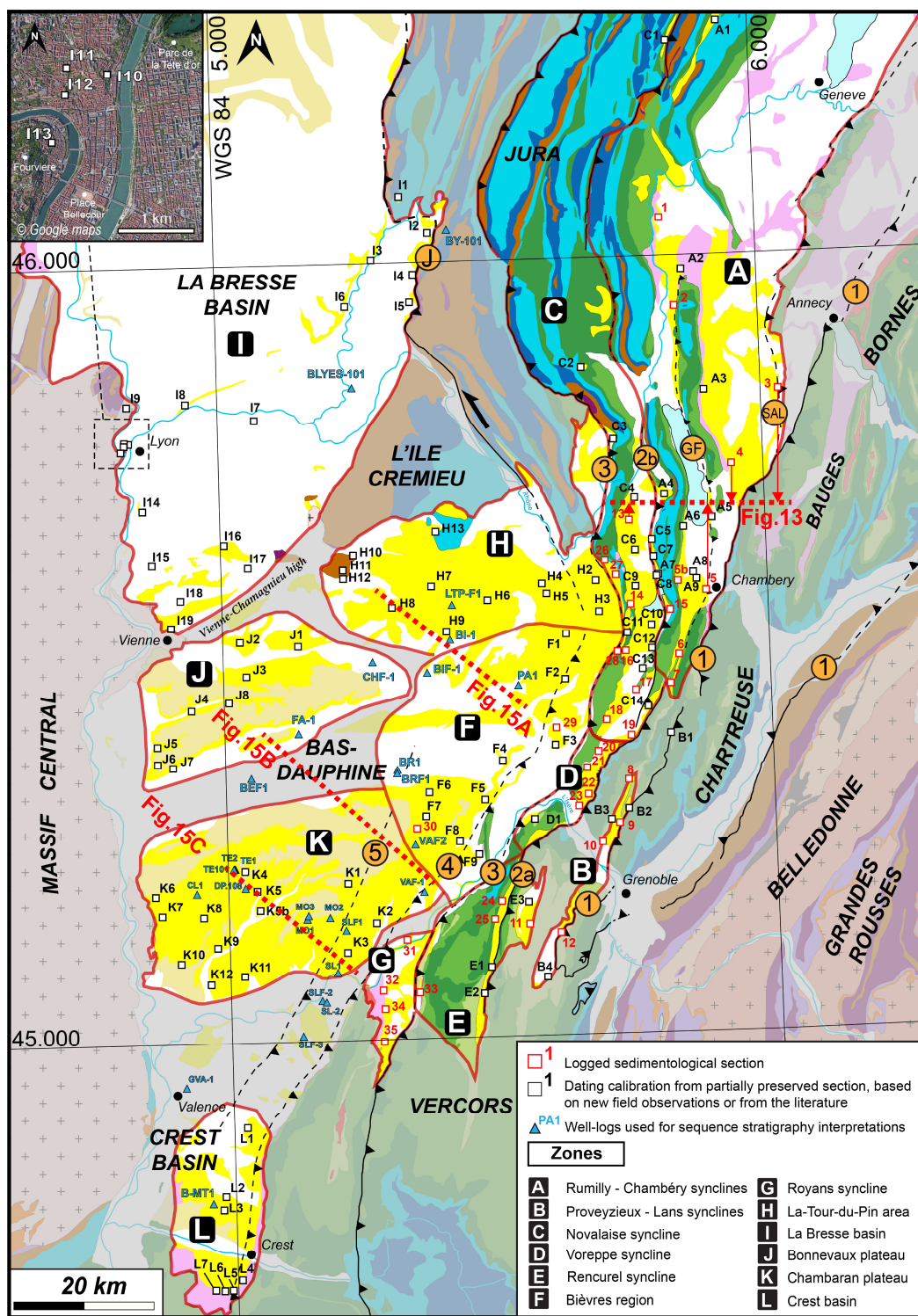
300 Figure 3: The 12 palaeogeographical zones of the Miocene basin of the subalpine massifs, southern Jura and adjacent basins (Bas-Dauphiné, La Bresse, Crest). Sedimentological and chronostratigraphical records of each zone are provided in Fig. S5 to Fig. S17.
