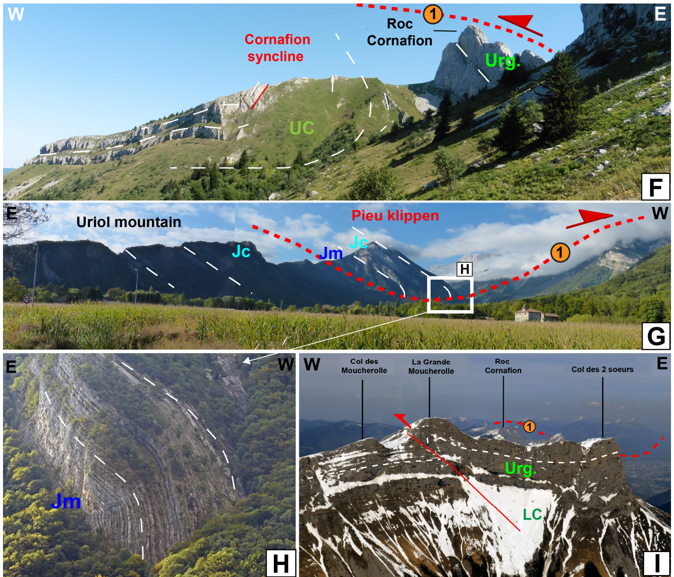
380 Figure 6: Field and aircraft pictures of the Chartreuse Orientale and Moucherotte thrusts (FZ1) in southern Chartreuse and and northern Vercors. See viewpoints A to I locations in Fig. 7A. m= Miocene; UC= Upper Cretaceous; Urg. = Urganian (Barremian- Aptian limestones); LC= Lower Cretaceous; Jc= Upper Jurassic limestones; Jm= Upper Jurassic marls. Dashed white lines underline the stratifications. Thrust faults in red. Orange circle= Fault zone (FZ). (A, B) Néron and Moucherotte thrusts, aerial 385 views from the N. The Provezieux Miocene deposits are underthrust below the Néron syncline. Beyond the Isère valley, the Sassenage fold capped with Miocene deposits is underthrust below the Moucherotte massif. Note that Provezieux syncline corresponds to two synclines separated by an anticline. (C) View towards the south of the Col de l'Arc and the Crête des Crocs: the folded Urganian is thrust above the Upper Cretaceous. (D) Urganian limestones of the Moucherotte anticline in the FZ1 hangingwall. (E) View towards the west of the eastern flank of the Moucherotte massif with the FZ1 geometry. (F) View towards the north of the Cornafion syncline. The Urganian is overturned, in the FZ1 footwall. (G) Duplication of the Jurassic series in the 390 Pieu klippen, view from the North; (H) Zoom on the anticline on the hangingwall of the FZ1 in the Pieu klippen. (I) View towards the north of the Grande Moucherolle, where autochthonous series are weakly deformed.
