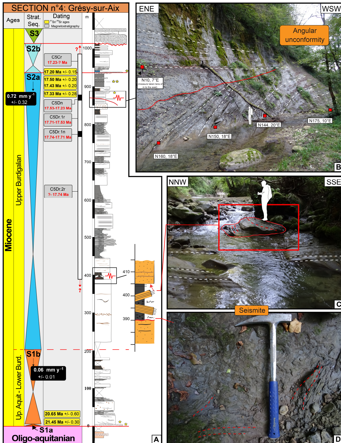
Figure 12: (A) Grésy-sur-Aix sedimentological section with sequence S2a syntectonic deposits indicated: seismitite near the bottom (see also C and D) and angular unconformity near the top (see also B). The S2a sequence boundary was observed and dated in the Forezan section (5, Fig. 2). Legend in Fig. 5. Black box= Average sedimentation rate of the sequence; (B) The angular unconformity has established between 17.53 and 17.23 Ma within Chron C5Dn. White dashed lines = bedding. Red line = erosive surface. Red
