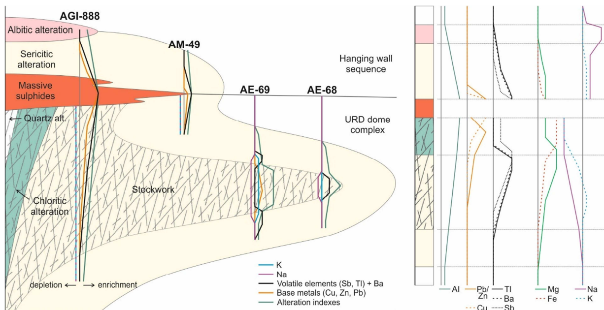
970 Figure 16: Schematic summary of the main observations performed in this study on vectoring tools related to hydrothermal alteration mineral zoning and whole rock geochemistry of major and trace elements. Sodium enrichment in the albite alteration zone is inferred and needs to be confirmed. Not to scale. AI: Alteration indexes.
