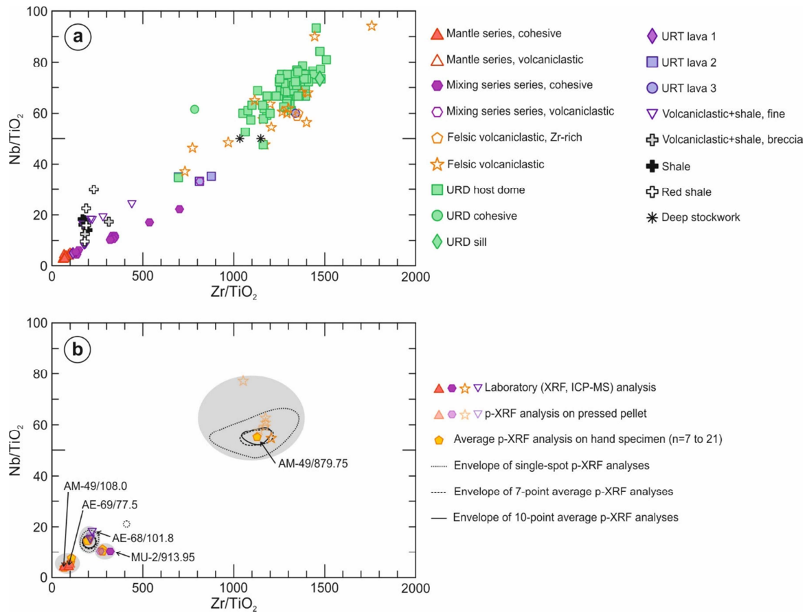
Figure 13: Nb/TiO 2 vs. Zr/TiO 2 discrimination diagrams showing (a) laboratory whole rock geochemistry data (XRF + ICP-MS) and (b) comparison between laboratory and p-XRF whole rock geochemistry data of representative samples. Ratios calculated with TiO 2 content in wt. % and Nb and Zr contents in μg -1 .
