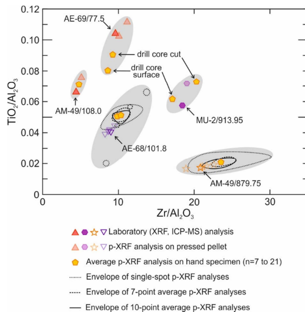
895 Figure 12: \text{TiO}_2/\text{Al}_2\text{O}_3 vs. \text{Zr}/\text{Al}_2\text{O}_3 discrimination diagram comparing whole rock geochemistry data obtained from laboratory (XRF + ICP-MS) and p-XRF analysis of representative samples. For each sample, the data obtained from 1) laboratory analysis (solid symbols), 2) pressed powder pellet p-XRF analysis (faded symbols), and 3) average hand specimen p-XRF analysis (yellow pentagons) are represented. In addition, for samples AM-49/879.75 and AE-68/101.8, the envelopes containing single spot-analyses, 7-point averages, and 10-point averages for hand specimen analyses are also shown to provide a general idea of the effect of multiple spot averaging on analytical precision. Ratios calculated with \text{TiO}_2 and \text{Al}_2\text{O}_3 contents in wt. % and Zr contents in \mu\text{g}\cdot\text{g}^{-1} . 900
