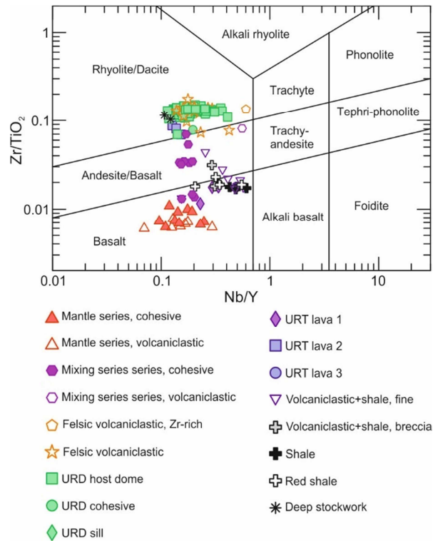
Figure 9: Zr/TiO 2 vs. Nb/Y diagram (Pearce, 1996, after Winchester and Floyd, 1977). Ratios calculated using concentrations in \mu\text{g g}^{-1} .
