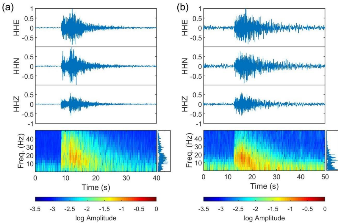
Figure 87: Comparison of a volcano-tectonic earthquake and a hybrid event. (a) Top: Traces of an earthquake occurring on occurring beneath Brava Fogo on 22 Feb 2017 18 Nov 2017 (16:44:19 UTC) recorded at the broad-band station AF02 of array AF on Fogo. Bottom left: spectrogram of the vertical component and overall, left: spectrogram of the vertical component, bottom right: corresponding frequency content (panel on the right). (b) Traces of a hybrid event recorded on 17 Aug 2017 (02:54 UTC) at the same station. Traces are filtered between 1 and 50 Hz to remove ocean-generated noise. Bottom left: spectrogram of the vertical component, bottom right: corresponding frequency content. Compared to the earthquake, the hybrid event shows no clear S-phase and more energy in the 1-10 Hz band (of the coda).
