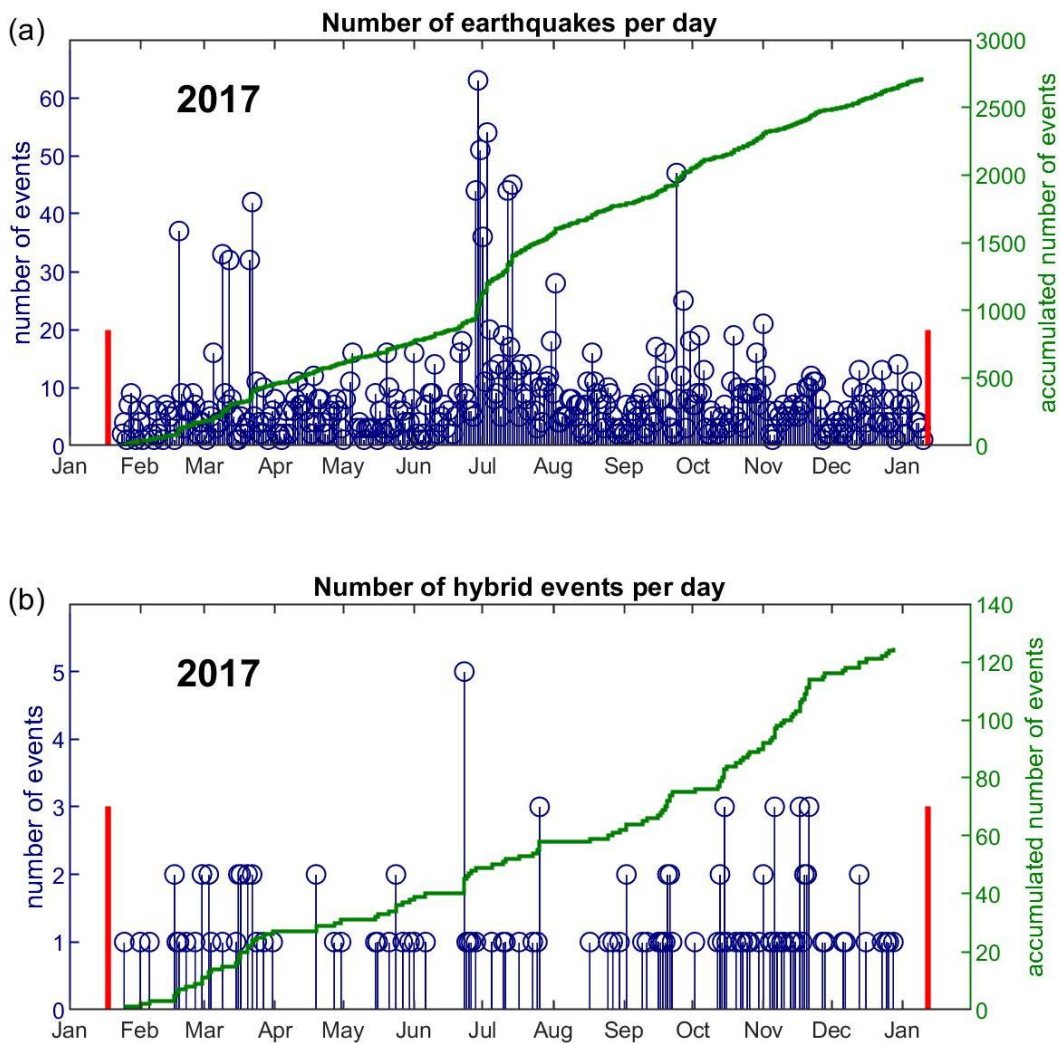
Figure 98: (a) Number of earthquakes per day. Green line: accumulated number of earthquakes. The Rrecordings range from 18 January 2017 to 12 January 2018. (b) Number of hybrid events per day. Green line: accumulated number of hybrid events during the same time period.
