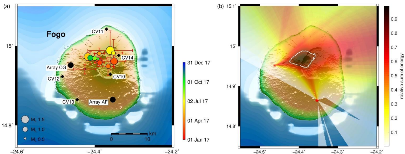
Figure 1011: (a) Locations of hybrid events detected between 18 Jan 2017 and 12 Jan 2018 and located with the arrays on Fogo. Black circles: array locations; black diamonds: short-period single stations. (b) Superimposed beams of all the hybrid localizations.
