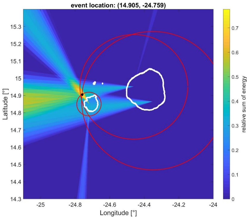
Figure 713: Verification of the result-event localization using additional travel-time information. b Black circle: location of the event derived from the intersecting beams; red circles: epicentral distances of the event estimated from S–P travel-time differences for observed at the three arrays. The circles give an rough estimate of the expected distance of the event to the array providing a tool to better judge the reliability of the outcome event location . Note, that this representation only serves as a support for the analyst. The final event location is only based on the multi-array analysis, and is not included in the estimation of the event location.
