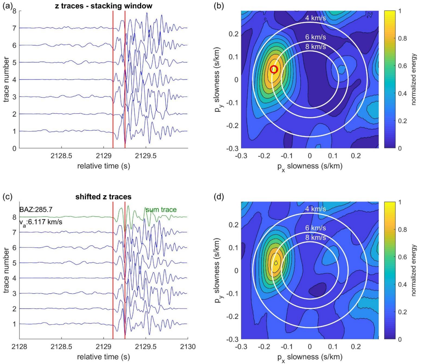
525 Figure 3: Time-domain array analysis of an earthquake on 22 July 2017 (23:35 UTC) at the array AF. (a) Analysis window of 2 s length with the stacking window marked in red. Traces are displayed before shifting and stacking and are filtered between 2 and 20 Hz. (b) Resulting time-domain energy stack. Red circle: maximum beam energy. (c) Time-shifted traces. The upper green trace represents the sum trace. (d) To retrieve the standard deviation of the backazimuth, the stacking window is varied 100 times by values between -0.2 and 0.2 s. The standard deviation is estimated from the 100 resulting backazimuth values. Shown here is the 530 stack of the 100 energy plots.
