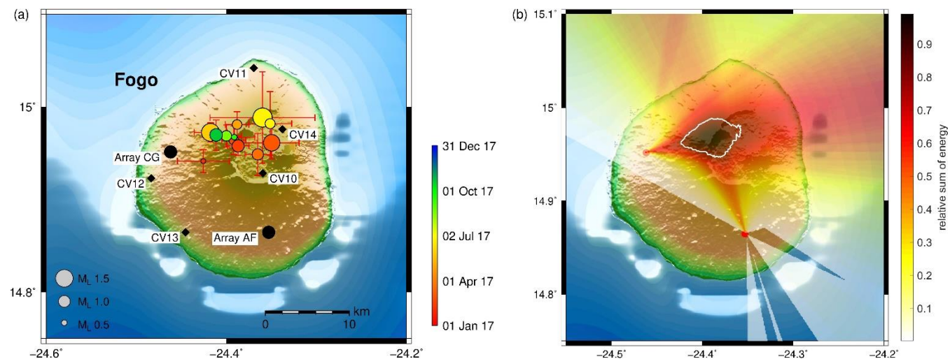
580 Figure 11: (a) Locations of hybrid events detected between 18 Jan 2017 and 12 Jan 2018 and located with the arrays on Fogo. Black circles: array locations; black diamonds: short-period single stations. (b) Superimposed beams of all the hybrid localizations. The
