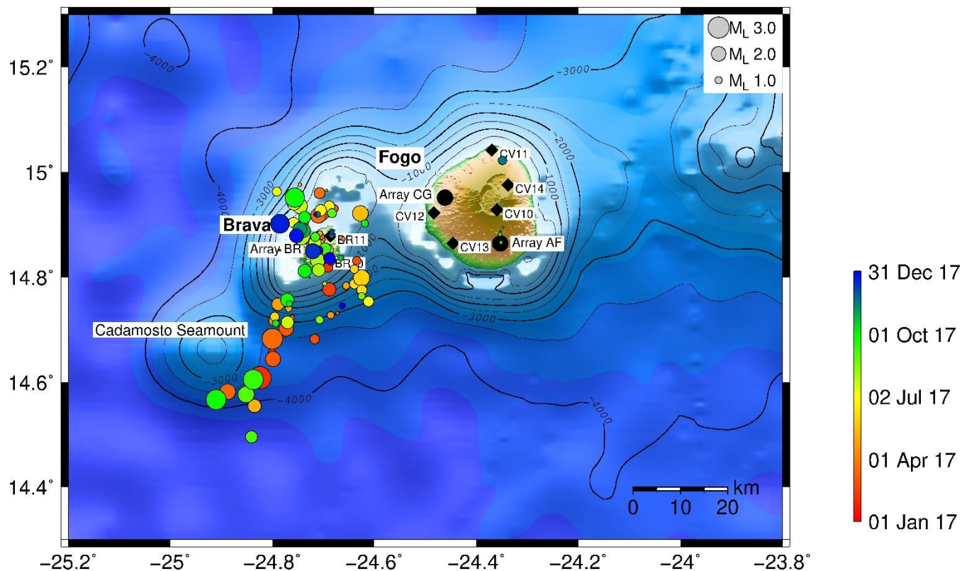
575 Figure 10: Earthquake locations from 18 Jan 2017 to 12 Jan 2018. Black circles: array locations; black diamonds: short-period single stations. Topography and bathymetry data are from Ryan et al. (2009).
