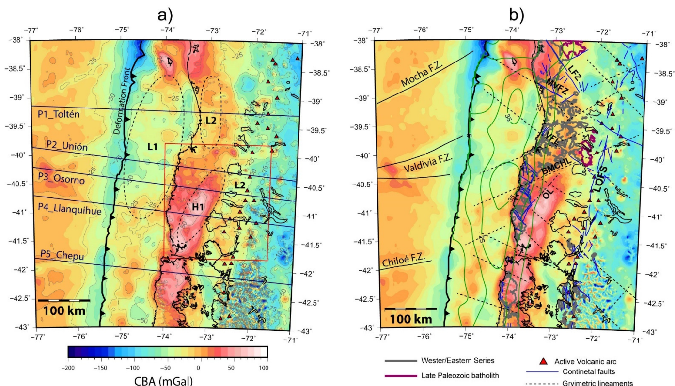
295 Figure 3: Complete Bouguer Anomaly (CBA) at the study zone. a) Main gravimetric forearc features observed in the area (see main text for details). The blue lines illustrate the tracks of 2D forward density models and the red rectangle indicates the zone where 3D density inversion was carried out. Dotted black ellipses shows the approximated extension of anomalies L1, L2 and H1 along with other elements seen in Fig. 1a. b) Crustal tectonic structures and CBA. The figure includes the contours of metamorphic Western/Eastern Series and Late Paleozoic batholith outcrops. Dotted black lines are interpreted gravimetric lineaments, e.g., Valdivia-Futroneo lineament (VFL), Bahía Mansa-Choshuenco lineament (BMCHL) and Osorno lineament (OL). The Other elements as in Fig. 1a.
