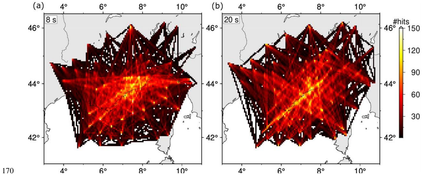
Figure 2: Hit count maps showing the ray coverage for ambient noise CCF-pairs at 8 s (a) and teleseismic CCF pairs at 20 s (b). The grid cells have a size of 5x5 km.
