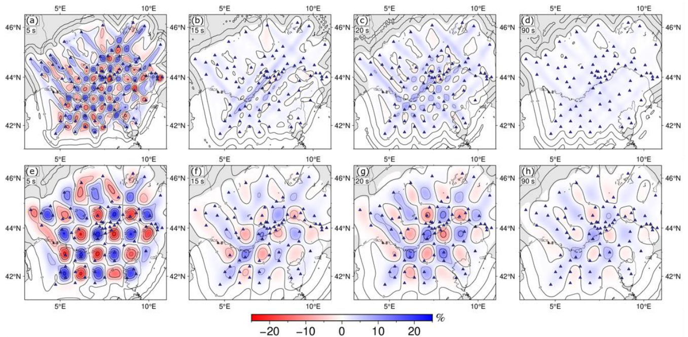
Figure 7: Checkerboard tests for periods of 5 s, 15 s (both ambient noise cross-correlation), 20 s, and 90 s (both teleseismic cross-correlation). The perturbation of the input checkerboard tiles is set to \pm 25\% . Panels (a)-(d) show checkerboard tests with a grid size of 0.4^\circ \times 0.4^\circ , panels (e)-(h) show a grid size of 0.8^\circ \times 0.8^\circ . The standard deviation of Gaussian noise (of travel times) is set to 0.375 s for (a) and (e), 0.665 s for (b) and (f), 0.708 s for (c) and (g), and 1 s for (d) and (h). Checkerboard tests for all other periods can be found in the Supplement (Fig. S3-S6). Blue triangles represent stations.
