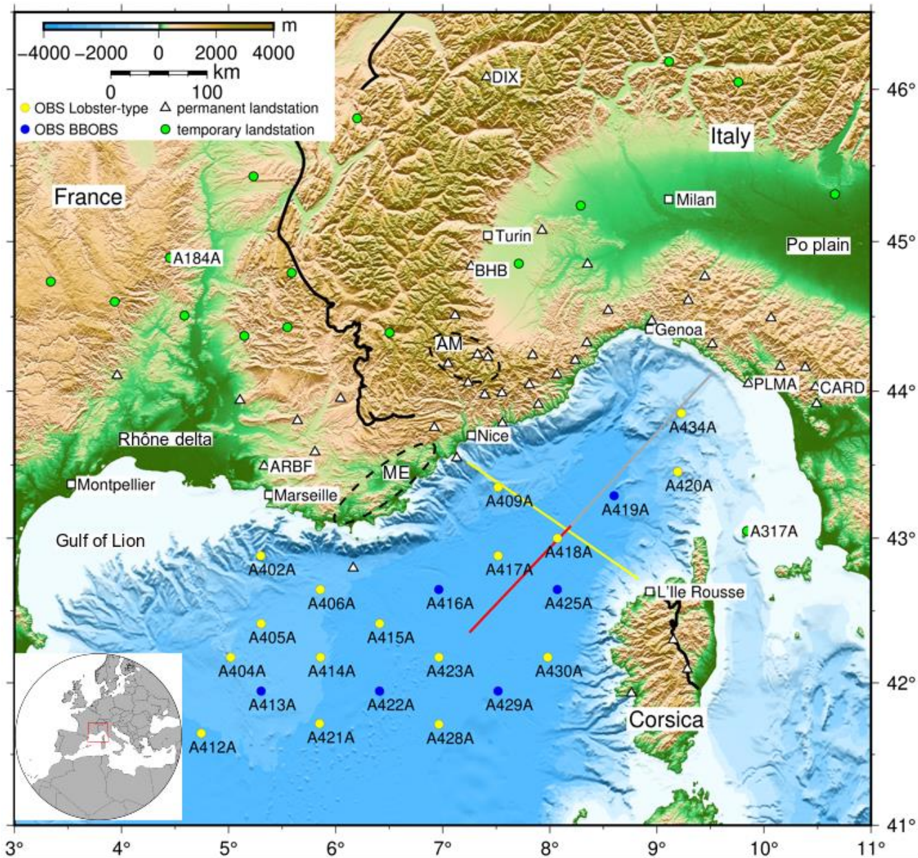
85 Figure 1: Map of the Ligurian Sea and adjacent Alpine region and the stations used for this study. OBS stations (network code: Z3) are shown as yellow (Lobster-type) and blue (BBOBS) circles. Permanent land stations (network codes: CH, FR, GU, IV, and MN, see Table S1) are shown as white triangles. Temporary land stations from AlpArray (network code: Z3) are shown as green circles. Station names are given for the OBS and land stations mentioned in the text or used in Fig. 3. White squares represent cities. The black line represents the Alpine front (Schmid et al., 2004), AM marks the Argentera Massif, and ME marks the Maures-Esterel 90 Massif. The inlay map in the bottom left shows the location of the research area (red box). The red, grey, and yellow lines show
