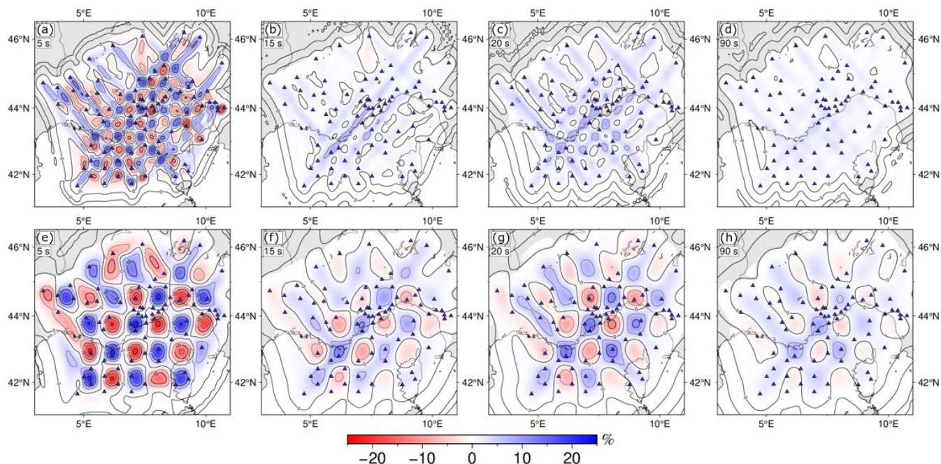
340 Figure 7: Checkerboard tests for periods of 5 s, 15 s (both ambient noise cross-correlation), 20 s, and 90 s (both teleseismic cross-correlation). The perturbation of the input checkerboard tiles is set to \pm 25 %. Panels (a)-(d) show checkerboard tests with a grid size of 0.4^\circ \times 0.4^\circ , panels (e)-(h) show a grid size of 0.8^\circ \times 0.8^\circ . The standard deviation of Gaussian noise (of travel times) is set to 0.375 s for (a) and (e), 0.665 s for (b) and (f), 0.708 s for (c) and (g), and 1 s for (d) and (h). Checkerboard tests for all other periods can be found in the Supplement (Fig. S3-S6). Blue triangles represent stations.
