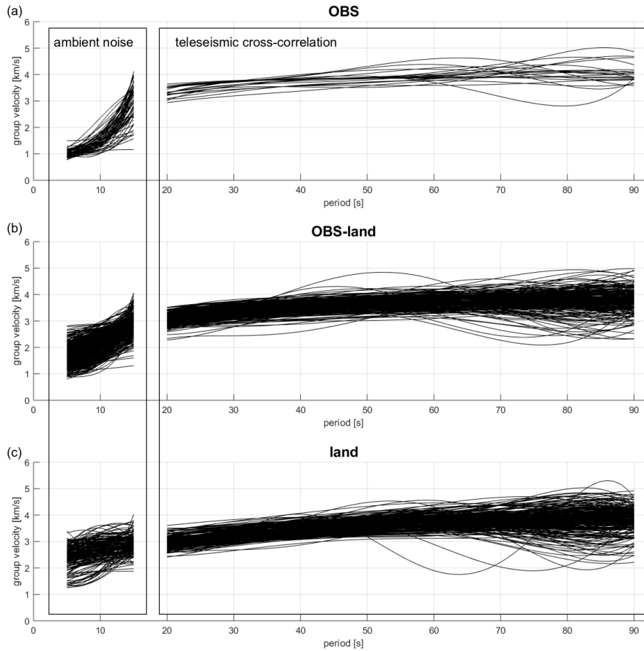
220 Figure 5: Picked dispersion curves from ambient noise cross-correlation and correlation of teleseismic events. The dispersion curves are sorted for different types of station pairs: (a) OBS-OBS pairs, (b) OBS-land pairs and vice versa, (c) land-land pairs.
