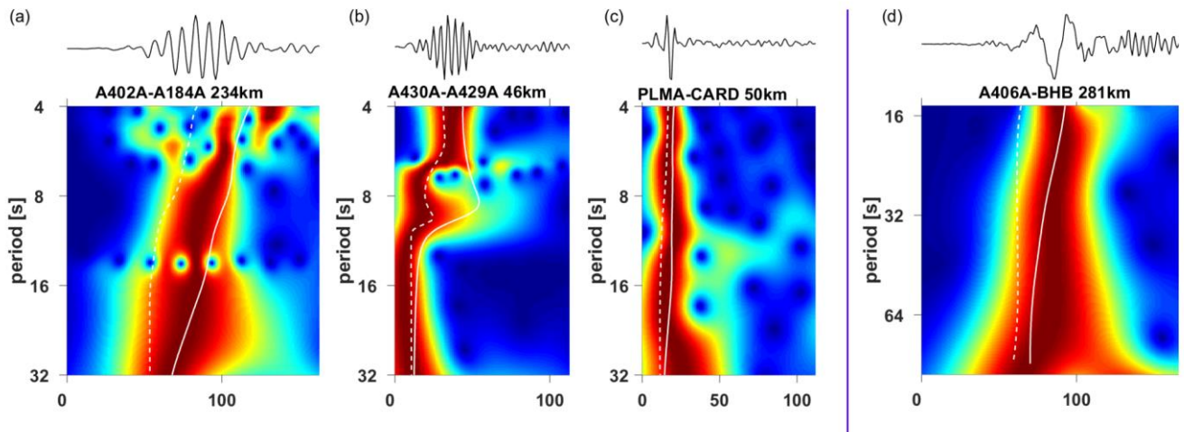
190 Figure 3: MFT examples for correlations on (a) OBS-land pair, (b) OBS-OBS pair, (c) land-land pair (all ambient noise cross-correlations), and (d) land-land station pair (cross-correlation containing teleseismic event). The solid white line shows the theoretical fundamental mode; the dashed white line shows the theoretical first higher mode. In (a), (c), and (d), the theoretical fundamental mode fits the theoretical velocities. In (b), the theoretical first higher mode correlates most strongly. Therefore, pair (b) was excluded from the tomography.
