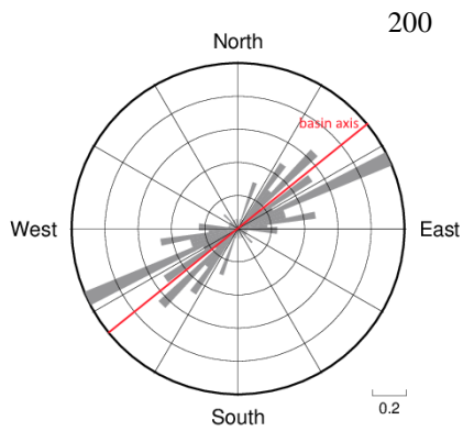
Figure 4: Rose diagram of ray path azimuths showing the striking directions of the higher modes. The red line indicates the basin axis.
