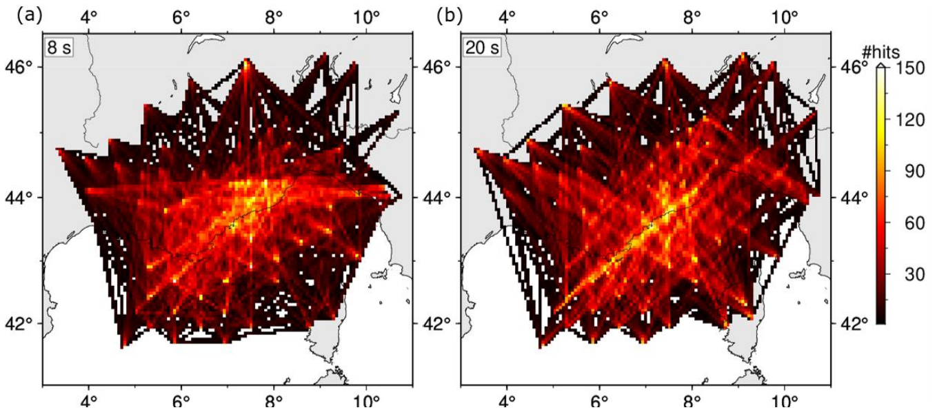
170 Figure 2: Hit count maps showing the ray coverage for ambient noise CCF-pairs at 8 s (a) and teleseismic CCF pairs at 20 s (b). The grid cells have a size of 5x5 km.
