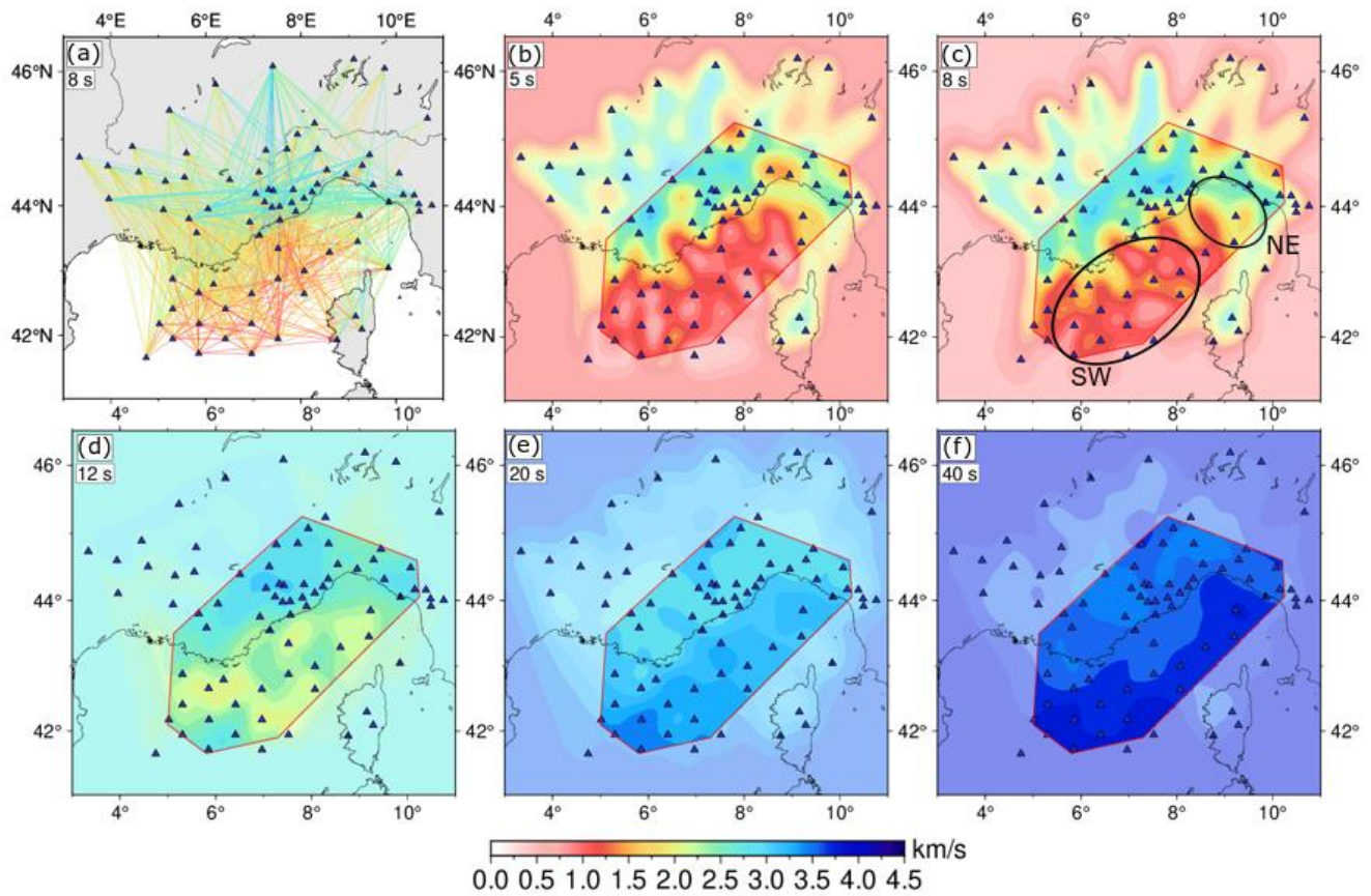
Figure 6: Panel (a) shows the tomography input for 8 s as a ray path plot. Panels (b)-(f) show group velocity maps of the Ligurian Basin from surface wave tomography for 5 s, 8 s, 12 s, 20 s, and 40 s period, whereby (b), (c), and (d) are based on ambient noise cross-correlation and (e) and (f) are based on the cross-correlation of teleseismic events. A red polygon marks the resolved area. Areas of low resolution are shown in transparent colours; areas without ray coverage show the initial velocity. Annotations in (c) mark the southwestern and central (SW) and the northeastern (NE) Ligurian Basin. Blue triangles represent stations.
