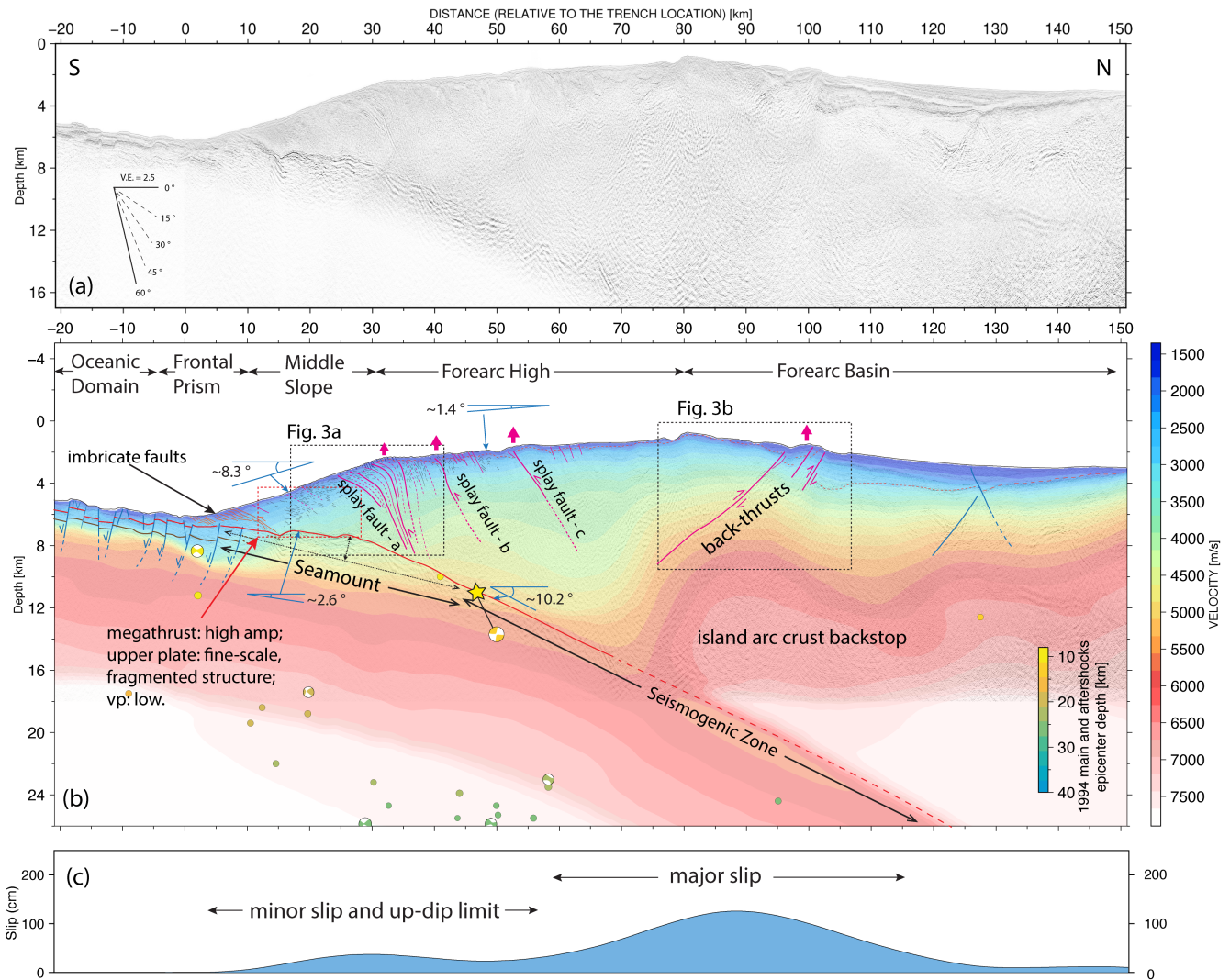
Figure 2. (a) Pre-stack depth migrated section of seismic profile SO190 BGR06_305. (b) Seismic section overlain by the vp model (based on MCS reflection tomography above 3 km depth, velocities below from Shulgin et al. (2011), see Fig. S5), our structural interpretation, and the aftershock seismicity (from catalogue ISC-EHB Bulletin; Engdahl et al., 2020) of the 1994 Java tsunami earthquake. The hypocentre is marked as a yellow star. Coloured circles and beach-balls are aftershocks (Timespan: 03 June, 1994 to 14 Oct, 1994) from the ISC-EHB Bulletin catalogue (Engdahl et al., 2020). Focal mechanisms from the gCMT catalogue (Dziewonski et al., 1981; Ekström et al., 2012). The well-developed forearc high (75 – 100 km) results from back-thrusting above the island arc crust backstop. A subducting seamount between kilometres 5 – 45 is overlain by upper plate splay faults. (c) Co-seismic slip model of the 1994 earthquake along the profile (Bilek & Engdahl 2007). Peak slip occurred underneath the backstop (55 – 105 km) and decreased towards the subducting seamount (5 – 45 km).
