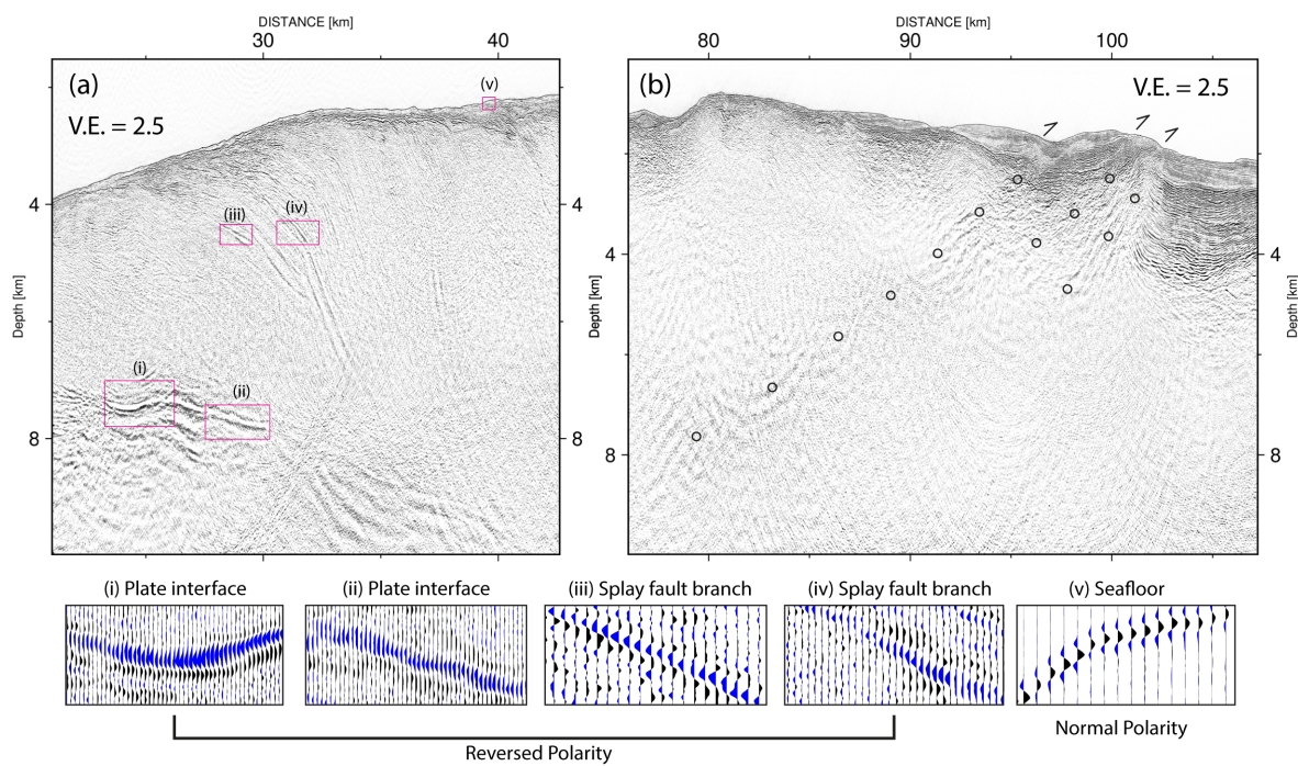
170 Figure 3. (a) Seismic section with a close-up view of the splay fault - a (compare Fig. 2b for location) branching from the landward side of the subducting seamount. Red boxes indicate close-up views shown in the lower panels. Reversed polarity reflections (relative to the seafloor) are observed at the plate interface seaward of the seamount and along the splay fault. The black and blue colours present positive and negative wavelet polarity, respectively. (b) Seismic section with a close-up view of the back-thrust (compare Fig. 2b for location). Black circles mark the back-thrust fault planes.
