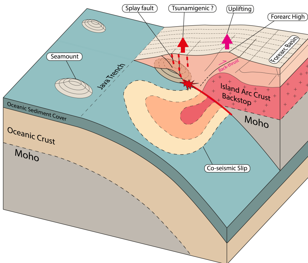
Figure 4. Conceptual seismo-tectonic model of the eastern Java margin in the region of the 1994 tsunami earthquake. Back-thrusting above the island arc crust backstop causes locally enhanced uplift of the forearc high. The 1994 hypocentre (red star) originated at the leading edge of a subducting seamount. The seamount stalled the co-seismic slip propagation locally along the plate boundary.
