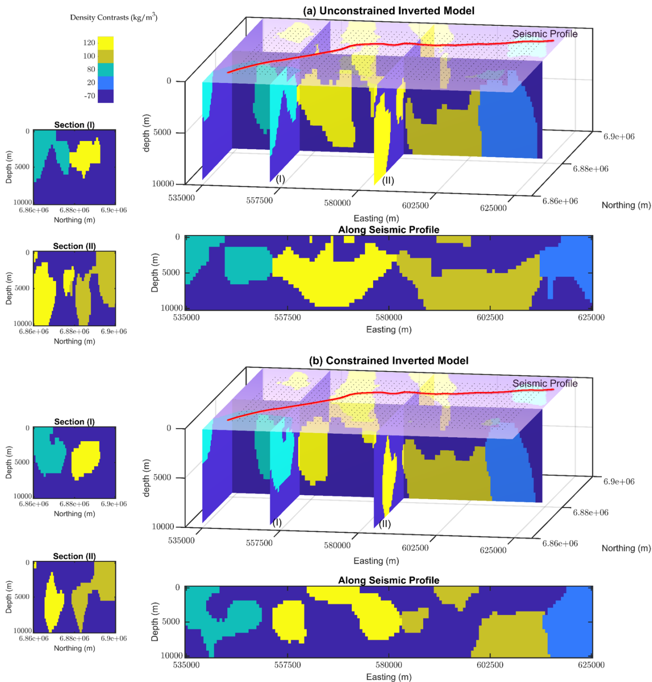
440 Figure 12: Different views of the final inverted models from the unconstrained and constrained 3d gravity level-set inversion of Yamarna Terrane respectively. Black dot points at the surface level represent the interpolated gravity data.
