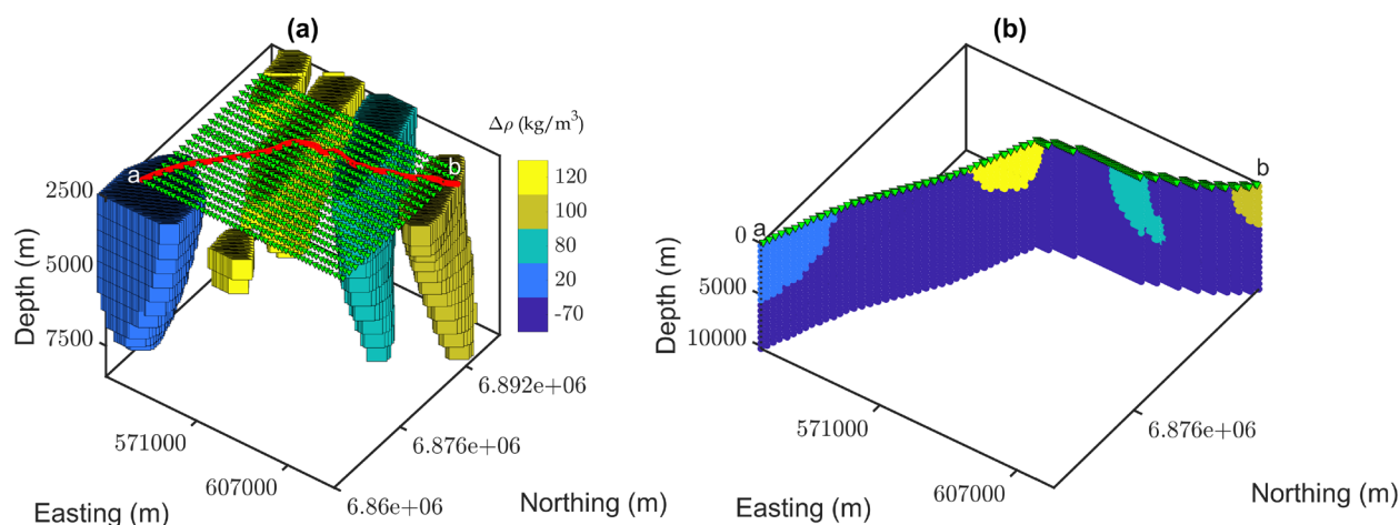
Figure 10: Density contrasts of the adjusted starting model and the interpolated gravity grid configuration (a) model cell centres of the extracted 2D model along the seismic profile (b).
