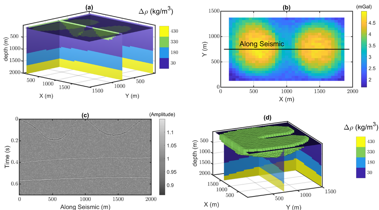
290 Figure 4: 3D view of the true model (a) and surface gravity anomaly response (b), zero-offset synthetic seismic section (c), 3D view of the starting model (d).
