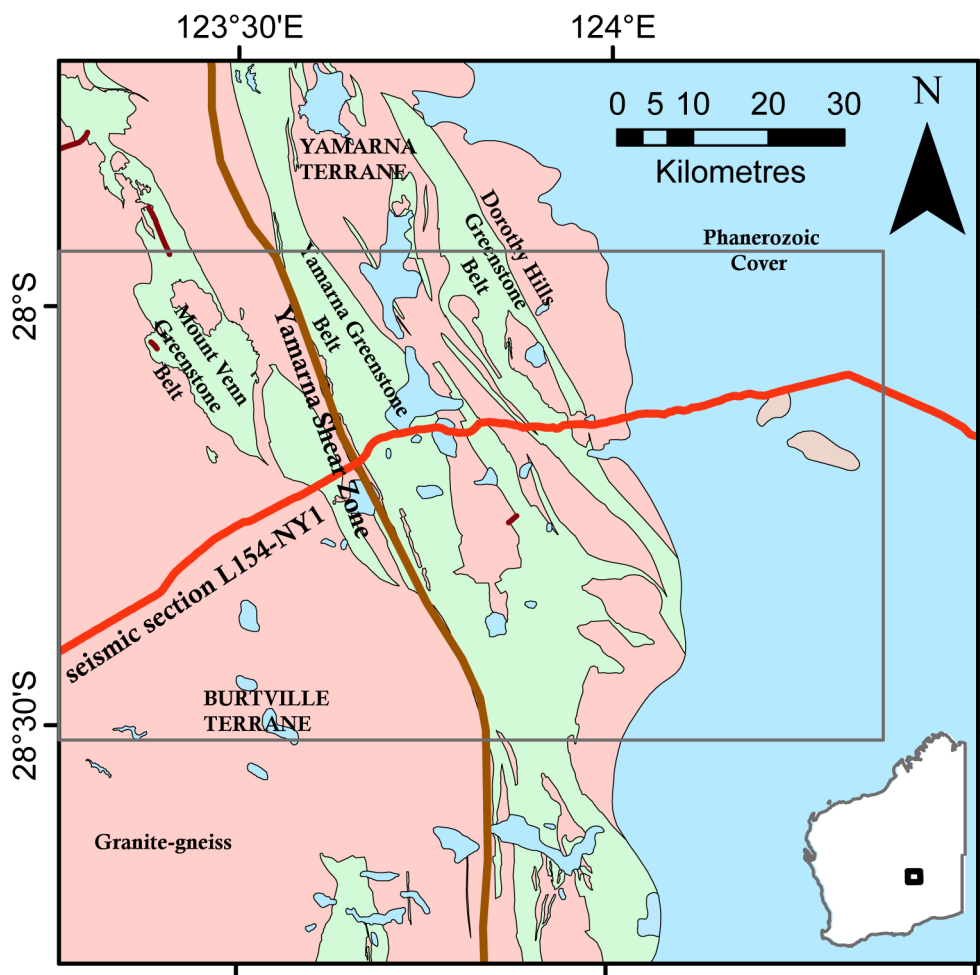
315 Figure 7: Geographical coordinates and geological units of the region of interest in the Yamarna Terrane, Eastern Yilgarn Craton, Albany-Fraser Orogen (Modified from Lindsay et al., 2020). The grey rectangular show the boundary of the region of interest in this study.
