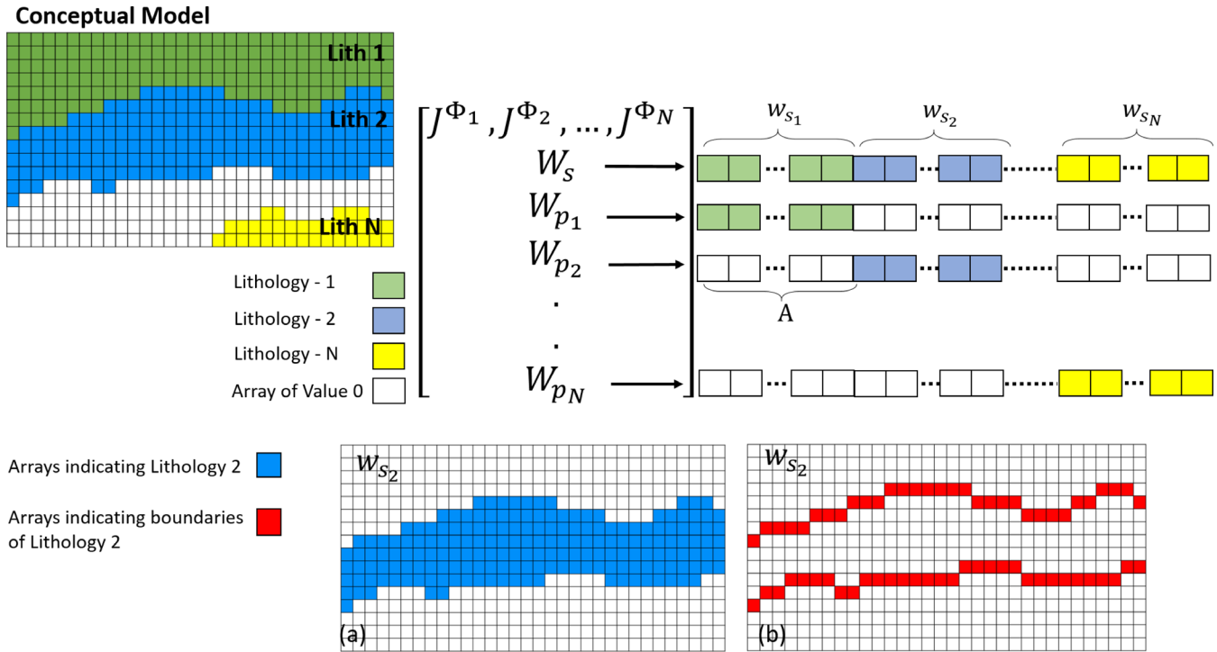
165 Figure 1: Illustration of the process of appending constraints to the level-set problem from a sample 2D geological model. Distribution of constraint matrix of from lithology 2 for the entire unit (a) and for the corresponding boundaries (b). W_{s_2} is shown only for the corresponding 2D section.
